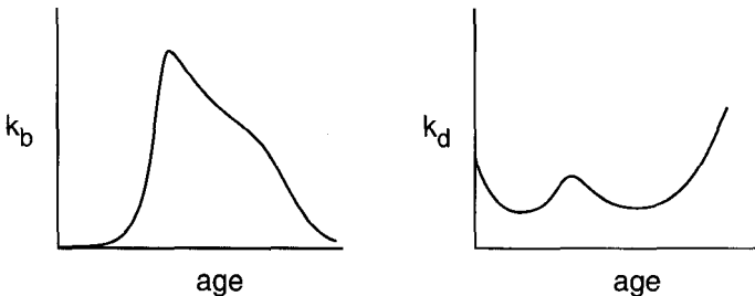
Figure 8-22 Effective “rate constants” of reproduction k_b and death k_d of living organisms.
