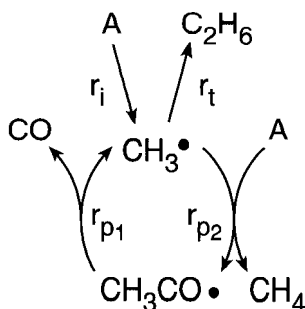
Figure 10-1 Sketch of the chain reaction for acetaldehyde decomposition. The chain cycles between \text{CH}_3\cdot and \text{CH}_3\text{CO}\cdot radicals in the propagation steps and is fed by acetaldehyde and terminated by methyl recombination.
