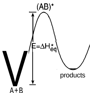
Figure 4-14 Energy diagram illustrating the reactants A and B and the activated complex (AB)^* in the activated complex theory of bimolecular reactions.
