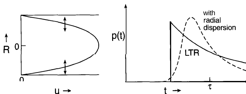
Figure 8-7 Effect of radial mixing on flow profile and p(t) .
