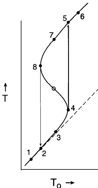
Figure 6-S Plot of reactor temperature T versus feed temperature T_0 in an adiabatic CSTR. The arrows indicate discontinuous jumps in reactor temperature T . The points marked are from Figure 6-7 with points 4 and 8 tangents of the heat generation and removal curves.
