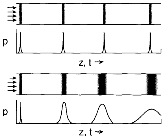
Figure 8-8 Dispersion broadening of p(t) in a tubular reactor.
