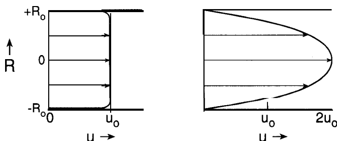
Figure S-4 Velocity profiles in a tube in plug-flow and in laminar flow reactors.
