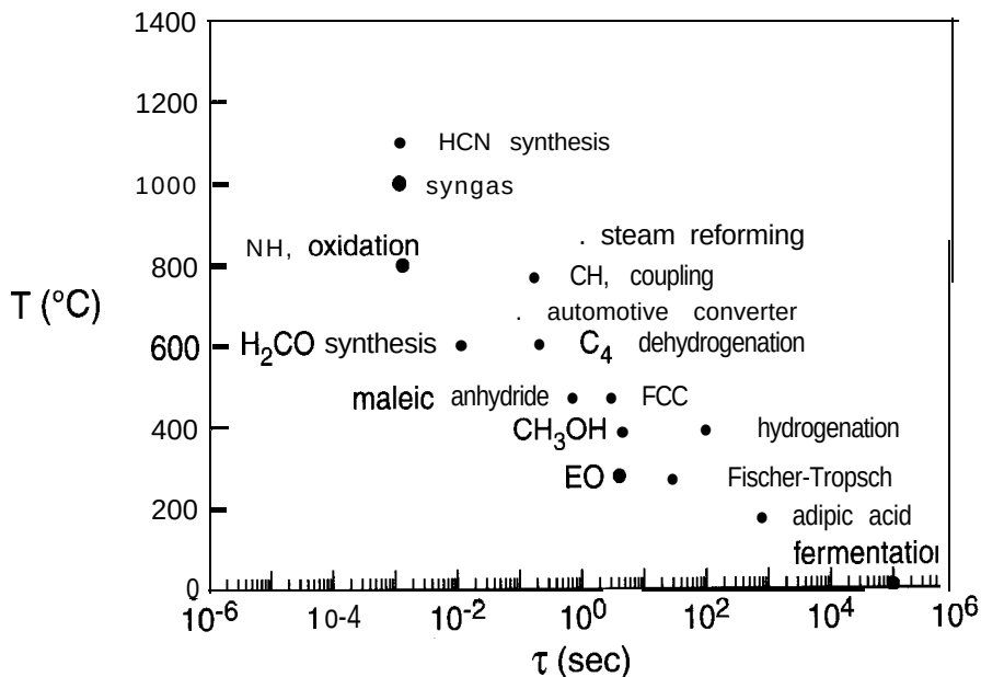
Figure 3-7 Plot of nominal space times (or reactor residence times) required for several important industrial reactors versus the nominal reactor temperatures. Times go from days (for fermentation) down to milliseconds (for ammonia oxidation to form nitric acid). The low-temperature, long-time processes involve liquids, while the high-temperature, short-time processes involve gases, usually at high pressures.
