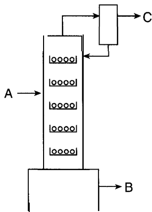
Figure 12-18 Catalytic distillation reactor in which catalyst in the distillation column combines chemical reaction with vapor-liquid equilibrium in the column to achieve conversions higher than obtainable with a reactor alone.
