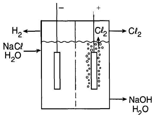
Figure 7-29 Salt electrolysis to produce \text{Cl}_2 gas and \text{NaOH} solution in a chloralkali process. This is the process by which most alkali and chlorine are produced. The reactor operates continuously with brine solution flowing into the cell and \text{NaOH} and \text{Cl}_2 gas flowing out.
