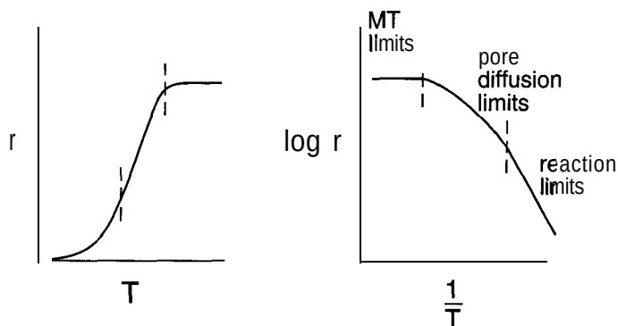
Figure 7-15 Plots of r versus T and \log r versus 1/T . We expect the rate to exhibit breaks on the 1/T plot as the reaction process goes from reaction limited at low temperature, pore diffusion limited at intermediate temperature, and external mass transfer limited at high temperature.
