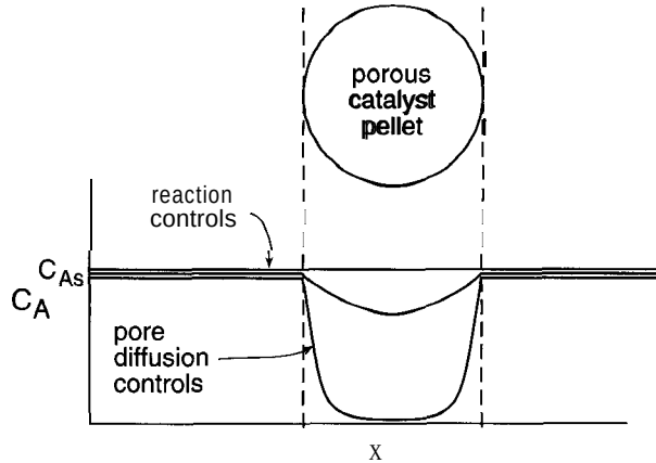
Figure 7-11 Reactant concentration profiles within a porous catalyst pellet for situations where surface reaction controls and where pore diffusion controls the reactions.
