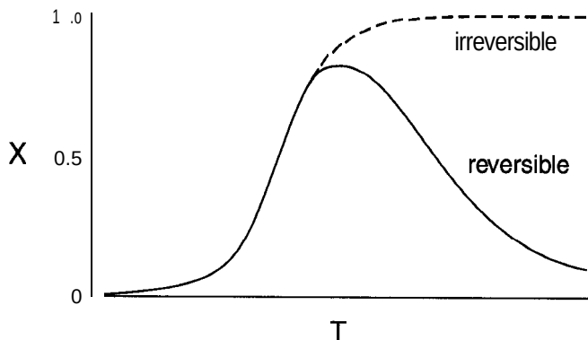
Figure 6-13 Plots of X(T) for the exothermic irreversible (dashed curve) and reversible (solid curve) reactions. If the reaction is reversible, the conversion falls at high temperature, but multiple steady states are still possible.
