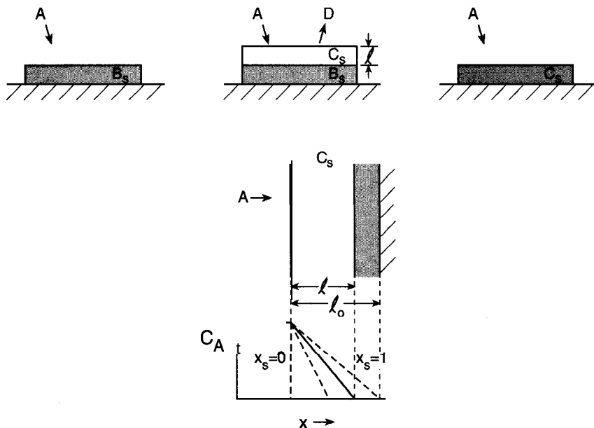
Figure 9-13 Reactant concentration profiles C_A(x) within a product film C_s for a film transforming from B_s to C_s . The profile of the diffusion-limited migration of A through the film remains a straight line; so the growth rate (proportional to the gradient) decreases as the film thickens, leading to the parabolic law of film growth.
