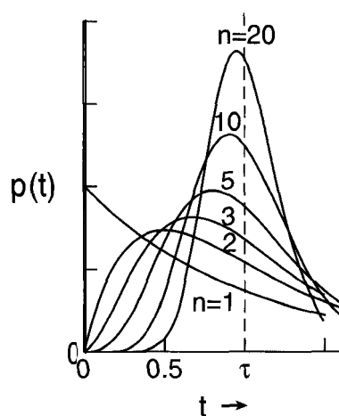
Figure g-12 Residence time distribution of n CSTRs of equal residence times in series. The distribution sharpens as n increases and eventually approaches the perfect PFTR.
