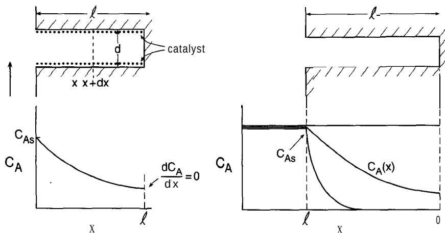
Figure 7-12 Reactant concentration profiles down a single catalyst pore of length \ell and diameter d_p with a catalytic reaction occurring on the walls of the pore. The concentration is C_{As} at the pore mouth, x = \ell , and the gradient is zero at the end of the pore because the end is assumed to be unreactive and there is therefore no flux of reactant through the end.
