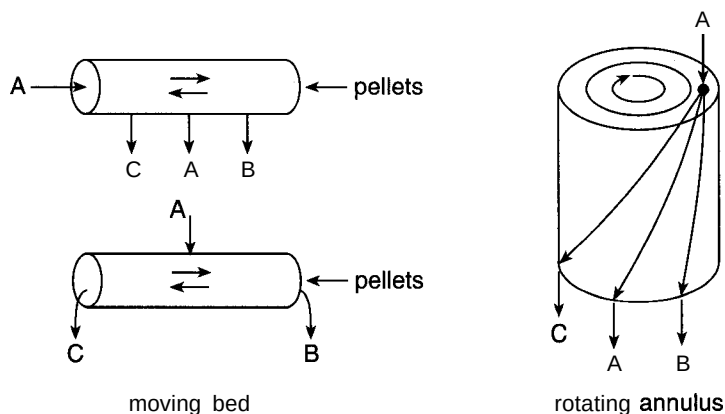
Figure 12-21 Countercurrent moving bed and rotating annulus reactors. Chromatographic separation of species in a continuous chemical reactor can be accomplished with a moving bed tubular reactor or a rotating annulus reactor that separates A , B , and C by carrying a product species counter to the flow direction because it is adsorbed on the moving catalyst.
