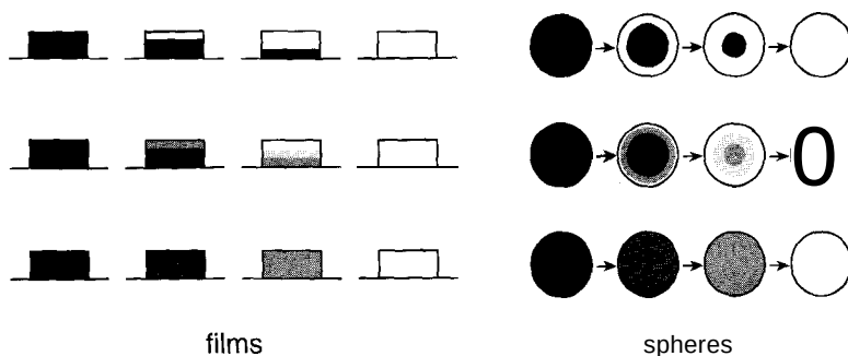
Figure 9-6 Sketches of transforming films or particles, where solid B_s (black) is transformed into C_s (colorless). Sketches shown involve a sharp boundary between reacted and unreacted layers, with reaction assumed to occur only at the interface between the core B and the film C .
