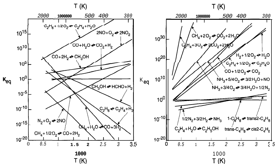
Figure 2-11 Plots of equilibrium constant K_T versus temperature for several chemical reactions we will consider in this text. All these reactions give nearly straight lines when plotted as \log K_T versus 1/T . Exothermic reactions have large K_T at low T , while endothermic reactions have large K_T at high T .
