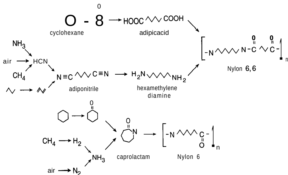
Figure 11-S Flowsheets of reactions to prepare Nylon 66 and Nylon 6 from petroleum feedstocks
