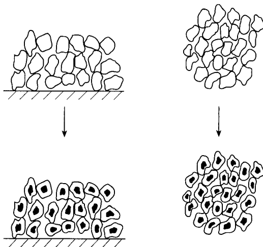
Figure 9-8 Microstructures of solid films and pellets. Variations can occur across a film or sphere as well as within individual particles in the film or sphere.
