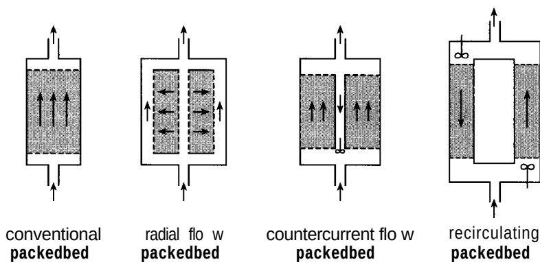
Figure 7-27 Fluid flow patterns in fixed bed reactors, which allow the variation of velocity profiles within the catalyst bed.
