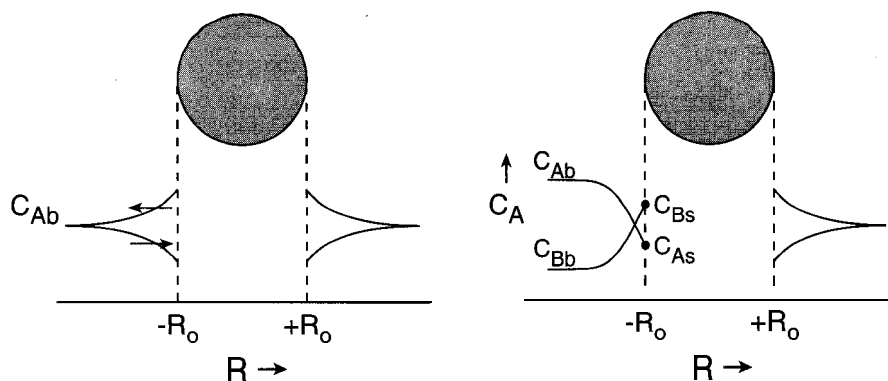
Figure 12-11 Sketches of concentration profiles of a reactant A around a drop where the reaction is in the surrounding continuous phase. Arrows indicate directions of reactant mass flow.
