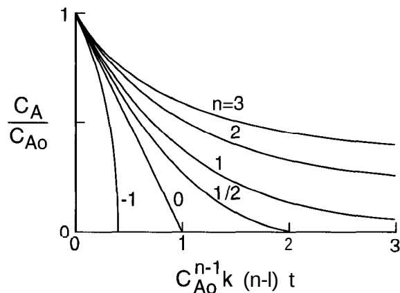
Figure 2-6 Plot of reactant concentration C_A versus dimensionless time (n-1)k C_{A0}^{n-1} t for the n th-order irreversible reactions A \rightarrow products, r = k C_A^n . The expression is indeterminate for n=1 .
