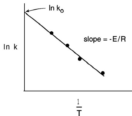
Figure 2-20 Plot of \ln k (obtained from isothermal reaction data in the previous figure) versus 1/T . The slope of this line is -E/R , and the intercept where 1/T = 0 is the pre-exponential factor k_0 .
