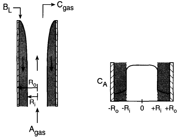
Figure 12-8 Sketch of a falling film reactor with positions R_o and R_i indicated. At the right are sketched possible concentration profiles of a reactant A , which is supplied in the gas but reacts in the liquid.
