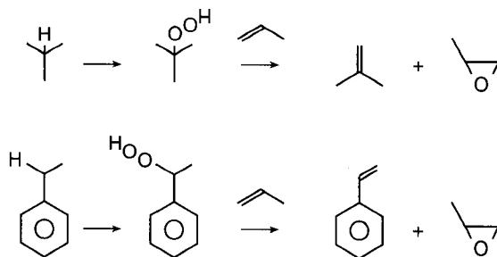
Figure 10-4 Reaction steps to make propylene oxide and either isobutylene or styrene by autooxidation.
