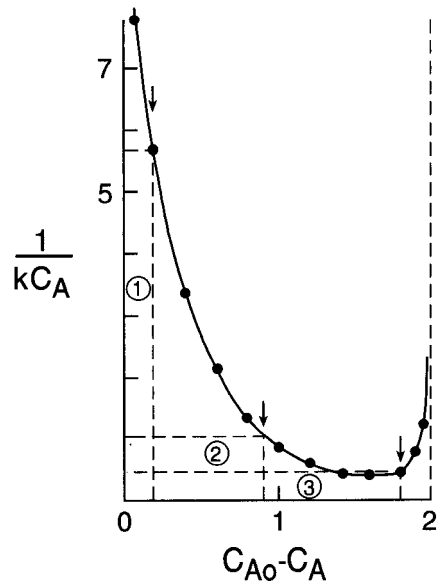
Figure 5-9 Plot of 1/r versus C_{A0} - C_A for the previous example. It is seen that 1/r increases and then decreases so that 1/r has a strong minimum. The arrows indicate the three possible steady states in a CSTR for \tau = 1.0 min (dashed rectangles).
