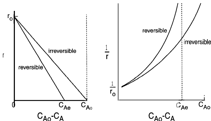
Figure 3-14 The r and 1/r plots for a reversible reaction where r goes to zero and therefore 1/r goes to infinity at the equilibrium conversion.
