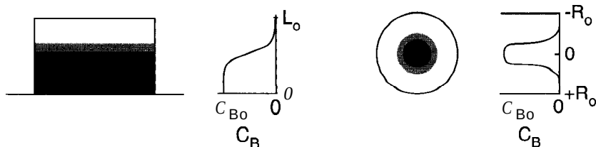
Figure 9-7 Sketch of possible concentration profiles (indicated by shading) as solids react
