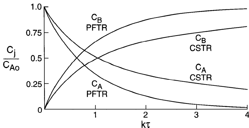
Figure 3-3 Plots of C_A(\tau) and C_B(\tau) in PFTR and CSTR for a first-order irreversible reaction A \rightarrow B, r = kC_A . By plotting versus kt , the graphs appear identical for any value of k .
