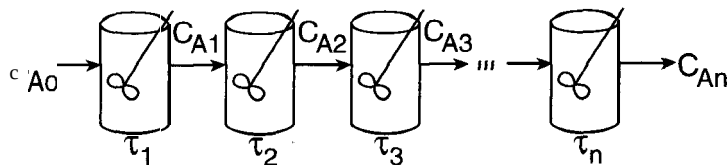
Figure 3-8 Sketch of ideal chemical reactors in series with C_{An} , the product from reactor n , which is also the feed into reactor n+1 .
