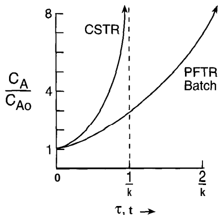
Figure 8-20 Plot of C_A(\tau) for the reaction A \rightarrow 2C , r = k_b C_A in a PFTR and in a CSTR. Reaction is always faster in a CSTR, and the concentration is predicted to go to infinity when k_b\tau = 1 .
