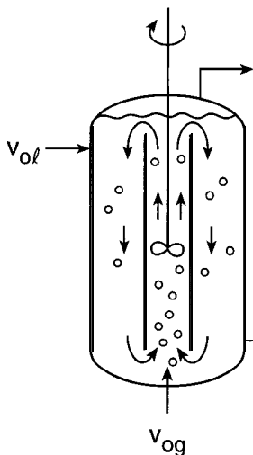
Figure 12-16 Sketch of sparger reactor in which an impeller continuously redisperses the bubble phase to maintain small bubble sizes and increase mass transfer. The impeller also recirculates the fluids in the reactor by placing it in a draft tube, which forces the fluids past the impeller at high velocities and further enhances mass transfer.
