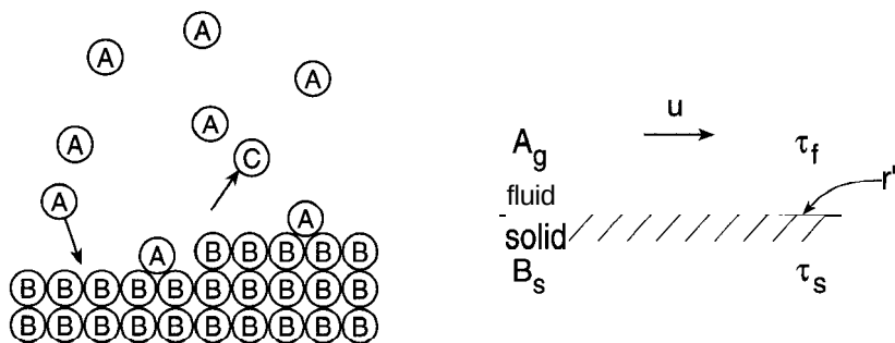
Figure 9-3 Sketch of molecules of A , reacting with solid atoms or molecules B_s to form gaseous and solid products in the reaction A + B_s \rightarrow C + B_s . Reaction occurs by species A first adsorbing on the surface of B ; so the process is a surface reaction. At the right are shown the quantities of interest in this process.
