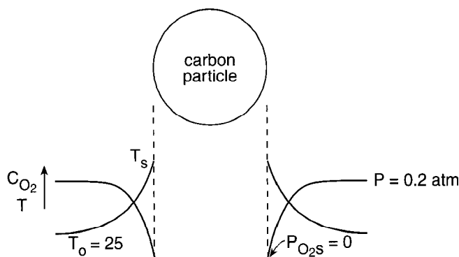
Figure 10-15 Concentration and temperature profiles around a burning carbon particle in air ( P_{O_2} = 0.2 atm and T_0 = 25^\circ\text{C} ). The concentration of O_2 falls to zero at the surface and the temperature rises to nearly the adiabatic flame temperature.
