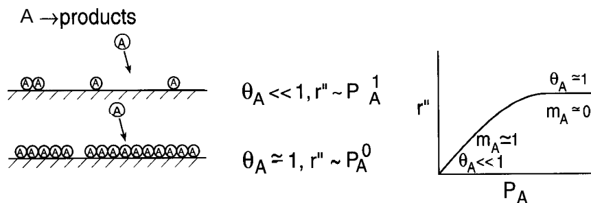
Figure 7-25 Langmuir-Hinshelwood kinetics for a unimolecular surface-catalyzed reaction A \rightarrow \text{products} . The rate is first order in P_A at low coverages and zeroth order at high coverage.
