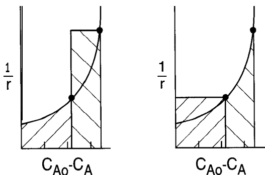
Figure 3-11 Residence times from 1/r plots for PFTR and CSTR in series.
