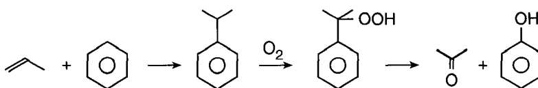
Figure 10-5 Reaction steps to make acetone and phenol by autooxidation of isopropyl benzene (also called cumene).
