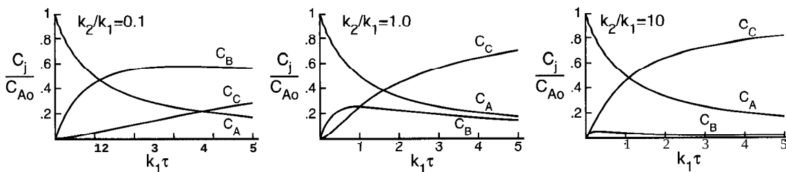
Figure 4-S C_A , C_B , and C_C versus k_1 \tau for series reactions A \rightarrow B \rightarrow C in a CSTR. Plots shown are for k_2/k_1 = 0.1 , 1.0, and 10. The yield to form B exhibits a maximum at a particular residence time \tau_{\max} , but this maximum is lower than in a PFTR.
