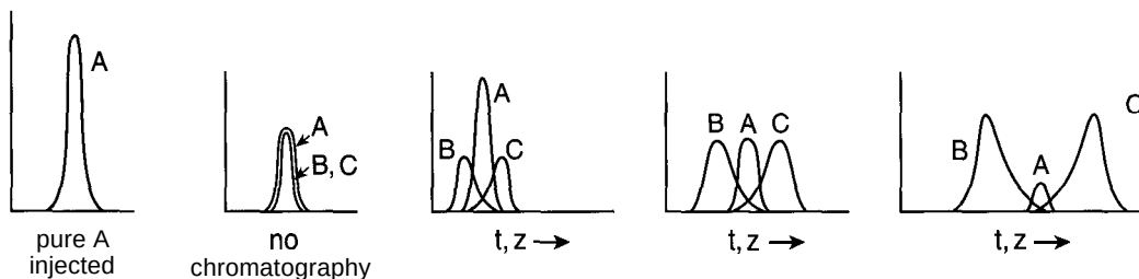
Figure 12-20 Chromatogram of species A , B , and C injection of pure A with the reaction A \rightarrow B + C . Separation of B from C reduces the rate of the back reaction and produces complete conversion even though equilibrium is not favorable.
