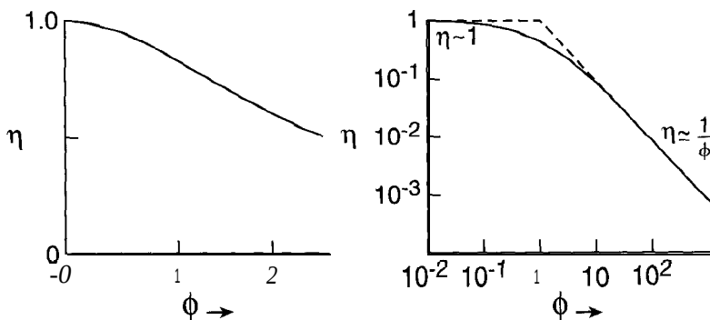
Figure 7-13 Plots of effectiveness factor \eta versus Thiele modulus \phi for diffusion in a single catalyst pore or in a porous catalyst pellet. On a log-log plot the effectiveness factor is seen to give \eta = 1 if \phi \ll 1 and \eta = 1/\phi if \phi \gg 1 .
