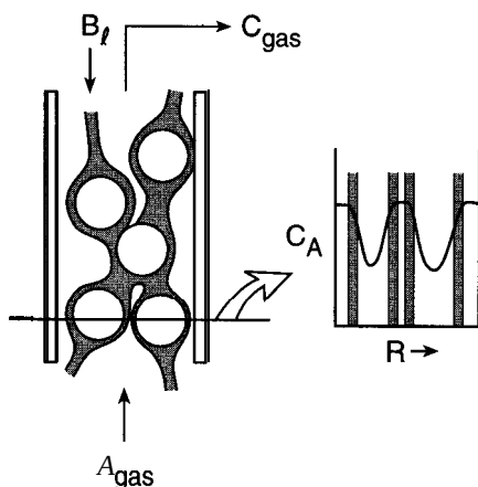
Figure 12-14 Sketch of trickle bed reactor in which liquid from the top of the reactor and gas rising from the bottom of the reactor contact stationary catalyst particles to produce a catalytic reaction. At the right is a sketched concentration profile for the cross section shown.
