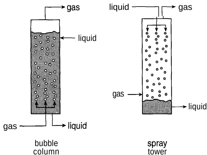
Figure 12-9 Bubble column and spray tower reactors. Large drop or bubble areas increase reactant mass transfer,
