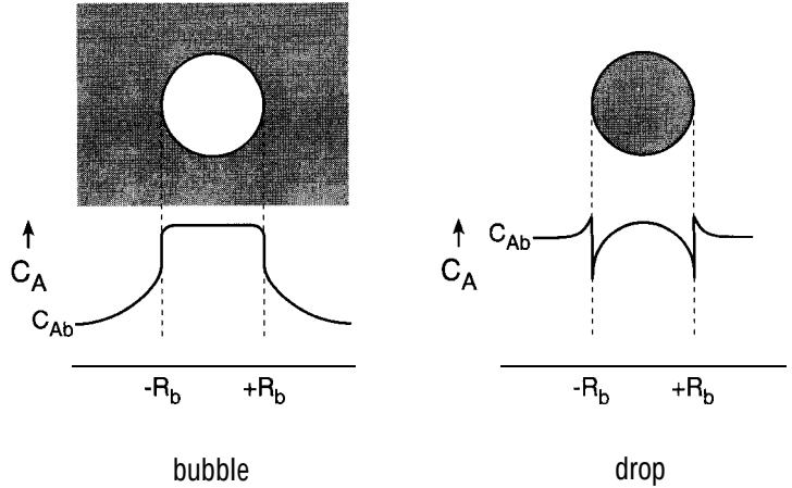
Figure 12-10 Sketches of reactant concentration C_A around a spherical bubble or drop that reacts after migrating from the gas phase into the liquid phase in bubble column and spray tower reactors.
