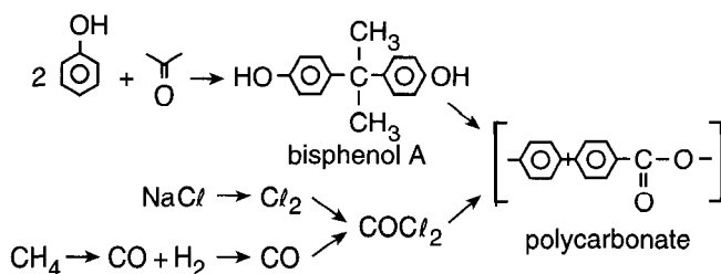
Figure 11-11 Flowsheet of a process to produce polycarbonate polymer.
