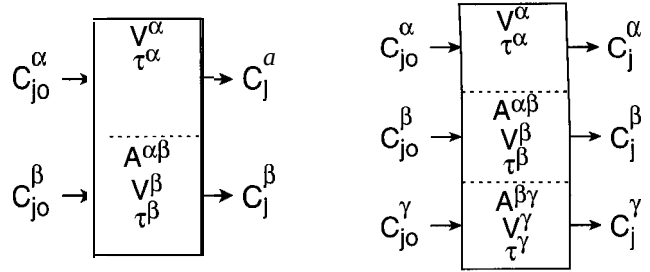
Figure 12-1 Sketch of two- and three-phase reactors. Variables must be specified in each phase \alpha , \beta , and \gamma .
