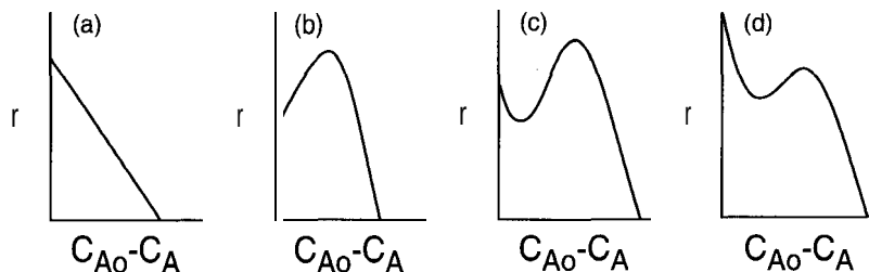
Figure 3-22 Same possible r versus conversion plots.
