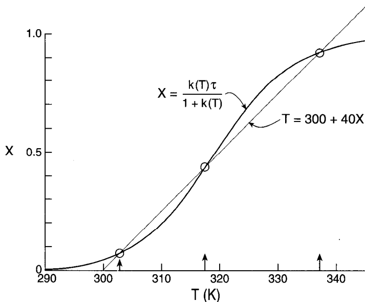
Figure 6-9 Plot of X(T) for the previous example for conditions that produce three steady states for \tau = 1 min..
