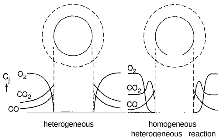
Figure 10-14 Concentration profiles around a burning carbon particle, either with or without homogeneous reaction in the boundary layer around the particle.
