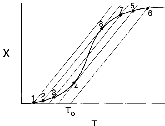
Figure 6-7 Heat removal curves in which T_0 is increased or decreased. One or three intersections with X(T) indicates that one or three steady states occur.
