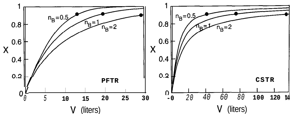
Figure 3-6 Plot of conversion versus reactor volume V for the reaction A \rightarrow n_B B , r = kC_B , with ideal gases for n_B = 2, 1 , and \frac{1}{2} . The times are all close until the conversion becomes large, when the product dilutes the reactant for n_B = 2 and slows the reaction.
