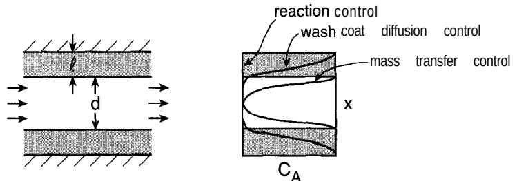
Figure 7-20 Sketch of tube wall reactor with a porous catalyst film of thickness \ell on walls. Expected reactant concentration profiles with reaction-limited, mass-transfer-limited, and pore-diffusion-limited reaction.
