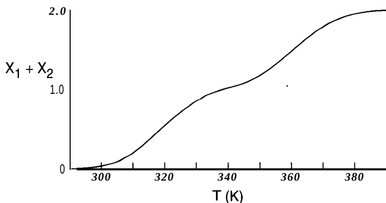
Figure 6-14 Plot of possible conversions ( X_1 + X_2 ) versus reactor temperature T in an adiabatic CSTR with series exothermic reactions A \rightarrow B \rightarrow C . Up to five steady state intersections are possible for this situation.
