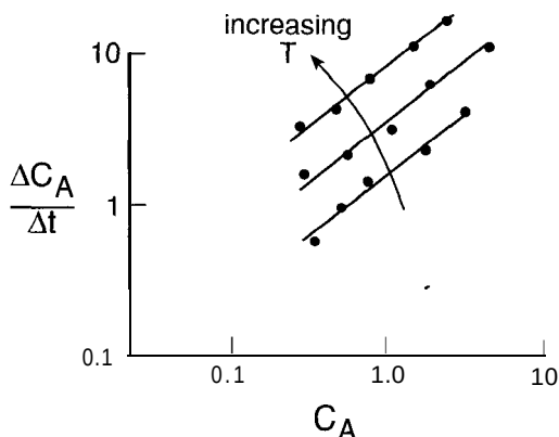
Figure 2-21 Differential reactor data analysis. Plots of \Delta C_A / \Delta t versus C_A on a log-log scale should give straight lines for fixed T . The slope of this line is the order m_A , while the value of the vertical scale where C_A = 1 is the rate coefficient k .
