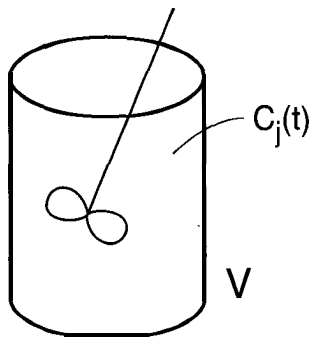
Figure 2-4. Sketch of a uniform closed container for running chemical reactions, which we call a batch reactor.
