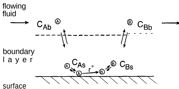
Figure 7-8 Elementary steps that must occur in a catalytic reaction on a surface. All catalytic processes involve transport through a boundary layer, adsorption, surface diffusion, reaction, and desorption.
