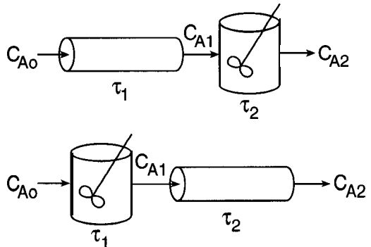
Figure 3-10 Combinations of CSTR and PFTR reactors in series.
