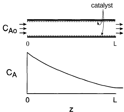
Figure 7-19 Sketch of a catalytic tube wall reactor with gases flowing down the tube and reaction occurring on the walls of the tube, which are coated with a wash coat of catalyst (dots).
