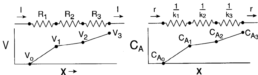
Figure 9-14 Analogy of voltage drop and concentration changes for processes in series. As long as chemical processes are linear in concentration, these can be written simply.
