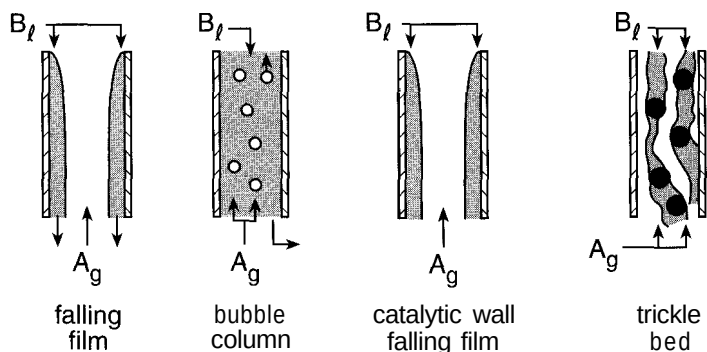
Figure 12-7 Sketches of four types of gas-liquid multiphase reactors.
