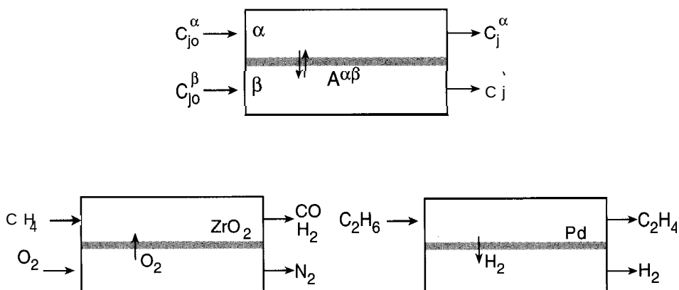
Figure 12-4 Membrane reactor in which a catalyst promotes reaction in the membrane and maintains reactants and products separate. Examples shown are \text{CH}_4 oxidation to syngas and \text{C}_2\text{H}_6 reduction to \text{C}_2\text{H}_4 . The membrane eliminates \text{N}_2 from the syngas and produces \text{C}_2\text{H}_4 beyond equilibrium by removing \text{H}_2 in these applications.
