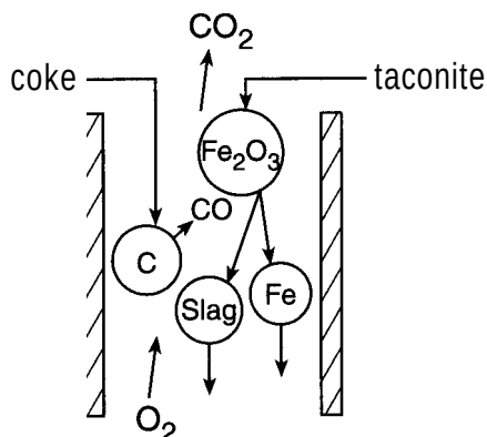
Figure 12-22 Phases and flows in iron ore refining in a blast furnace.
