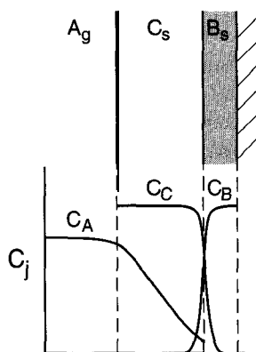
Figure 9-12 Concentration profiles of films where one solid B_s reacts with a gas A , to form another solid C_s , which forms a film that covers the shrinking film of B_s . In the sketch we assume that C_A goes to zero at the C-B boundary and that this boundary is fairly sharp.
