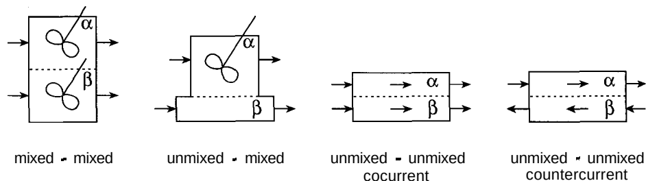
Figure 12-2 Situations for mixed and unmixed phases. Since PFTRs may flow either cocurrent or countercurrent, there are four different configurations for two phases.
