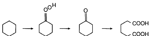
Figure 10-6 Reaction steps to make adipic acid by autooxidation of cyclohexane. Adipic acid is a key ingredient in Nylon.
