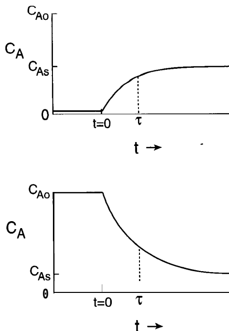
Figure 3-15 Possible transients in CSTR reactors. The upper panel shows the situation starting with pure solvent ( C_A = 0 ) in the reactor initially, C_A = C_{A0} at t = 0 with no reaction. The concentration in the reactor in steady state approaches C_{As} . The lower panel shows the situation where the reactor initially contains pure reactant at C_{A0} , and at t = 0 reactant flow at C_{A0} is begun and eventually approaches a steady-state concentration C_{As} .
