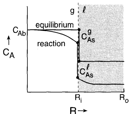
Figure 12-3 Concentration profiles across a gas-liquid interface in equilibrium and with mass flow from left to right. There is a discontinuity in C_A between the gas-liquid and liquid-liquid phases because of differences in equilibrium solubilities.
