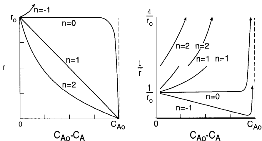
Figure 34 Plots of r and 1/r versus C_{A0} - C_A for the n th-order irreversible reactions.
