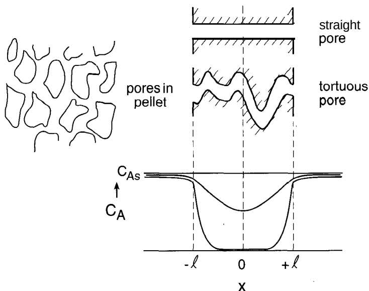
Figure 7-14 Structure and concentration profiles for a planar porous catalyst, which could have straight (honeycomb) or tortuous pores.
