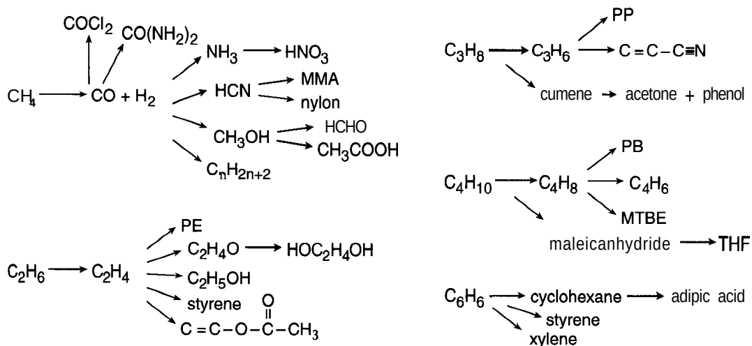
Figure 3-16 Reactions by which \text{CH}_4 , \text{C}_2\text{H}_6 , \text{C}_3\text{H}_8 , and \text{C}_4\text{H}_{10} are converted into chemicals and monomers for common polymers. Most of these are major commercial processes, and most will be expanding considerably as production of natural gas and natural gas liquids expands.
