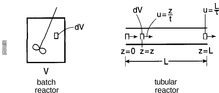
Figure 2-9 Sketch showing correspondence between time in a batch reactor and position z in a plug-flow tubular reactor. The mass-balance equations describe both reactors for the constant-density situations.
