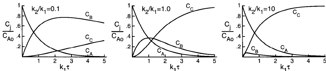
Figure 4-4 C_A , C_B , and C_C versus k_1\tau for series reactions A \rightarrow B \rightarrow C in a PFTR. Plots shown are for k_2/k_1 = 0.1 , 1.0, and 10. The yield to form B exhibits a maximum at a particular residence time \tau_{\max} .
