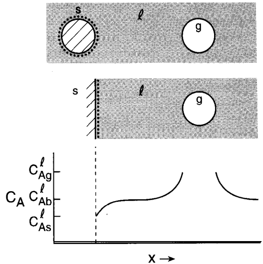
Figure 12-15 Sketch of concentration profiles between a spherical bubble and a solid spherical catalyst particle in a continuous liquid phase (upper) in a gas-liquid slurry reactor or between a bubble and a planar solid wall (lower) in a catalytic wall bubble reactor. It is assumed that a reactant A must migrate from the bubble, through the drop, and to the solid catalyst surface to react. Concentration variations may occur because of mass transfer limitations around both bubble and solid phases.
