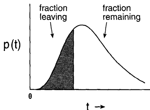
Figure 8-2 Fractions of fluid that have left a reactor and remain in the reactor in terms of p(t) .
