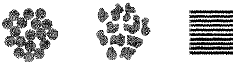
Figure 7-5 Porous catalyst pellets consisting of spheres or grains pressed together into spheres or cylinders. Reactants must diffuse into the pellet in the space between spheres or grains and products must diffuse out of the pellet for reaction to occur. At the right is shown a monolith catalyst in which a ceramic is coated with a wash coat (gray) of porous catalyst.
