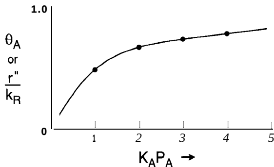
Figure 7-23 Langmuir isotherm of coverage \theta_A versus K_A P_A and rate of reaction r'' for a unimolecular surface-catalyzed reaction A \rightarrow products.
