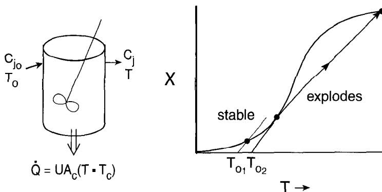
Figure 10-10 Heat generation and removal for combustion reaction in a CSTR. When the feed temperature increases slightly, the rate can go from nearly zero to nearly completion when the heat removal curve becomes tangent to the heat generation curve, and the steady-state temperature jumps to a high value. This simple model shows why these processes can be extremely sensitive to conditions such as size, heat transfer, and the temperature of surroundings.
