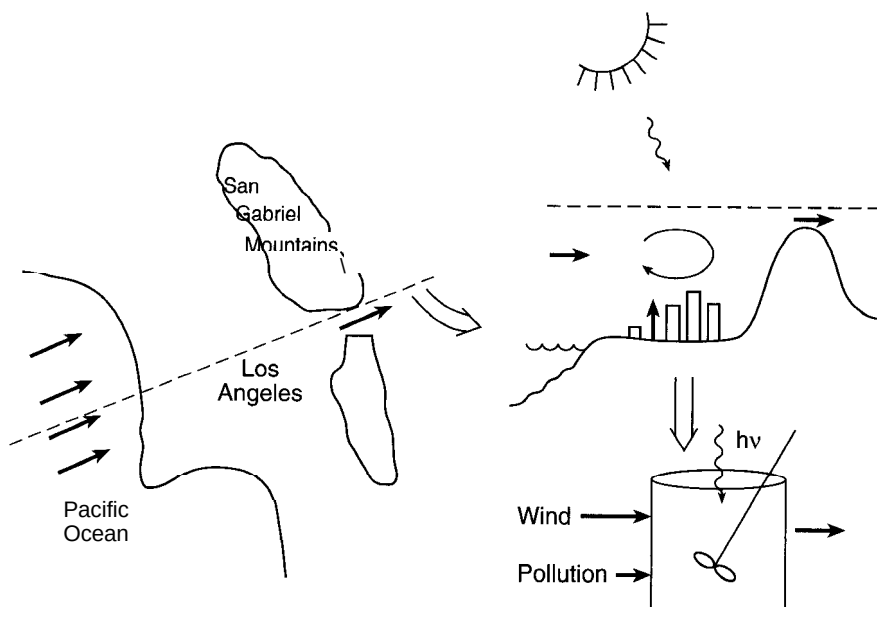
Figure 8-15 Sketch of Los Angeles and simplified CSTR model of air in the LA basin.
