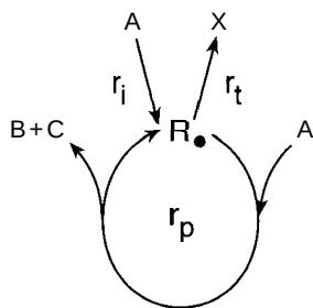
Figure 10-2 Sketch of a simple generic chain reaction A \rightarrow B + C propagated by a radical species R^\bullet .
