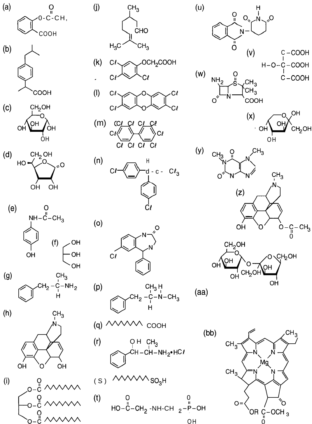
Figure 1-I Some very important organic chemicals that are either made in nature or by us.
