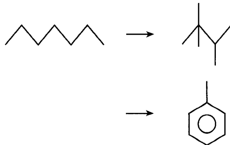
Figure 2-15 Reactions in catalytic reforming of n-heptane to 2,2,3-trimethylbutane and toluene.
