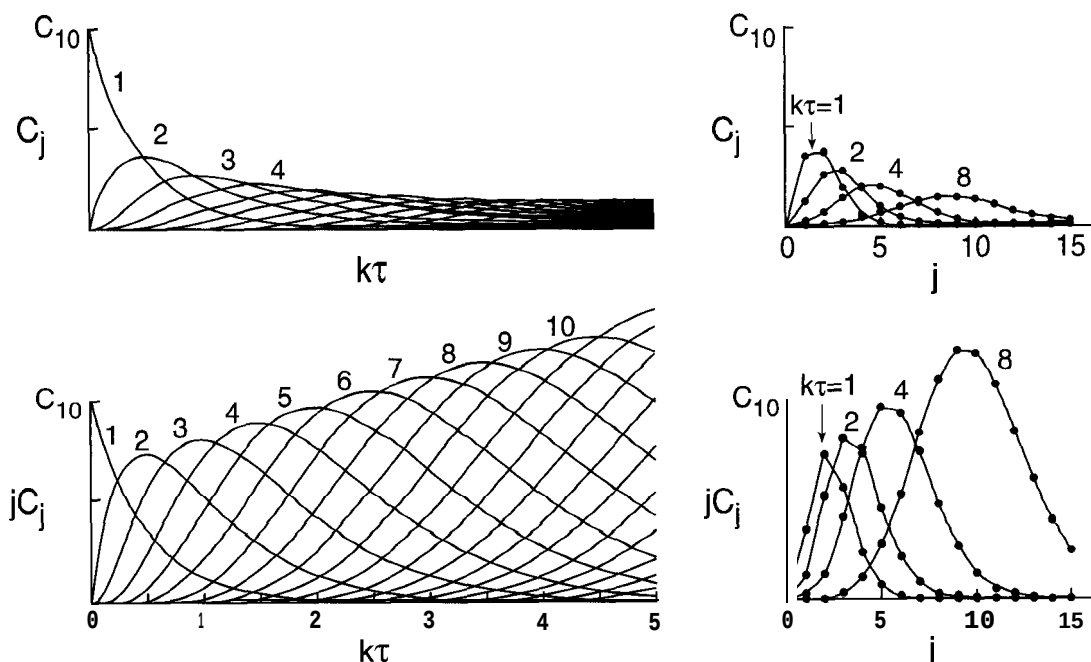
Figure 11-4 Typical distribution of polymer sizes determined on molecule and weight bases.
