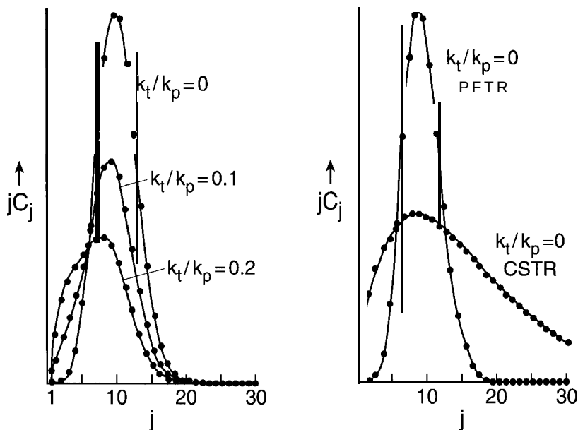
Figure 11-S Average polymer size and size distribution.
