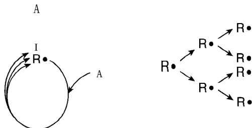
Figure 10-9 Sketch of chain branching reactions where the propagation steps produce more than one radical so that the process tends to grow exponentially, leading to a rapid acceleration of the reaction and possibly a chain-branching explosion.
