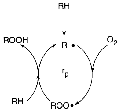
Figure 10-3 Chain reaction for alkane oxidation by autooxidation in which the alkyl and alkylperoxy radicals propagate the chain, which is fed by the alkane RH.
