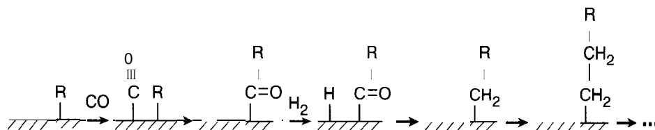
Figure 11-9 Proposed mechanism for Fisher-Tropsch polymerization of CO and \text{H}_2 to form an alkane polymer.
