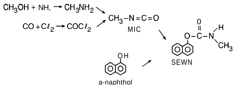
Figure 10-16 Reaction steps to prepare SEVIN, a common agricultural pesticide. All of the reactants are quite inert and harmless except phosgene, MIC, and the final product.
