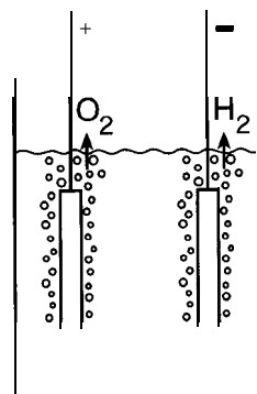
Figure 7-28 Electrochemical reactor in which water is electrolyzed into \text{H}_2 and \text{O}_2 by application of a voltage sufficient to dissociate \text{H}_2\text{O} in a batch reactor configuration.
