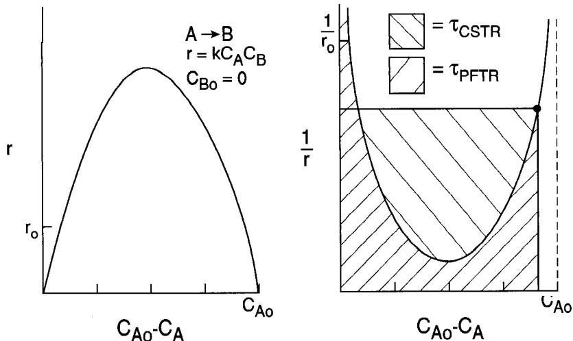
Figure 3-12 Plots of r and 1/r versus C_{A0} - C_A for the autocatalytic reaction A \rightarrow B , r = kC_A C_B . The PFTR requires infinite residence time if no B is added to the feed.
