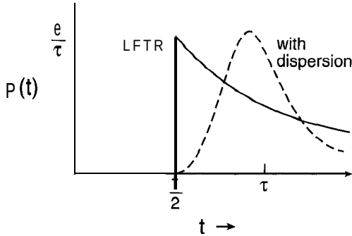
Figure 8-5 Residence time distribution in a laminar flow tubular reactor. The dashed curve indicates the p(t) curve expected in laminar flow after allowing for radial diffusion, which makes p(t) closer to the plug flow.
