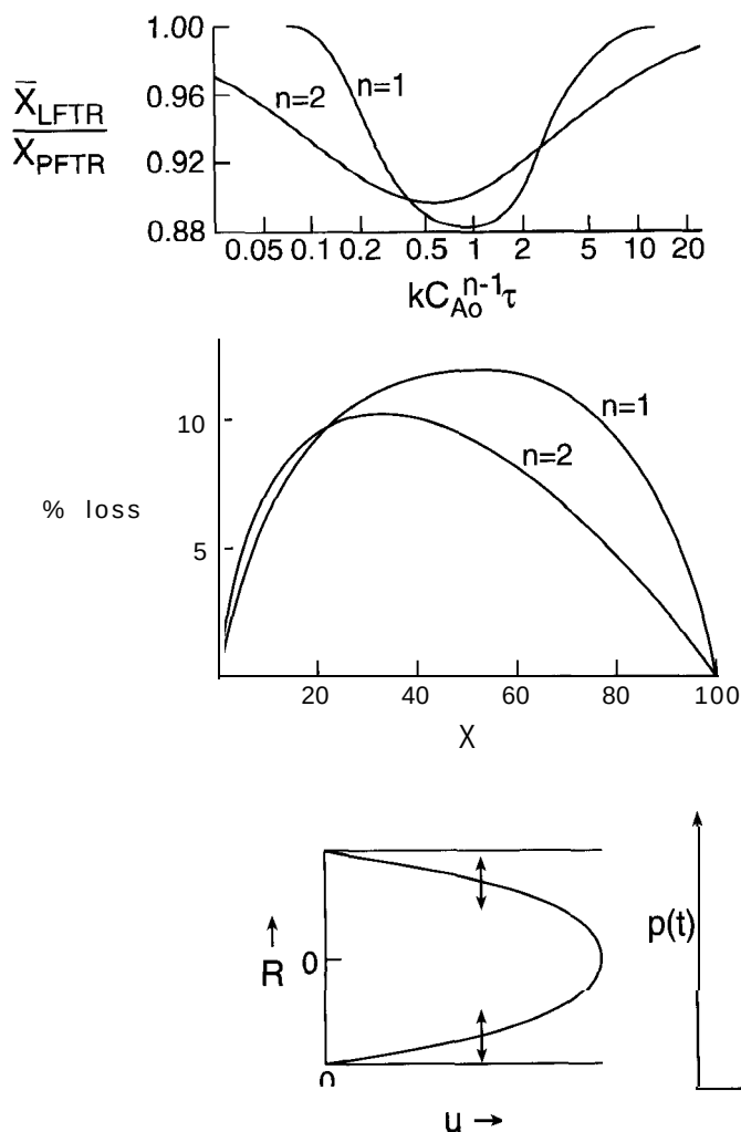
Figure 8-7 Effect of radial mixing on flow profile and p(t) .
