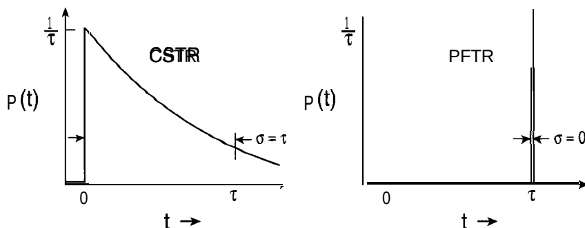
Figure 8-3 Residence time distributions p(t) in an ideal PFTR and CSTR.
