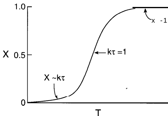
Figure 6-1 Plot of conversion X versus temperature for an irreversible first-order reaction in a CSTR.
