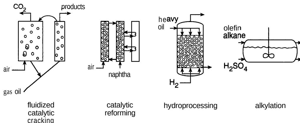
Figure 12-23 Sketches of the four major chemical reactors in petroleum refining. These were considered first in Chapter 2, but now they are seen to be multiphase catalytic reactors using catalysts and requiring careful design for heat transfer and mass transfer.
