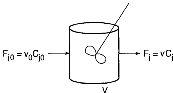
Figure 3-1 The continuous stirred tank reactor (CSTR) of volume V with inlet molar flow rate F_{j0} and outlet molar flow rate F_j
