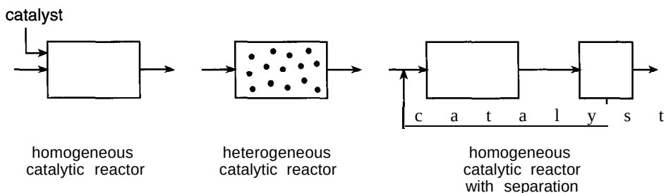
Figure 7-2 Homogeneous catalysts must be separated from the reaction products and returned to the reactor while heterogeneous catalysts can be easily retained in the reactor.
