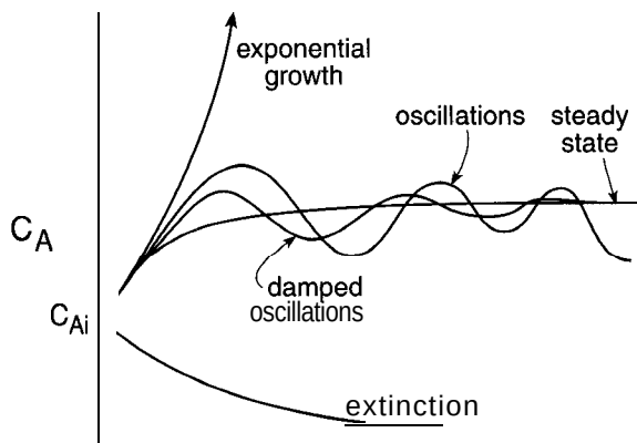
Figure 6-5 Possible transients in a CSTR following small perturbations from the steady state x_s . If \lambda is real, the solution will return to x_s if \lambda < 0 but not if \lambda > 0 . If \lambda is complex, the system will exhibit either damped or growing oscillations depending on whether the real part of \lambda is positive or negative.
