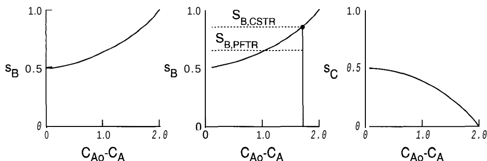
Figure 4-10 Differential selectivity s_B versus conversion C_{A0} - C_A for situations where the desired reaction has a lower order and where the desired reaction has a higher order. The overall selectivity S_B increases or decreases for these situations. The overall selectivity in the CSTR will be higher than in the PFTR if the desired reaction has a lower order.
