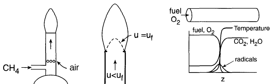
Figure 10-11 Bunsen burner, which is a typical premixed flame in which the flame velocity u_f equals the flow velocity u in the expansion at the end of the tube, creating a stable flame.
