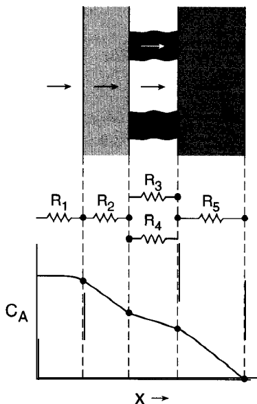
Figure 9-15 Analogy of series and parallel resistors for transformations in composite films.
