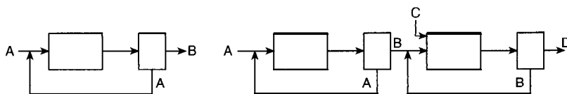
Figure 3-20 Sketch of a single-stage reactor with product separation and recycle and also two stages where reactants from the first stage are separated and recycled into the first reactor while products are mixed with other reactants and fed into a second stage.
