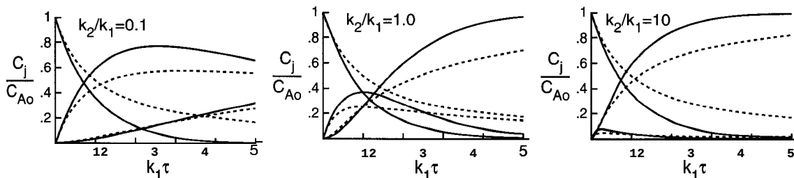
Figure 4-6 Comparison of concentrations in the reactions A \rightarrow B \rightarrow C in a PFTR (solid curves) and CSTR (dashed curves). The PFTR is seen to give a larger Y_B and shorter \tau for maximum yield of B .
