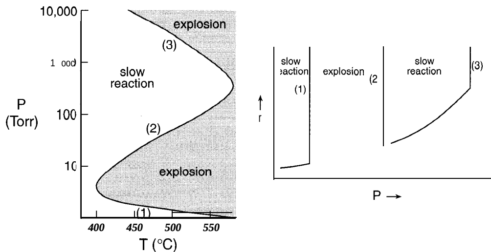
Figure 10-8 Explosion limits of the \text{H}_2 + \text{O}_2 reaction. At low pressures explosion is determined by the quenching of chain branching of radicals at the walls of the vessel, while at high pressures the larger rate of heat generation leads to a thermal explosion,
