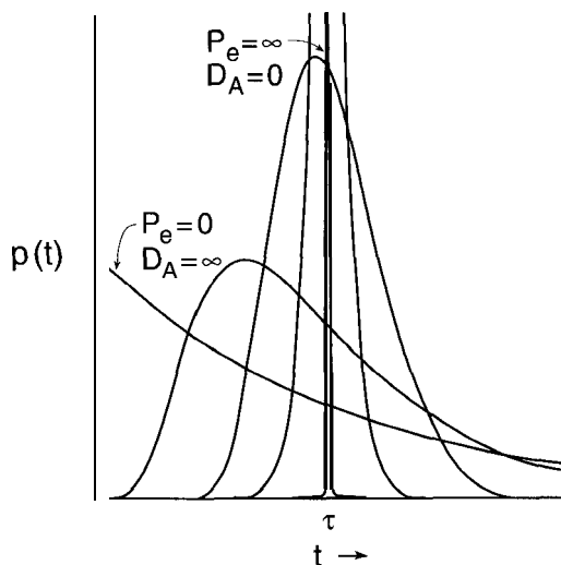
Figure S-9 Plots of p(t) versus Pe in a tubular reactor.
