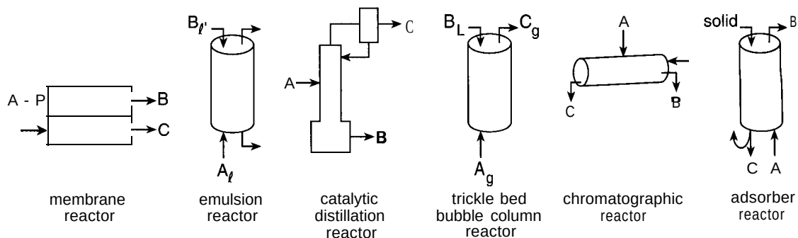
Figure 12-17 Some reactor separation configurations that can produce conversions beyond single-stage equilibrium.
