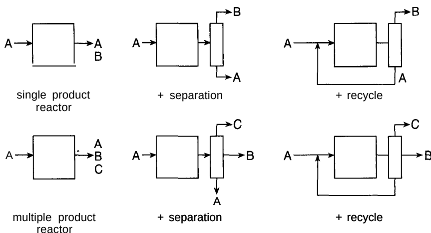
Figure 4-2 Sketches of single reactor and reactor with separation and recycle in which reactant can be fed back into the reactor to increase the overall yield of a process.
