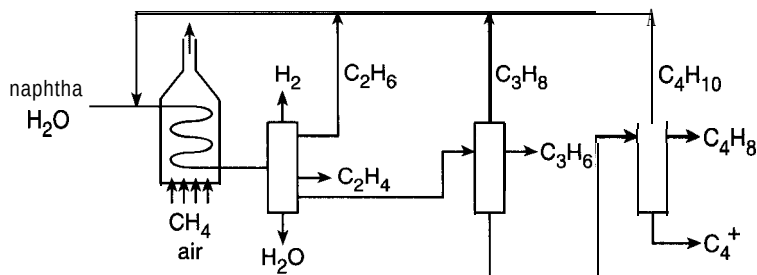
Figure 4-1 Flow sheet of a steam cracking plant to produce olefins from alkanes.
