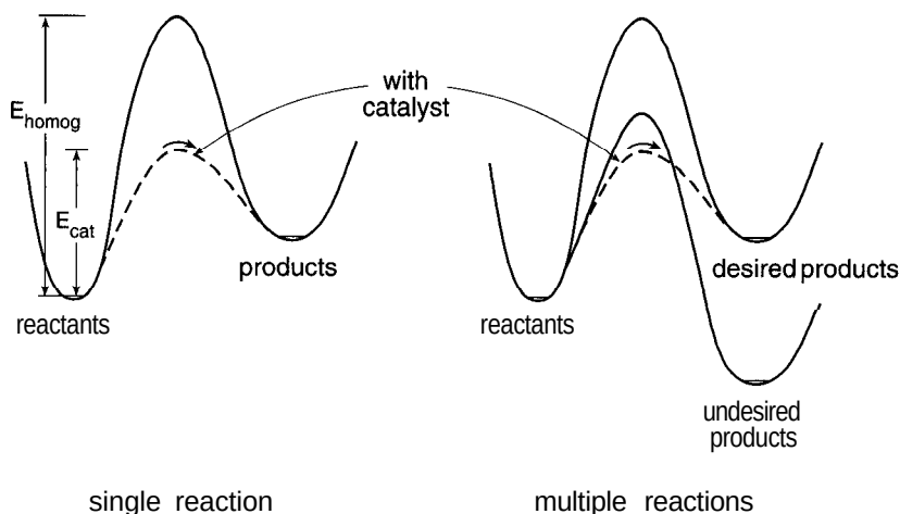
Figure 7-1 Energy diagram showing how a catalyst lowers the barrier for a reaction to improve conversion (left) or lowers the barrier for a desired reaction to improve selectivity (right).
