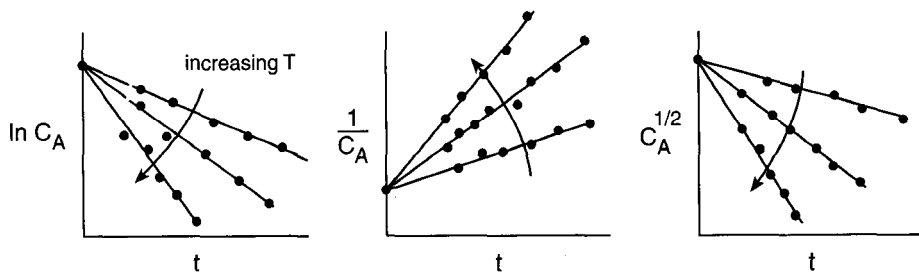
Figure 2-19 Plots of C_A versus time, which give straight lines for an n th-order irreversible reaction. The slopes of these lines give the rate coefficient k .
