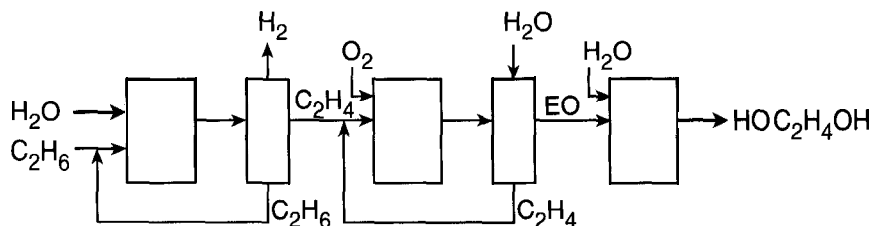
Figure 2-18 Flow sheet of process to produce ethylene glycol from ethane.
