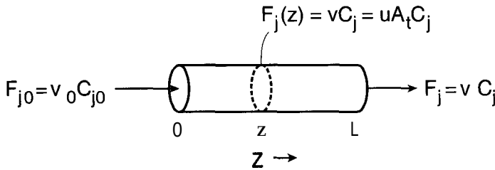
Figure 3-2 The plug-flow tubular reactor (PFTR). The length of the reactor is L , the inlet molar flow rate of species j is F_{j0} , and the outlet flow rate of species j is F_j .
