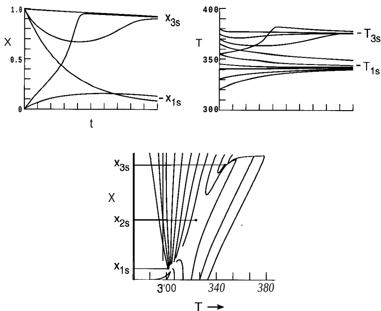
Figure 6-12 Transients in the adiabatic CSTR for the irreversible reaction of the previous example. The upper panels show X(t) and T(t) , while the lower panel displays X(T) for the same curves shown in the upper panel. The system converges on one of the stable steady states but never on the middle unstable steady state.
