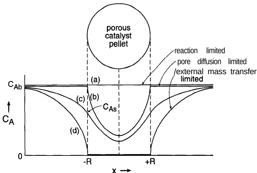
Figure 7-9 Reactant concentration profiles around and within a porous catalyst pellet for the cases of reaction control, external mass transfer control, and pore diffusion control. Each of these situations leads to different reaction rate expressions.
