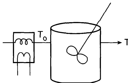
Figure 6-6 Adiabatic CSTR in which feed temperature T_0 is varied.
