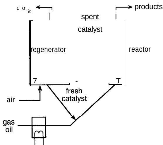
Figure 2-13 Sketch of a fluidized catalytic cracking reactor (FCC) for cracking heavy petroleum fractions into the boiling range needed for gasoline.
