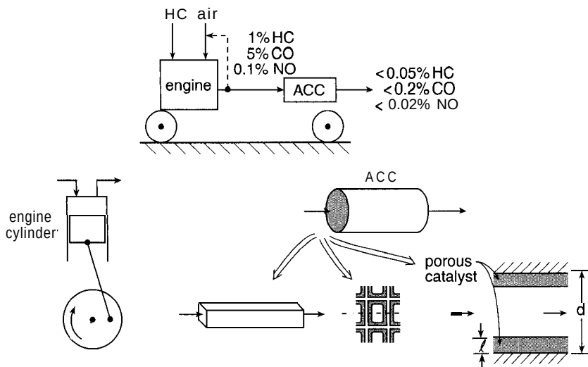
Figure 7-16 A highly simplified sketch of an automobile engine and catalytic converter with typical gas compositions indicated before and after the automotive catalytic converter. The catalytic converter is a tube wall reactor in which a noble-metal-impregnated wash coat on an extruded ceramic monolith creates surface on which reactions occur.
