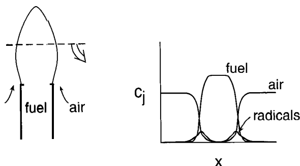
Figure 10-13 Concentration and temperature profiles in a diffusion flame such as a candle. Radical intermediates that propagate the flame have high concentrations in the flame zone between fuel and \text{O}_2 .
