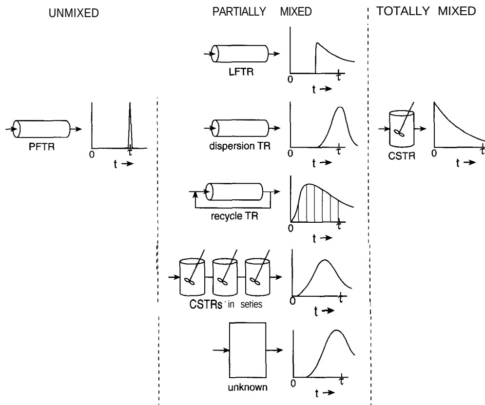
Figure S-13 Residence time distributions for the nonideal reactors considered in this chapter.
