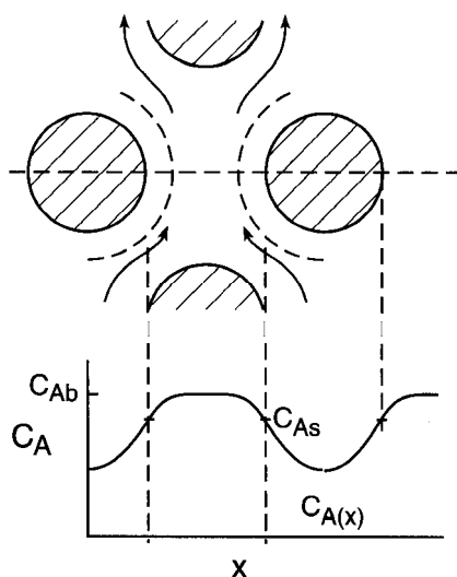
Figure 7-7 Reactant concentration profiles in direction x , which is perpendicular to the flow direction z expected for flow over porous catalyst pellets in a packed bed or slurry reactor. External mass transfer and pore diffusion produce the reactant concentration profiles shown.
