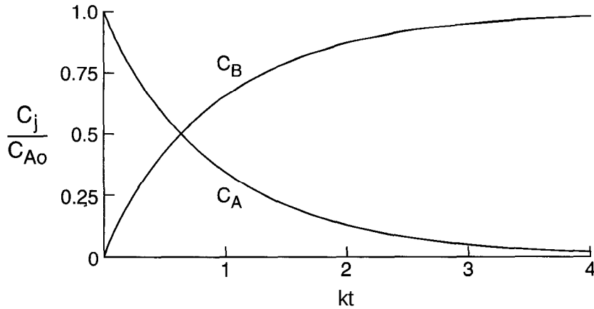
Figure 2-5 Plots of C_A(t) and C_B(t) versus kt for the first-order irreversible reaction A \rightarrow B , r = kC_A in a batch reactor.
