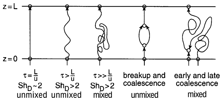
Figure 12-12 Sketches of possible flow patterns of bubbles rising through a liquid phase in a bubble column. Stirring of the continuous phase will cause the residence time distribution to be broadened, and coalescence and breakup of drops will cause mixing between bubbles. Both of these effects cause the residence time distribution in the bubble phase to approach that of a CSTR. For falling drops in a spray tower, the situation is similar but now the drops fall instead of rising in the reactor.
