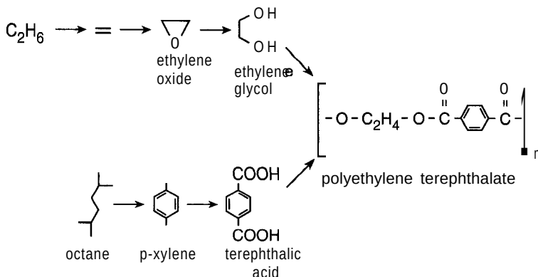
Figure 2-17 Reaction steps to prepare polyethylene terephthalate from ethane and naphtha.
