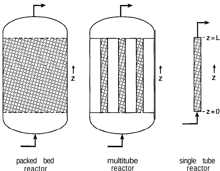
Figure 7-3 Packed bed reactors, which may be a single bed, many tubes, or a single tube filled with catalyst pellets. Multitube reactors allow efficient heat transfer for exothermic or endothermic reactions.
