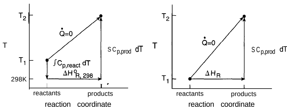
Figure 2-10 Energy diagram illustrating the temperature change in a reaction in which no heat is exchanged with the surroundings, a situation called an adiabatic reactor.
