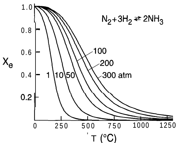
Figure 3-17 Plot of equilibrium conversion X_e versus temperature for ammonia synthesis starting with stoichiometric feed. While the equilibrium is favorable at ambient temperature (where bacteria fix N_2 ), the conversion rapidly falls off at elevated temperature, and commercial ammonia synthesis reactors operate with a Fe catalyst at pressures as high as 300 atm to attain a high equilibrium conversion.
