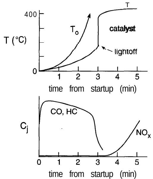
Figure 7-18 Since the reactions in the ACC are strongly exothermic, the catalyst can exhibit multiple steady states as the catalyst suddenly lights off as the car is started and the temperature rises to the ignition temperature, which then causes a rapid increase in temperature.
