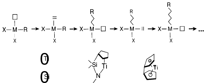
Figure 11-7 Proposed mechanism for catalytic polymerization. An olefin and an alkyl group on an organometallic site react to add the olefin to the growing chain. Also shown are typical polymerization catalysts: Ti/Si solid catalyst and organometallic metallocene catalysts.
