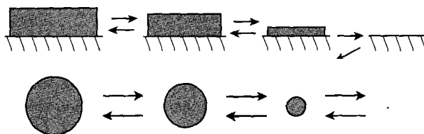
Figure 9-5 Sketches of shrinking or growing films and particles, with arrows going either forward or backward as the process progresses. Reaction is assumed to occur only at the interface of the solid with the fluid.
