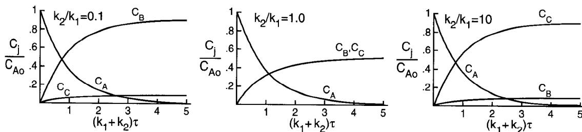
Figure 4-7 C_A , C_B , and C_C versus (k_1 + k_2)\tau for parallel reactions A \rightarrow B , A \rightarrow C in a PFTR. Plots shown are for k_2/k_1 = 0.1 , 1.0, and 10. The selectivity to B and yield of B are independent of conversion for equal-order kinetics.
