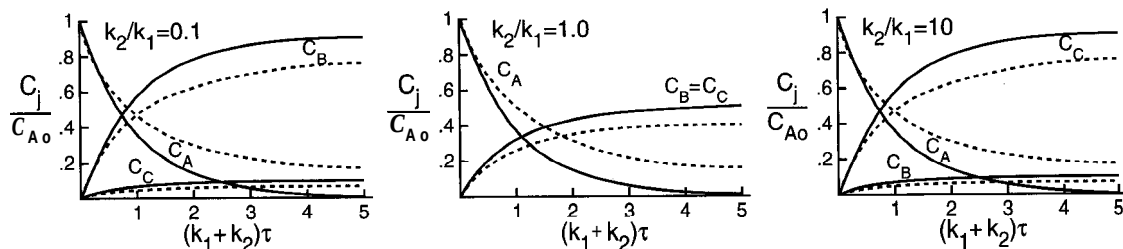
Figure 4-9 Comparison of C_A , C_B , and C_C for parallel first-order reactions in a PFTR (solid curves) and CSTR (dashed curves).
