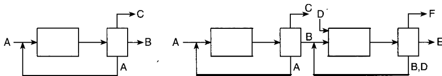
Figure 4-15 Sketch of a two-stage process where the reactant A from the first reactor is separated from the desired product B and the undesired product C . The desired product B is then fed into a second reactor, where another reactant D may be added to make a desired product E and an undesired product F , which are further separated.
