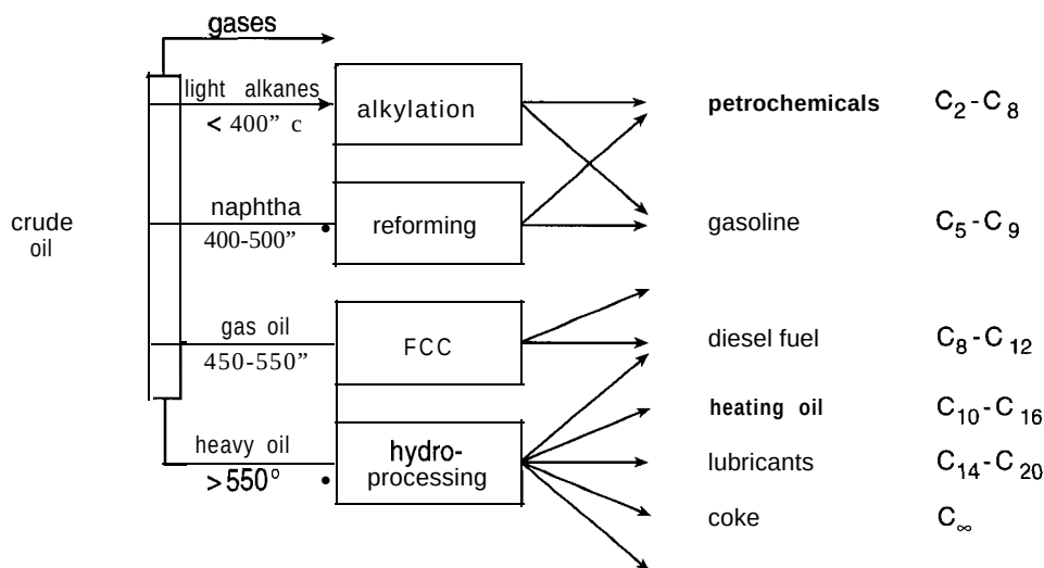
Figure 2-12 Qualitative flow sheet of reactants, reactors, and products in petroleum refining.
