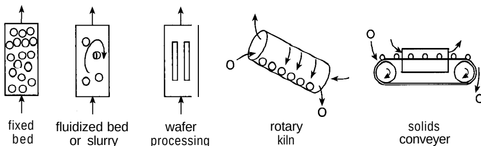
Figure 9-2 Typical continuous reactors for processing solids. Solids handling and particular solid products frequently require configurations not common in processing fluids.
