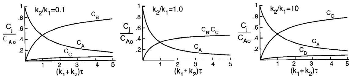
Figure 4-8 C_A , C_B , and C_C versus (k_1 + k_2)\tau for parallel reactions A \rightarrow B , A \rightarrow C in a CSTR. Plots shown are for k_2/k_1 = 0.1 , 1.0, and 10. The selectivity to B and yield of B are independent of conversion for equal-order kinetics. The selectivities and yields are the same for both PFTR and CSTR, but the CSTR requires a longer \tau for a given conversion.
