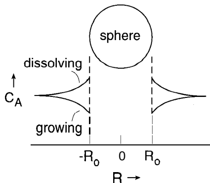
Figure 9-11 Concentration profiles around growing or dissolving sphere. The dissolving case implies a product species.
