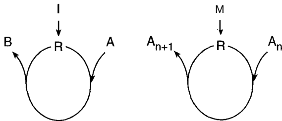
Figure 11-2 Sketch of simple ideal chain reaction not involving polymerization (left) and where a long-chain polymer is formed by adding monomer successively (right).
