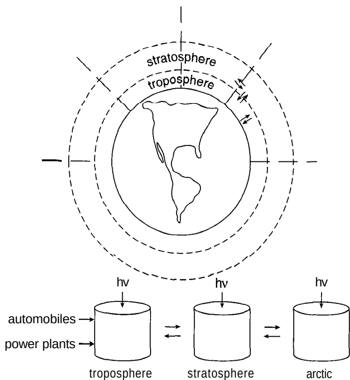
Figure S-16 A sketch of the global environment broken into several mixed regions (CSTRs), each with specific chemical reactions and residence times.
