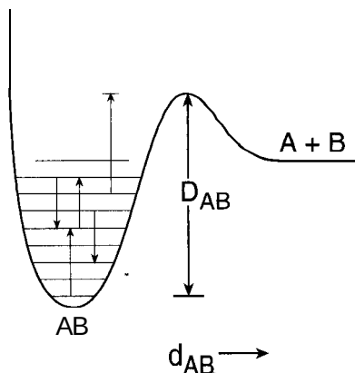
Figure 4-13 Energy diagram for the dissociation of a molecule into two products.
