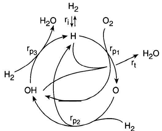
Figure 10-7 Sketch of chain reaction in \text{H}_2 + \text{O}_2 \rightarrow \text{H}_2\text{O} . This is a highly simplified set of the reactions shown in the table, which indicate the dominant chain reaction steps in forming water from three chain-propagating radical species: H, O, and OH.
