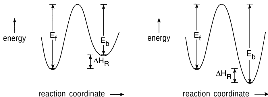
Figure Z-3 Plot of energy of reactants and products in a chemical reaction versus the reaction coordinate. The activation energy for the forward reaction is E_f , for the back reaction E_b , and the heat of the reaction is \Delta H_R = E_f - E_b . The curve at the left is for an endothermic reaction ( E_f > E_b ), while the curve at the right is for an exothermic reaction ( E_f < E_b ).
