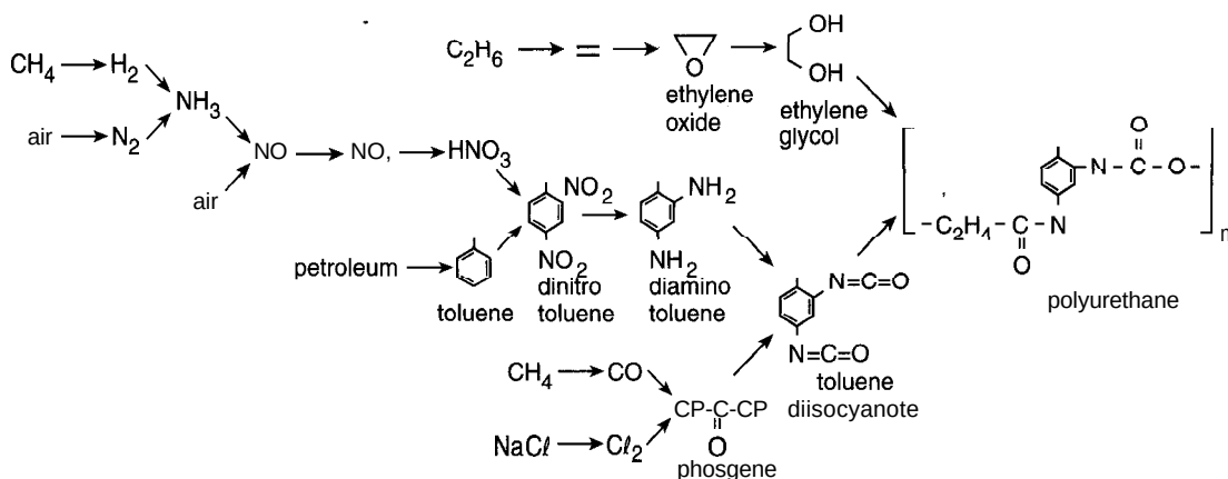
Figure 3-21 Reactions in production of polyurethane. These processes involve many of the individual reaction steps discussed previously.
