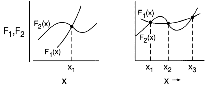
Figure 6-2 Graphical solution to the equation F_1(x) = F_2(x) for situations with 1 and 3 intersections (solutions).
