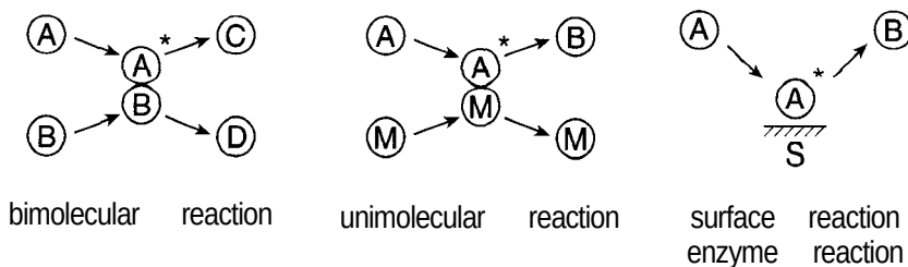
Figure 4-12 Elementary reaction steps involving collisions of two reactants A and B , of A with an inert M , or with A with a surface S .
