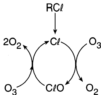
Figure 8-17 The chain reaction by which small concentrations of organic chlorine compounds produce ozone destruction in the stratosphere.
