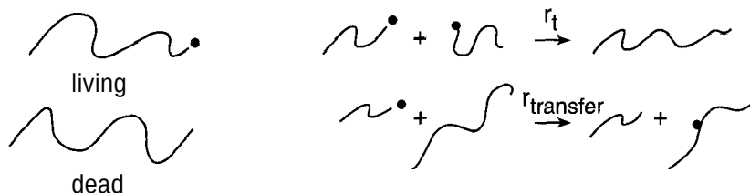
Figure 11-6 Sketches of living and dead polymers.
