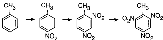
Figure 3-19 Successive reactions in the nitration of toluene. These reactions can be described as series reactions A \rightarrow B \rightarrow C \rightarrow D , which are a type of multiple reactions that will be considered in the next chapter.
