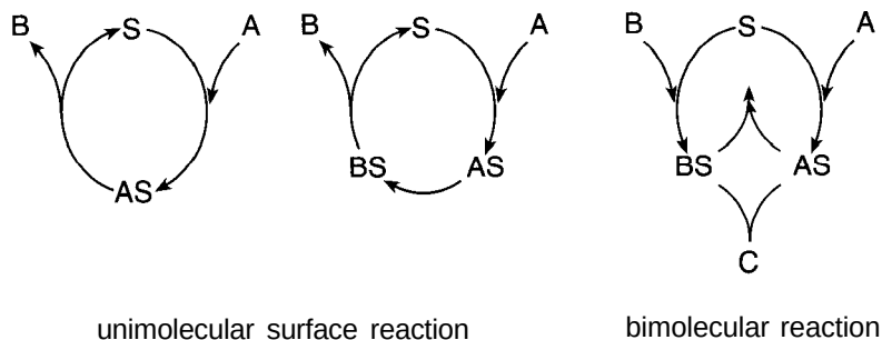
Figure 7-22 Catalytic cycle in which reactant A adsorbs on a vacant surface site S to form the adsorbate AS , which reacts to form BS . The product B then desorbs to form the original vacant site S , which allows the catalytic process to continue indefinitely in a cycle.
