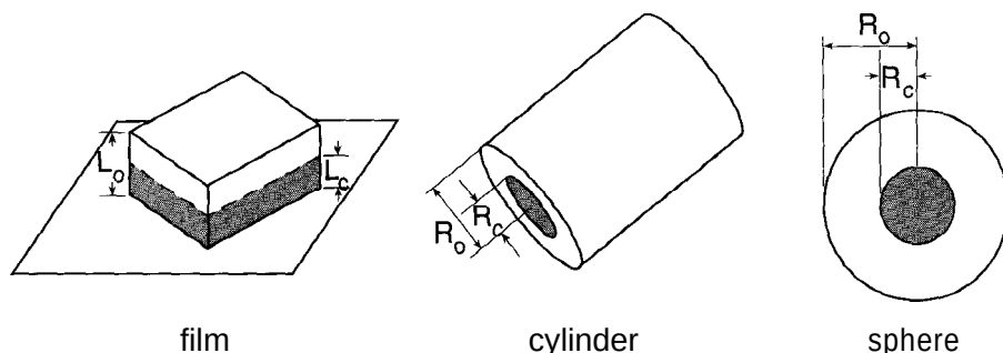
Figure 9-4 Geometries of films, cylinders, and spheres as one-, two-, and three-dimensional reacting solids. The gray region is unreacted B_s , while the white region is solid product C_s .
