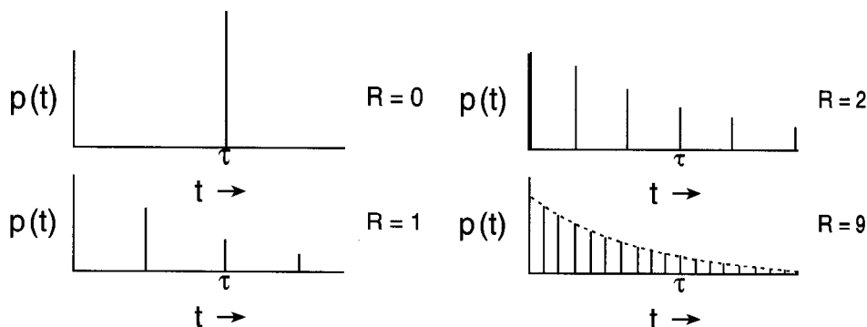
Figure S-11 p(t) for a tubular reactor with increasing recycle.
