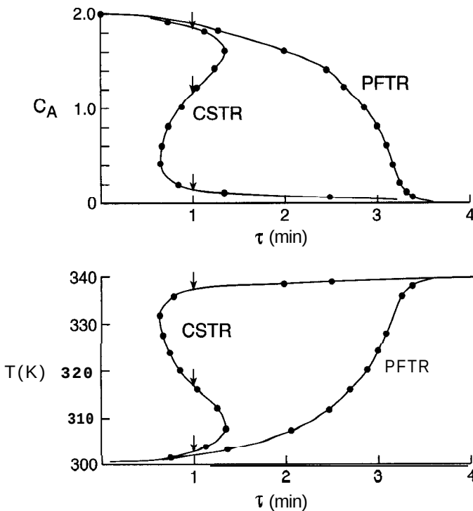
Figure 5-10 Residence times in a PFTR and CSTR for adiabatic reactors. The CSTR can require a much smaller \tau than the PFTR and can exhibit multiple steady states for some \tau (arrows).
