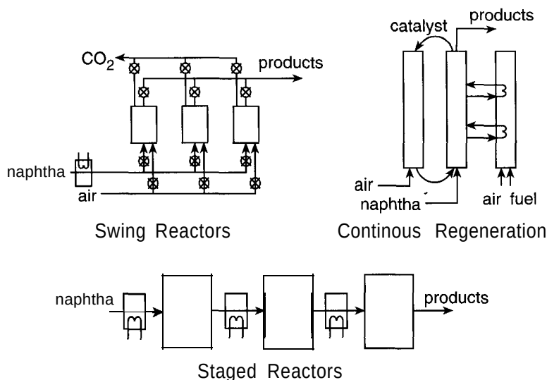
Figure 2-16 Several reactor configurations for catalytic reforming to produce high-octane gasoline.
