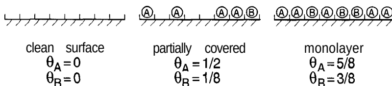
Figure 7-21 Densities of molecules adsorbed in a monolayer on surfaces
