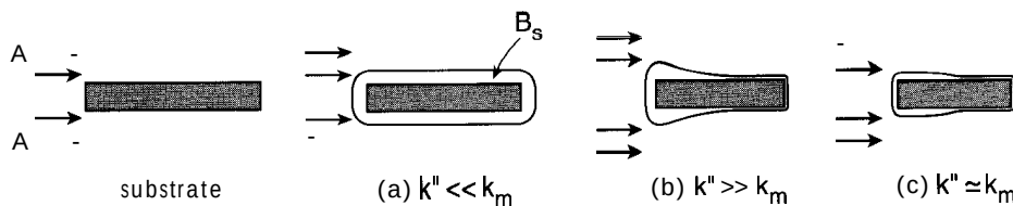
Figure 9-10 Sketches of film profiles for chemical vapor deposition over a flat plate with reactant gases flowing from left to right. Reaction-limited deposition should produce a uniform film (a), while mass-transfer-limited Row should produce a thicker film near the leading edge (b).
