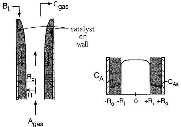
Figure 12-13 A falling film catalytic wall reactor in which reactant in the gas must diffuse through a liquid film to react on a catalyst which coats the wall of the reactor.
