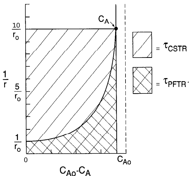
Figure 3-5 Residence times in CSTR (shaded rectangle) and PFTR (area under curve) from the 1/r plot.
