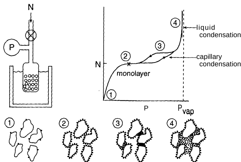
Figure 7-24 Adsorption equilibrium apparatus to determine adsorption isotherms and surface areas of catalysts. From the saturation of a sample of known weight, the surface area can be determined if the area occupied by a molecule is known. (Adsorbed molecules are dots.)
