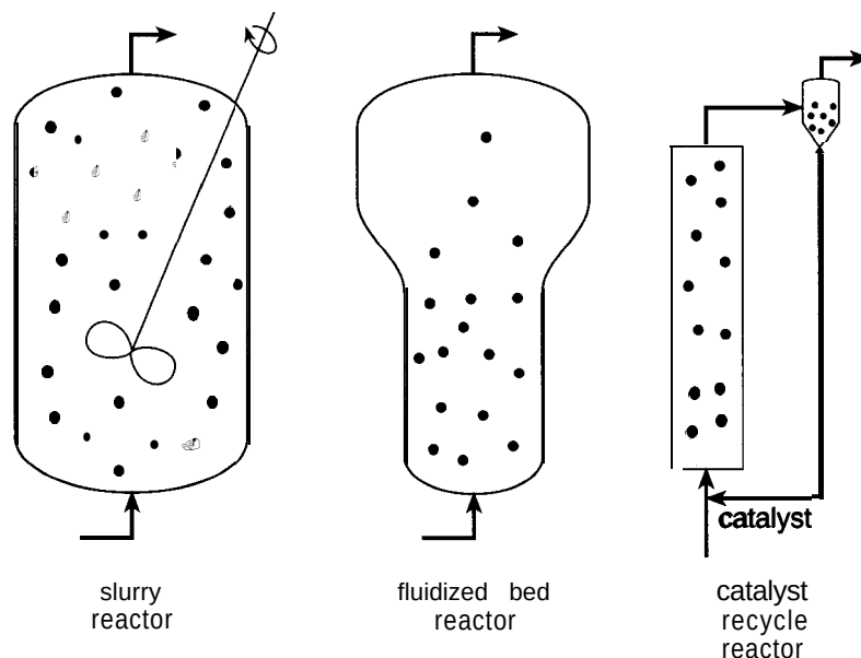
Figure 7-4 Slurry reactor (left) for well-mixed gas-solid reactions and fluidized bed reactor (center) for liquid-solid reactions. At the right is shown a riser reactor in which the catalyst is carried with the reactants and separated and returned to the reactor. The slurry reactor is generally mixed and is described by the CSTR model, while the fluidized bed is described by the PFTR or CSTR models.
