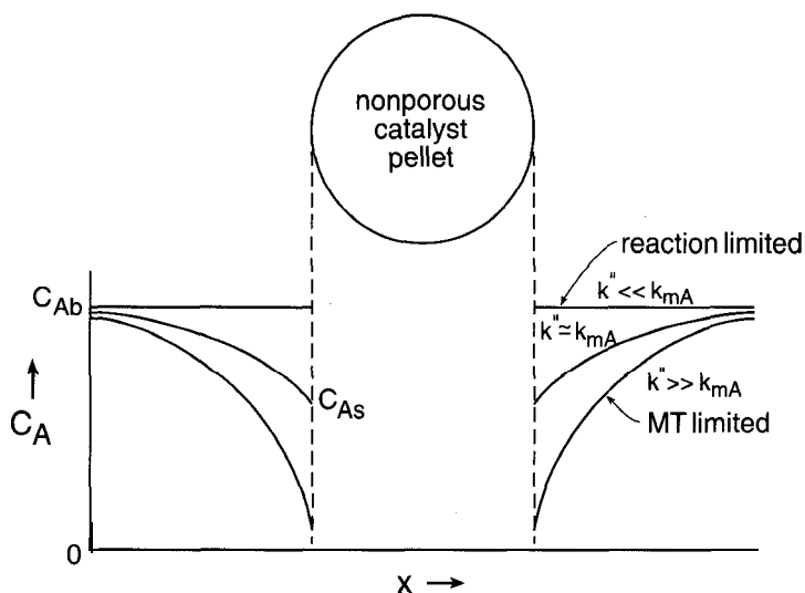
Figure 7-10 Reactant concentration profiles around a catalyst pellet for reaction control ( k_m \gg k'' ) and for external mass transfer control ( k_m \ll k'' ).
