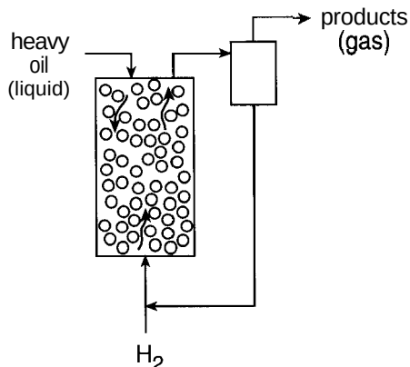
Figure 2-14 Sketch of a trickle bed reactor used for hydroprocessing of the residual oil fraction of crude oil into the boiling range used for gasoline and diesel fuel.
