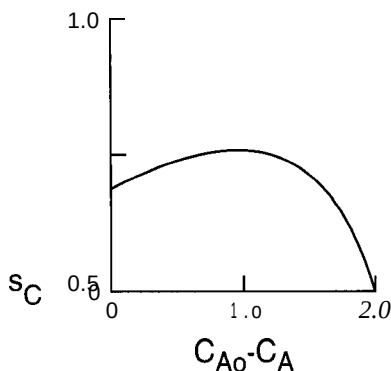
Figure 4-11 Plot of differential selectivity s_C for the example of three reactions in parallel. If C is desired, the CSTR gives a larger S_C , and this occurs when the reactor is operated at C_A = 1 mole/liter.
