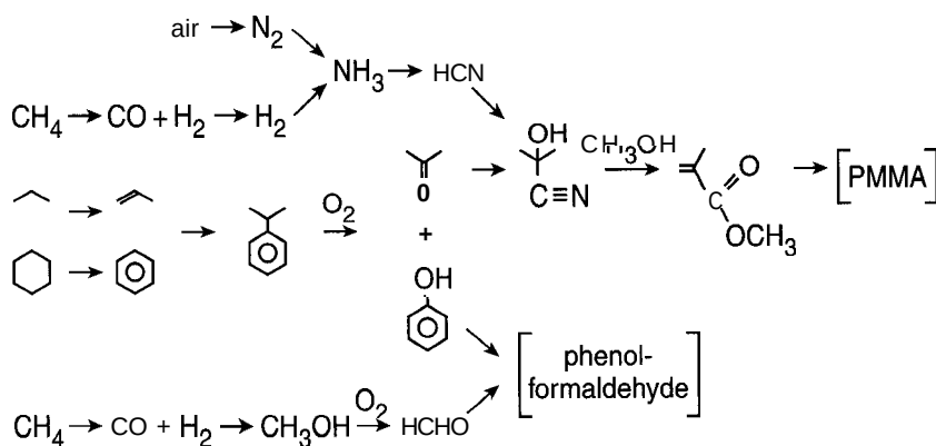
Figure 11-10 Flowsheet of an integrated process to produce PMMA and phenol-formaldehyde polymers simultaneously starting from methane, propane, and cyclohexane through a cumene intermediate.
