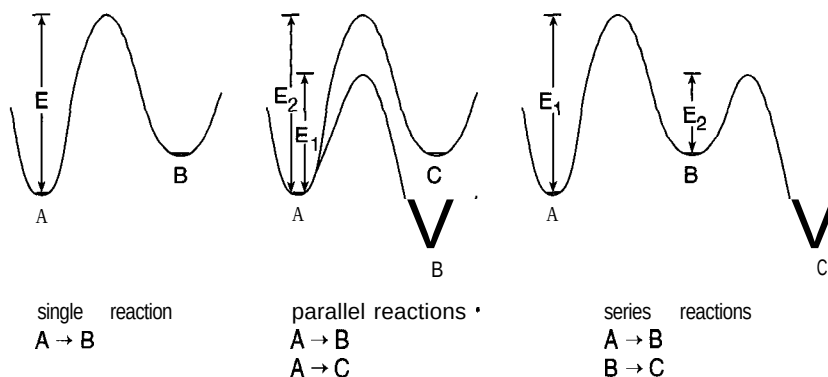
Figure 4-3 Energy diagrams for a single reaction (left) and for parallel reactions (center) and series reactions (right). For parallel and series reactions there are several activation energies that must be considered in describing selectivity and yield of a desired product.
