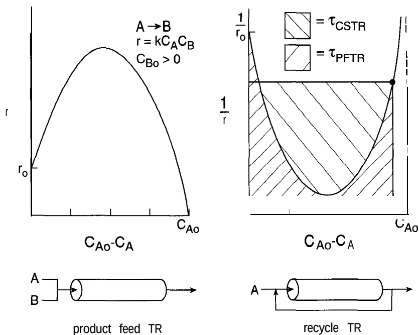
Figure 3-13 Possible tubular reactor configurations for autocatalytic reactions. With large recycle, the tubular reactor performance approaches that of a CSTR, as will be considered in Chapter 8.
