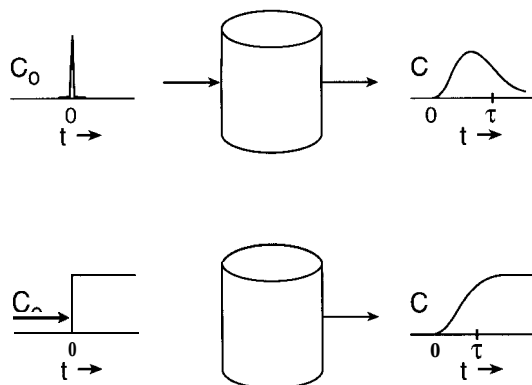
Figure 8-1 Sketch of response to a pulse injection \delta(t) of a tracer (upper) and response to a step injection of a tracer (lower) in a steady state chemical reactor with an arbitrary flow pattern. The response to a pulse injection is the residence time distribution p(t) , and the derivative of the step response is p(t) .
