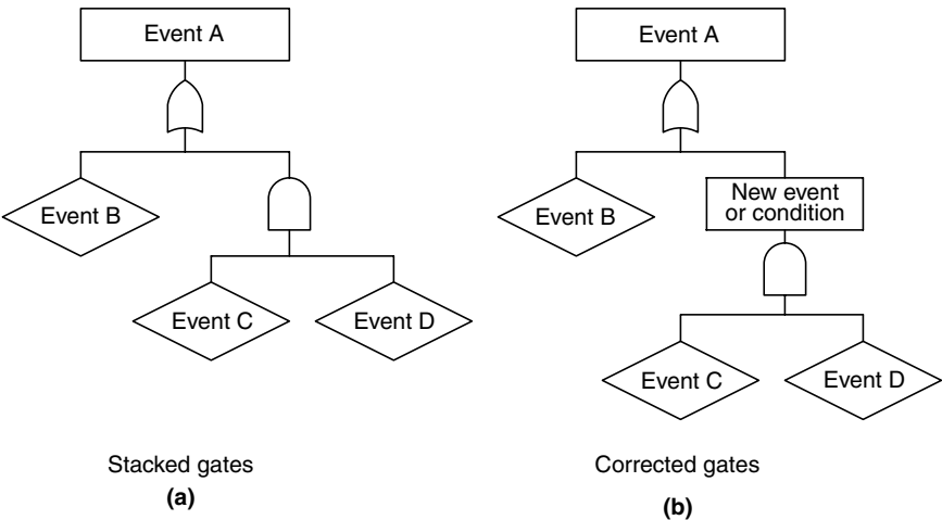
Figure 7.8 Example of improperly stacked gates and correction.
