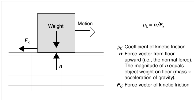
Figure 14.2 Free-body diagram of floor friction to illustrate Newton's Third Law of Motion.
