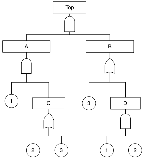
Figure 8.5 Fault tree to illustrate cut sets.
