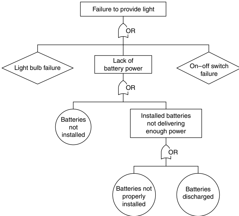
Figure 7.3 Example of a flashlight fault tree.
