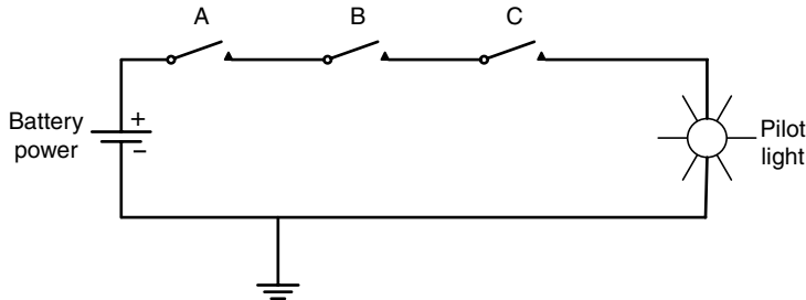
Figure 7.4 Circuit diagram with three normally open switches.
