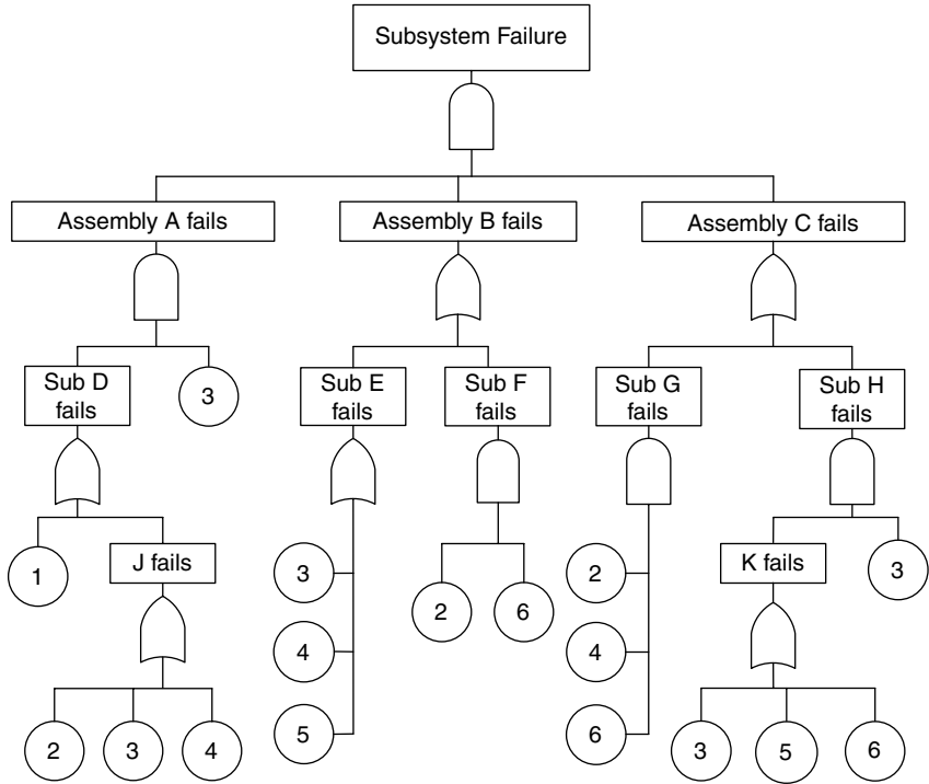
Figure 8.7 Fault tree illustrating a common-cause failure.
