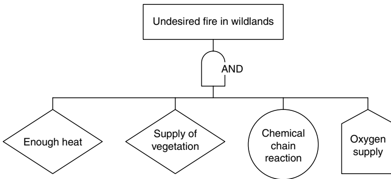
Figure 7.6 First tier of a fault tree for undesired fire in wildlands.
