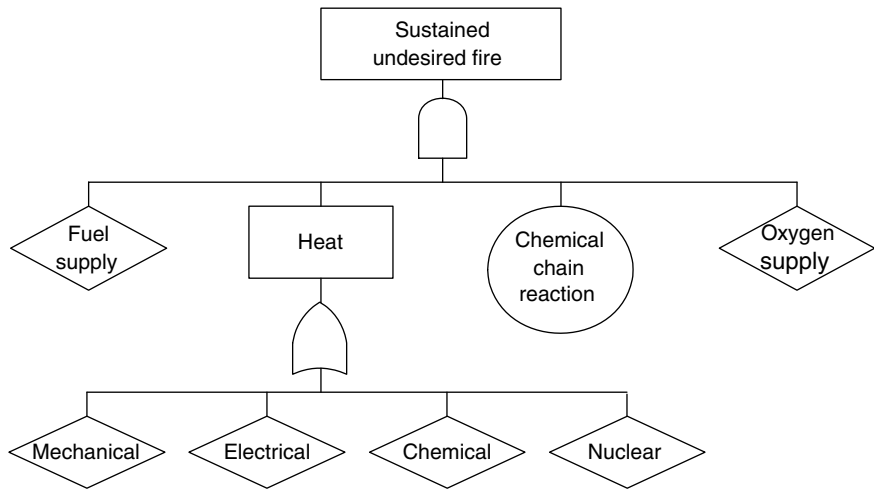
Figure 18.2 Fault tree depicting how a fire can be sustained by any of four alternative heat sources.
