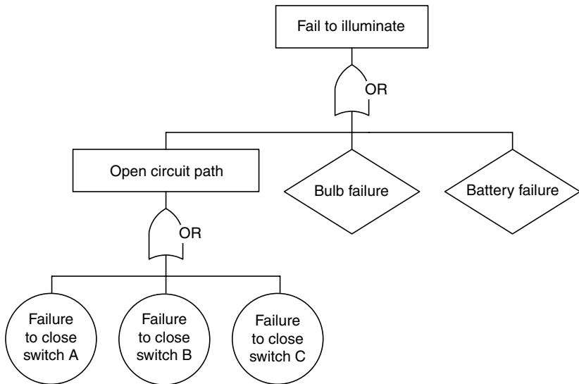
Figure 7.5 Fault tree for circuit in Figure 7.4.
