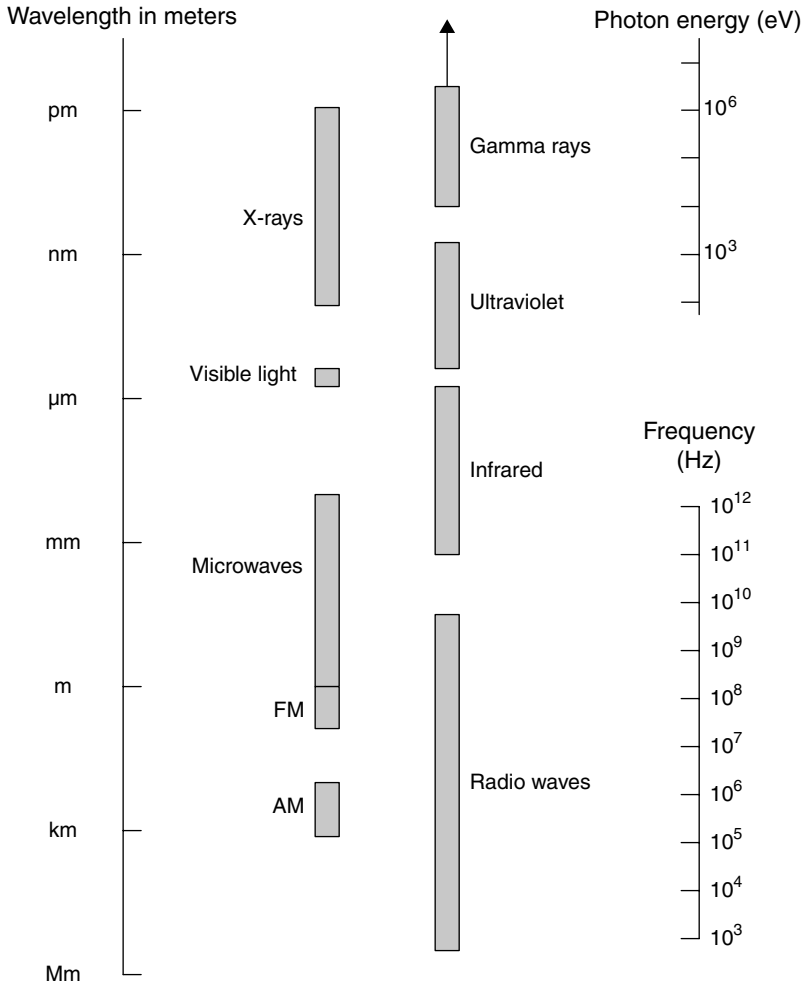
Figure 21.2 Forms of electromagnetic energy arranged by wavelength.
