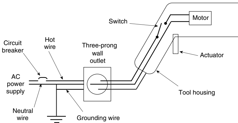
Figure 15.1 Wiring for a power tool plugged into a three-prong receptacle.
