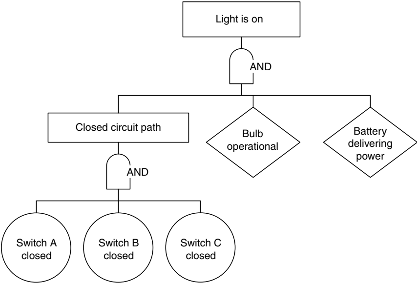
Figure 7.7 Success tree for circuit in Figure 7.4.
