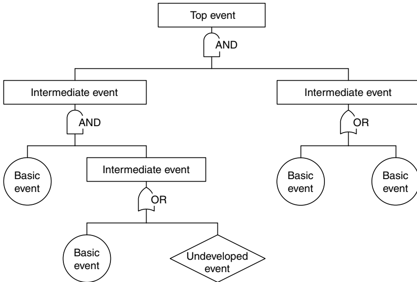
Figure 7.2 General locations of symbols on a typical fault tree.
