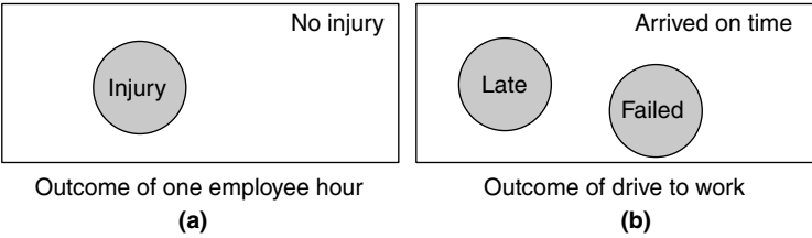
Figure 8.1 Two examples of Venn diagrams.
