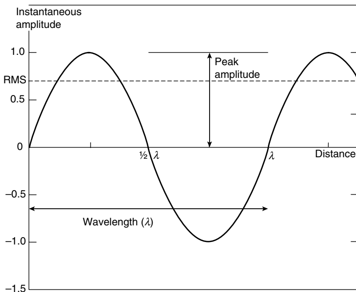
Figure 21.1 Instantaneous amplitude of an oscillating electromagnetic wave plotted against distance.
