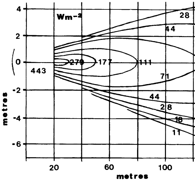
Figure 5.8 Calculated values for the intermediate field in example 2
