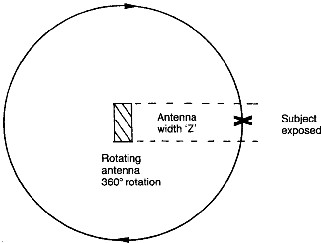
Figure 5.14 Rotating beam power density time-averaging for a subject in the near field case
