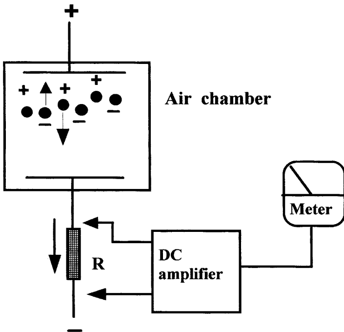
Figure 8.11 Ionisation chamber X-ray measuring instrument – basic concept
