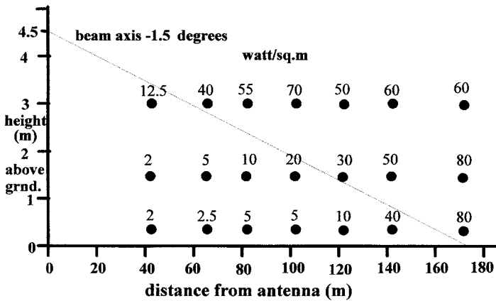
Figure 10.13 Measurement on a microwave beam tilted towards the ground
