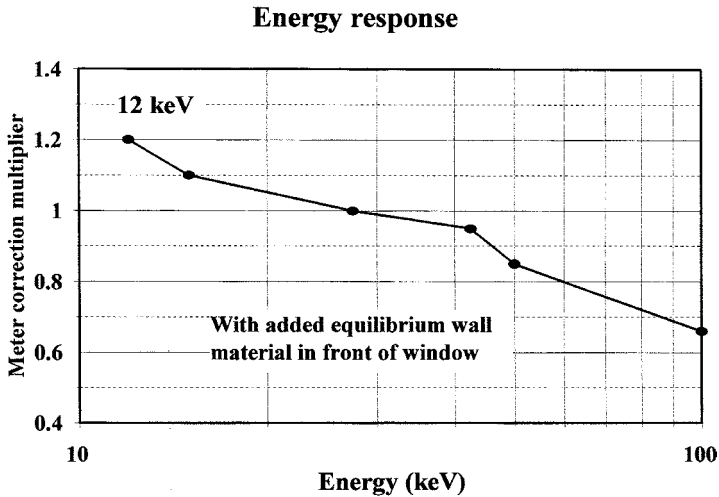
Figure 8.17 Victoreen 440RF/D energy response (Courtesy Victoreen Inc.)
