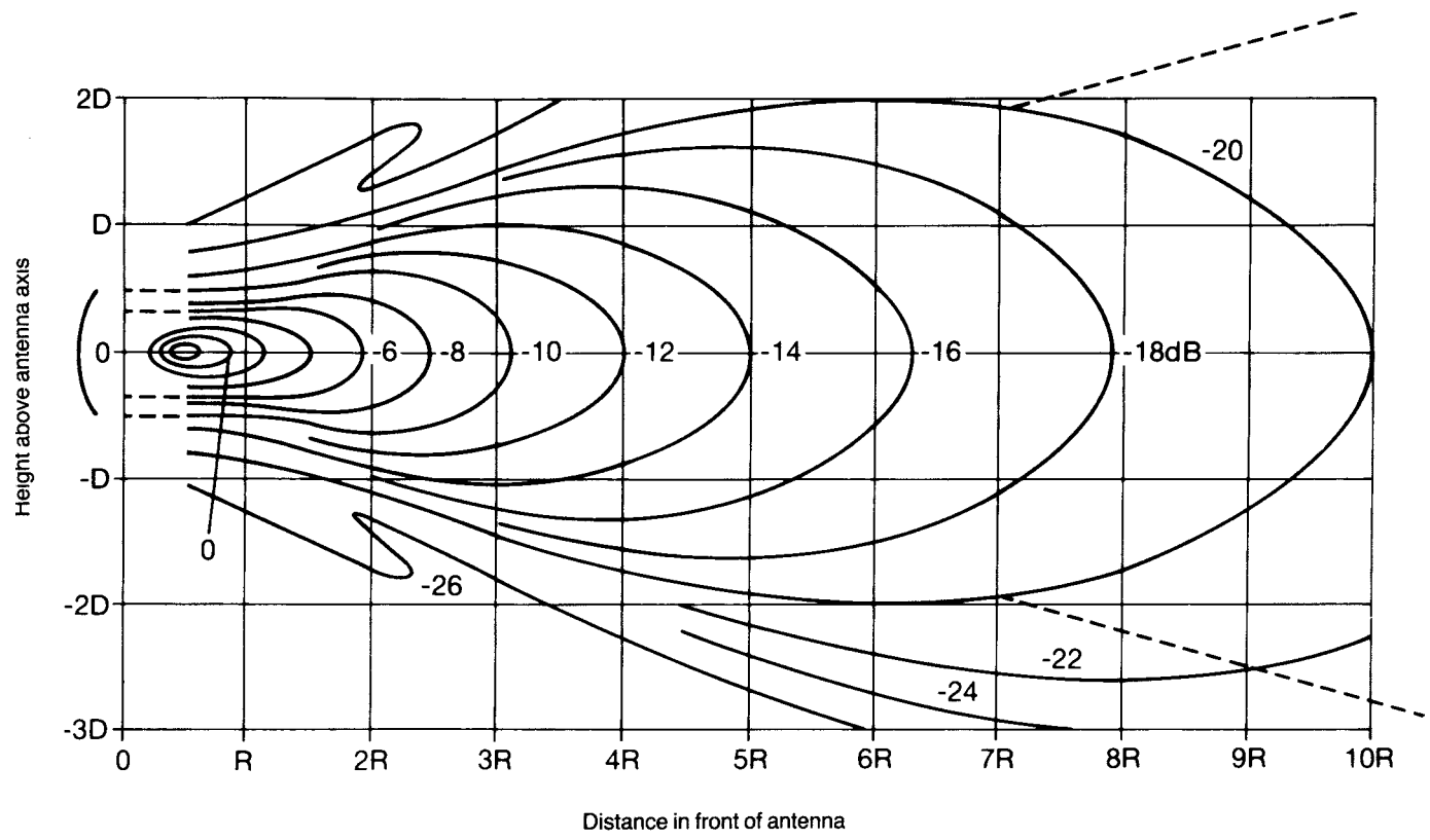
Figure 5.4 Far field of circular aperture antennas
