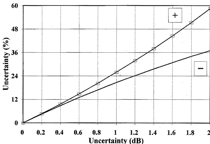
Figure 12.5 Uncertainties of measurement expressed in decibels and percentage for power density
