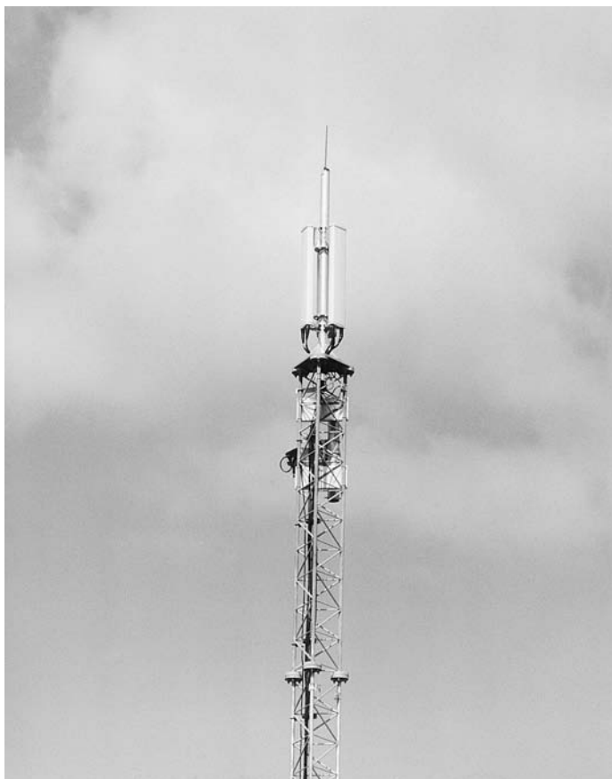
Figure 6.23 Narrow tower without separate ladder (Courtesy of E. Randall)
