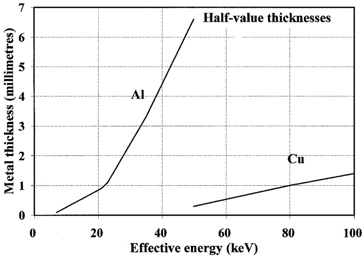
Figure 11.4 Half value layer thicknesses plotted from Table 10.1
