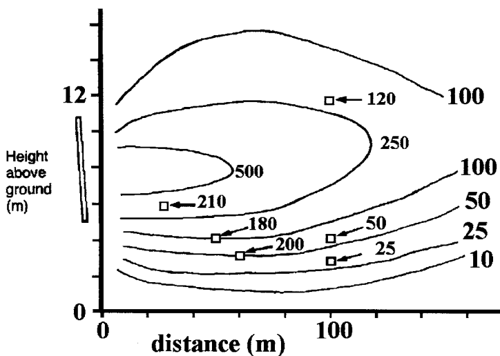
Figure 10.12 Use of elevated platform for special measurements
