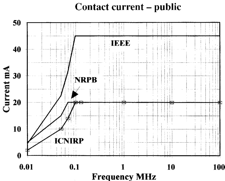
Figure 4.12 Contact current (public)
