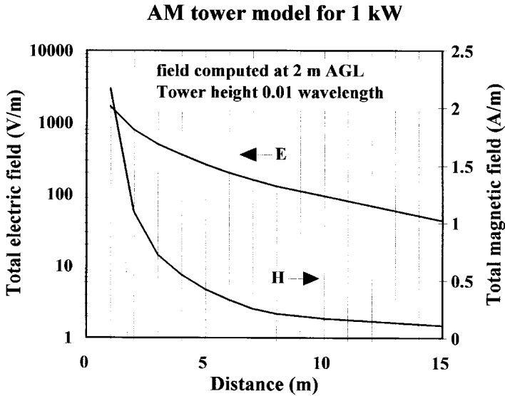
Figure 5.20 AM broadcast model for 1 kW, 0.01\lambda tower height
