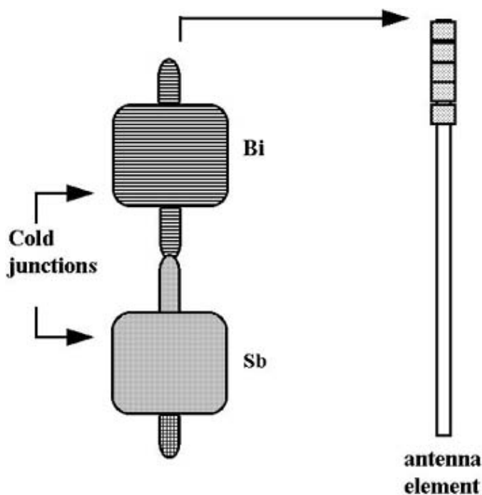
Figure 7.5 Typical thermocouple elements (Courtesy Narda Safety Test Systems)
