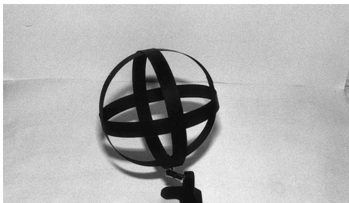
Figure 7.4 Sensor isotropic antennas – magnetic field
