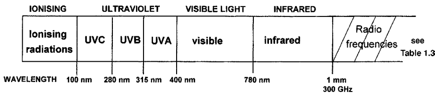
Figure 1.8 Radiation wavelengths relative to 300 GHz (WHO)
