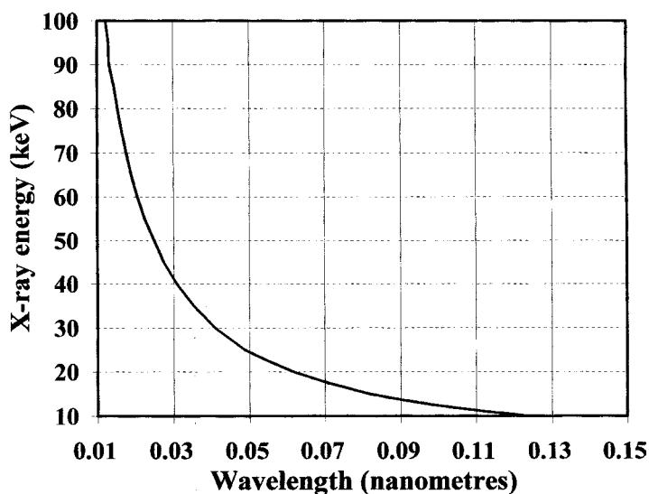
Figure 8.2 X-ray wavelength versus X-ray energy (keV)
