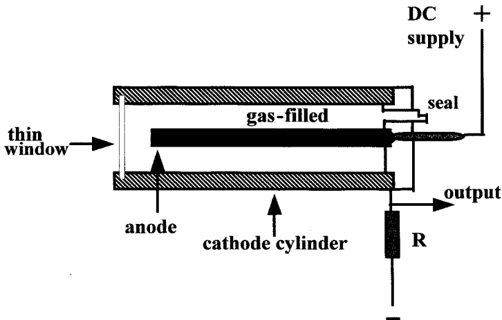
Figure 8.12 GM X-ray counter tube (Courtesy Philips Electronic tubes)
