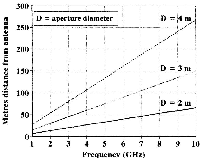
Figure 5.2 Rayleigh distance versus frequency for three circular aperture diameters
