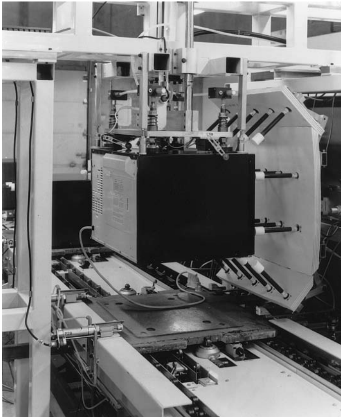
Figure 7.14 Holaday automated microwave oven test system (Courtesy Holaday Industries)
