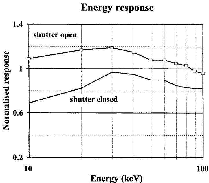
Figure 8.19 SmartION energy response curve (Courtesy Mini-Instruments Ltd)
