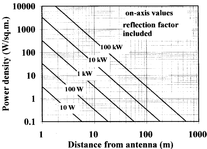
Figure 5.19 Transmission on-axis power densities for various power values
