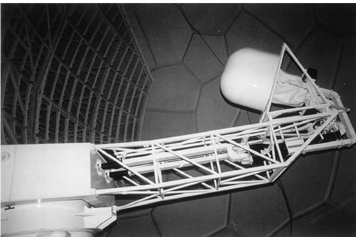
Figure 2.18 Inside ATC radome (Courtesy NATS)
