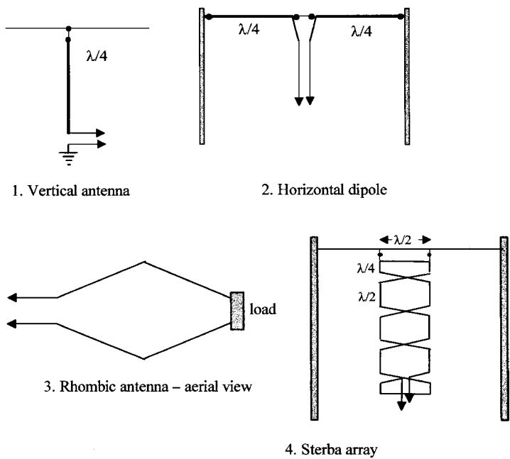
Figure 2.5 Simple HF antennas
