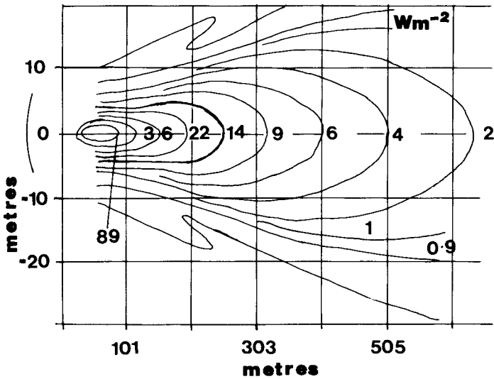
Figure 5.9 Calculated values for the far field in example 2 (values below 1 \text{ Wm}^{-2} not plotted)
