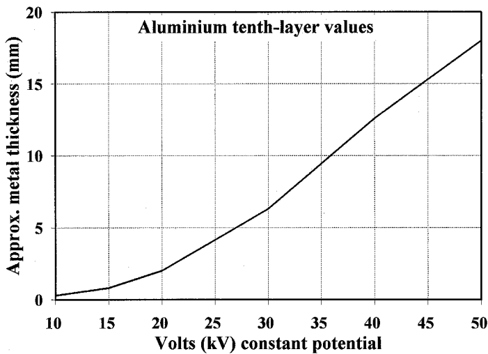
Figure 11.6 Tenth value layer thicknesses for aluminium shielding (Courtesy of BSI London)
