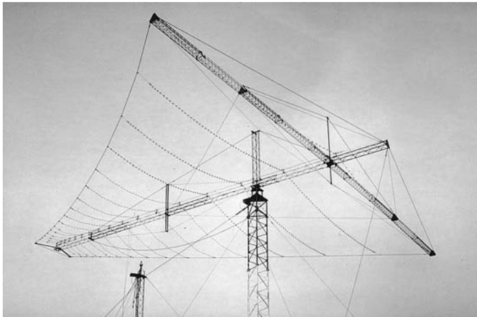
Figure 2.6 Horizontal log aperiodic (Courtesy Jaybeam Ltd)
