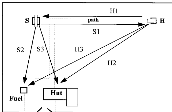
Figure 9.6 Site test alignments
