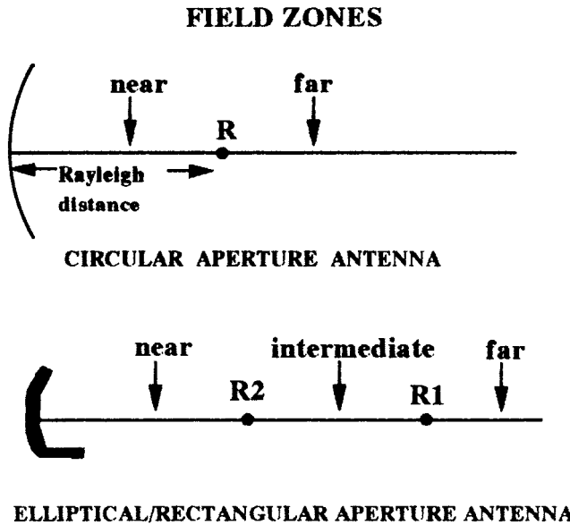
Figure 5.3 Radiation field zones of antennas
