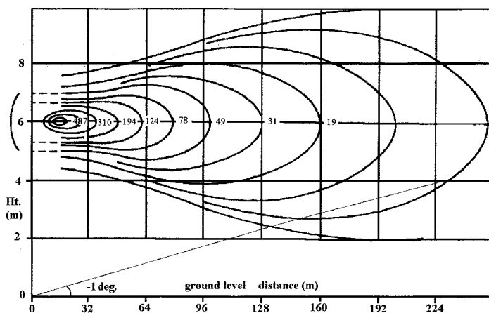
Figure 10.8 Change of beam elevation on calculation diagrams
