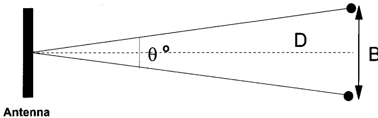
Figure 10.7 Beamwidth approximation by measurement
