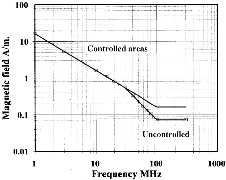
Figure 4.5 IEEE99 magnetic field
