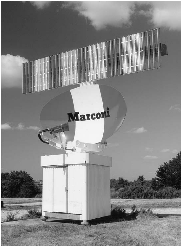
Figure 2.19 Surveillance radar with co-located Messenger SSR (Courtesy Alenia – Marconi)
