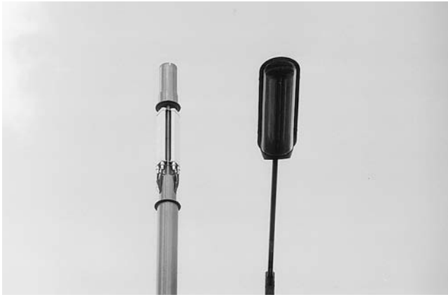
Figure 6.5 Concealed sector antennas – weather cover removed (Courtesy of E. Randall)
