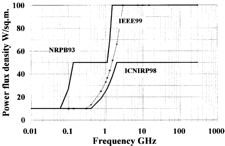
Figure 4.2 Comparison of power density limits for three standards (Occupational)
