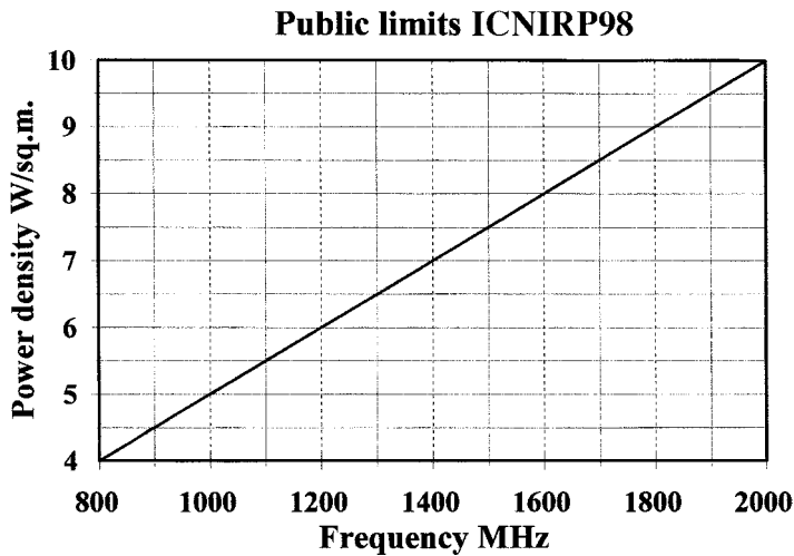
Figure 6.6 ICNIRP public limits over mobile phone frequencies
