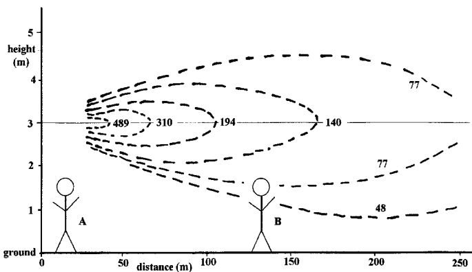
Figure 10.9 The danger of superficial assessments of safe distances with microwave beams
