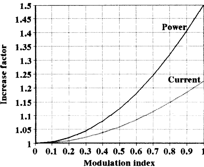
Figure 1.6 Sine wave amplitude modulation depth versus RF power and RF current
