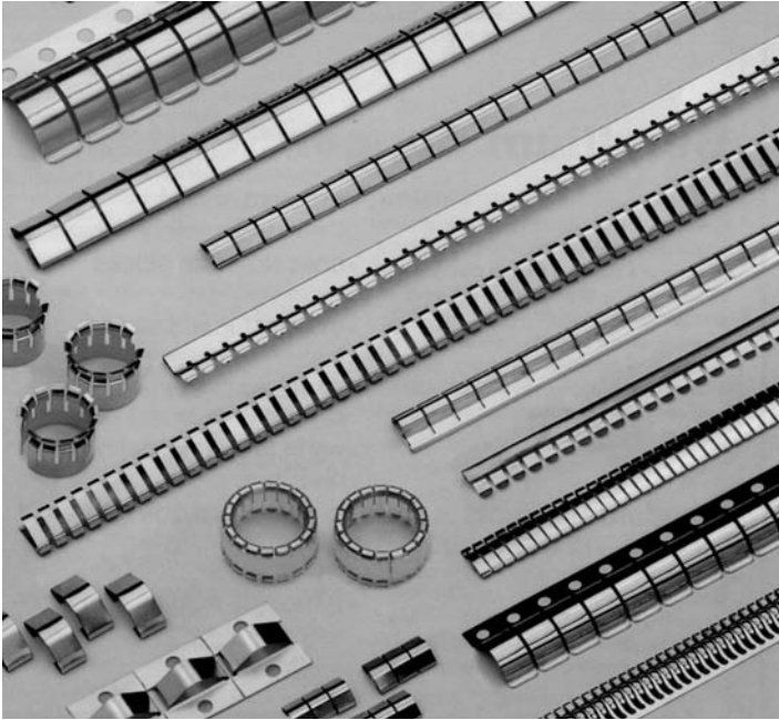
Figure 11.8 Selection of contact finger strips (Courtesy of TBA Electro Conductive Products)
