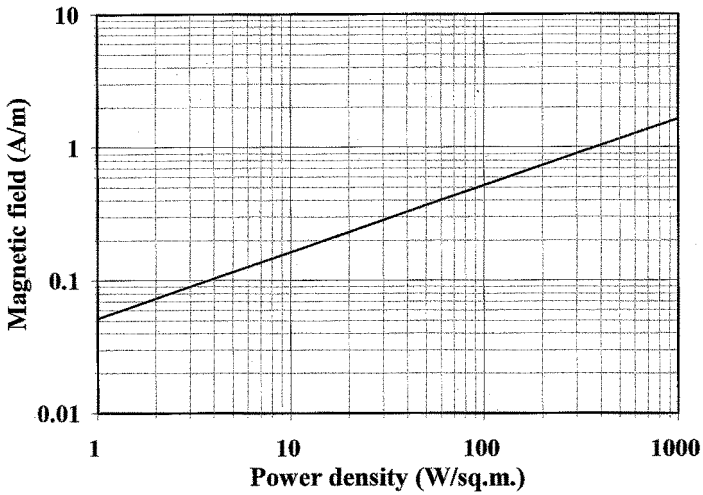
Figure A1.2 Power density values ( \text{Wm}^{-2} ) versus magnetic field plane wave values ( \text{Am}^{-1} )
