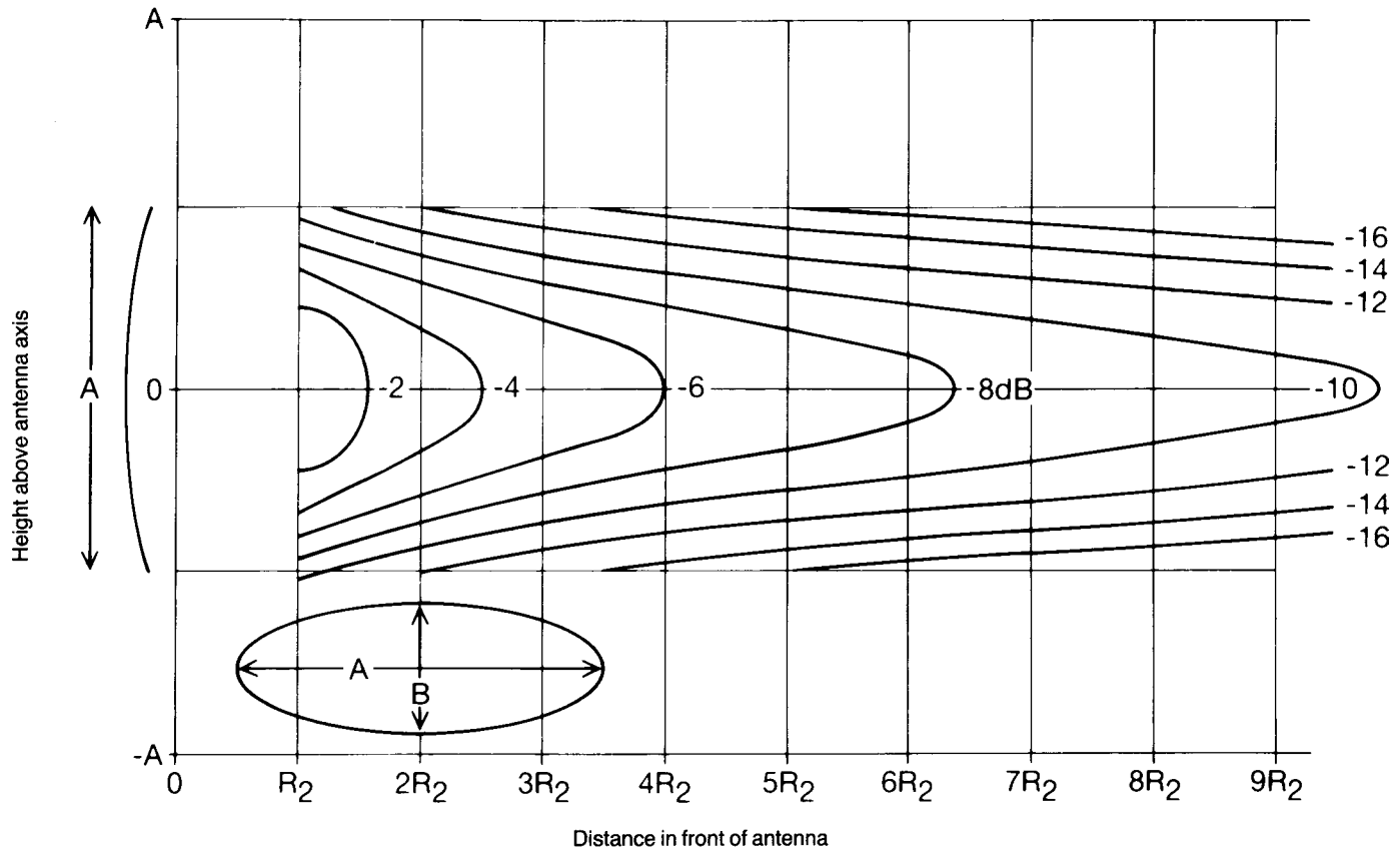
Figure 5.6 Elliptical and rectangular aperture antennas – intermediate field with larger aperture dimension vertical
