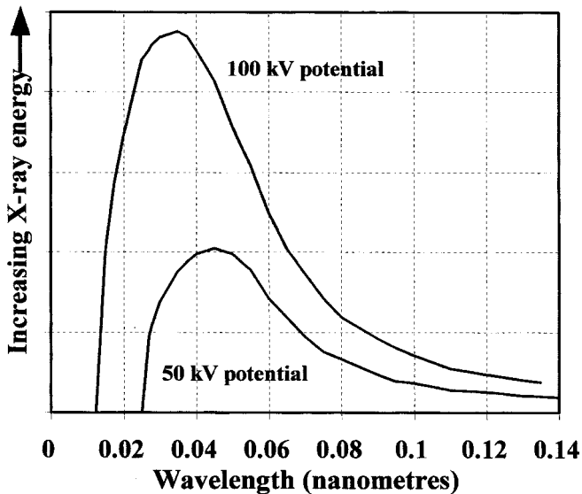
Figure 8.3 X-ray energy distribution versus tube voltage
