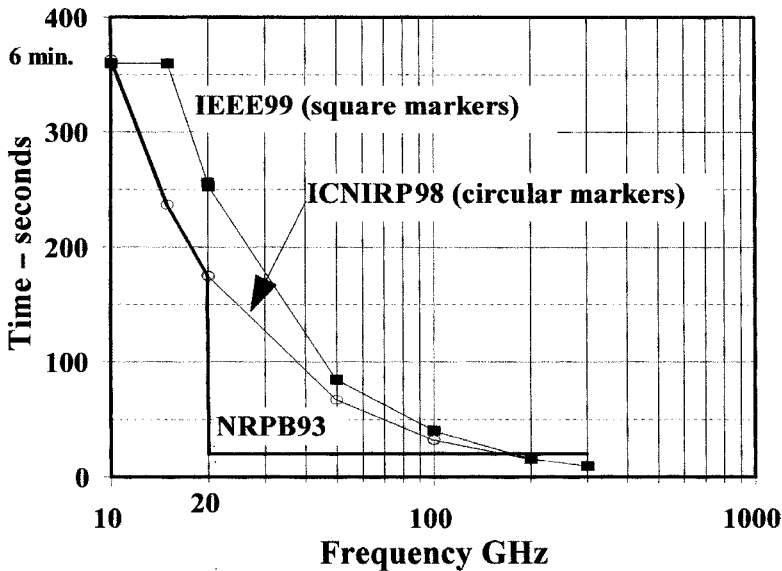
Figure 4.13 Time-averaging above 10 GHz
