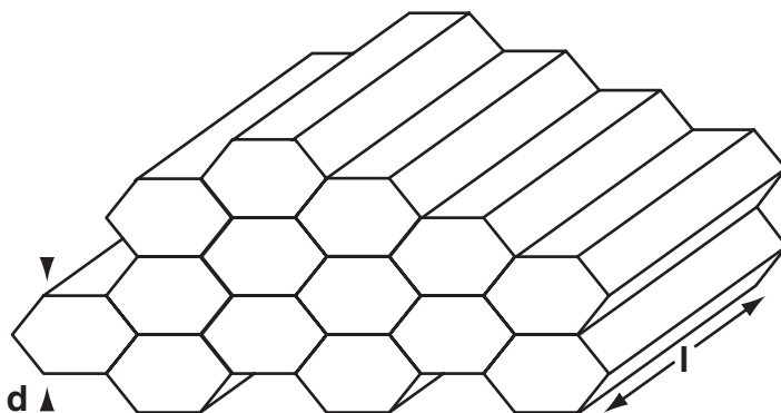
Figure 11.9 Honeycomb vent utilising waveguides below cut-off
