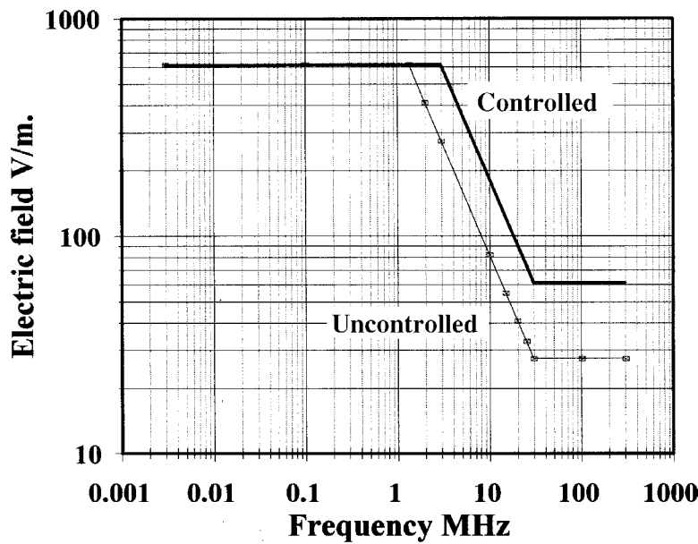
Figure 4.4 IEEE99 electric field
