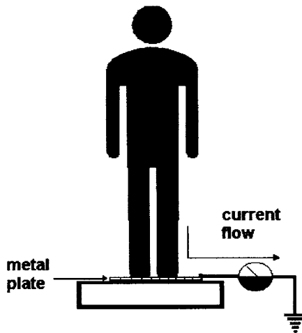
Figure 3.4 Limb current measurement concept
