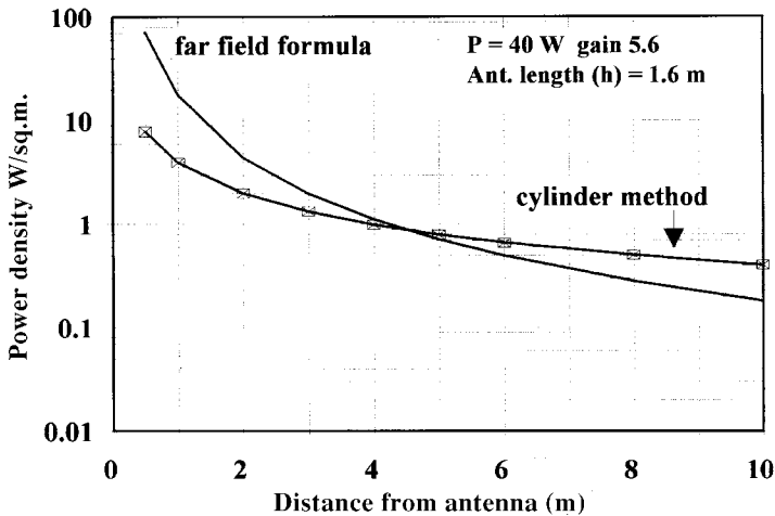
Figure 5.18 Comparison of 'cylinder' formula and the far field formula versus distance
