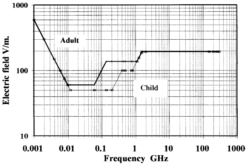
Figure 4.6 NRPB93 electric field
