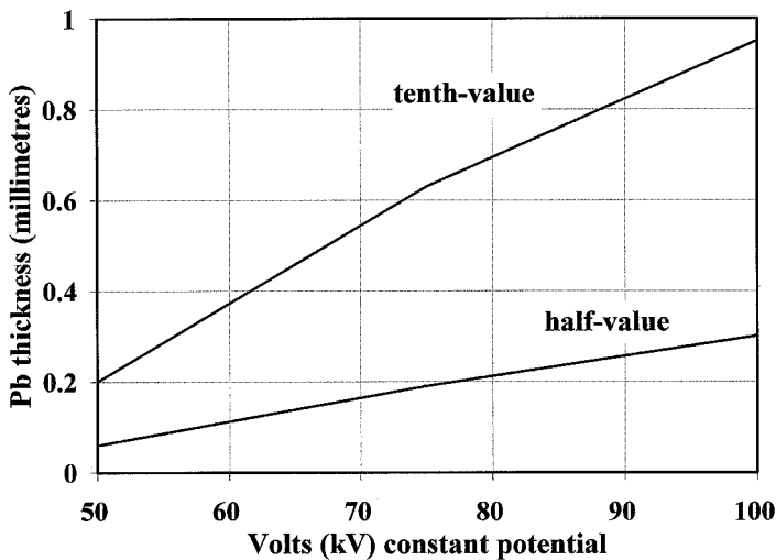
Figure 11.5 Half and one tenth value layer thickness for lead shielding (Courtesy of BSI London)
