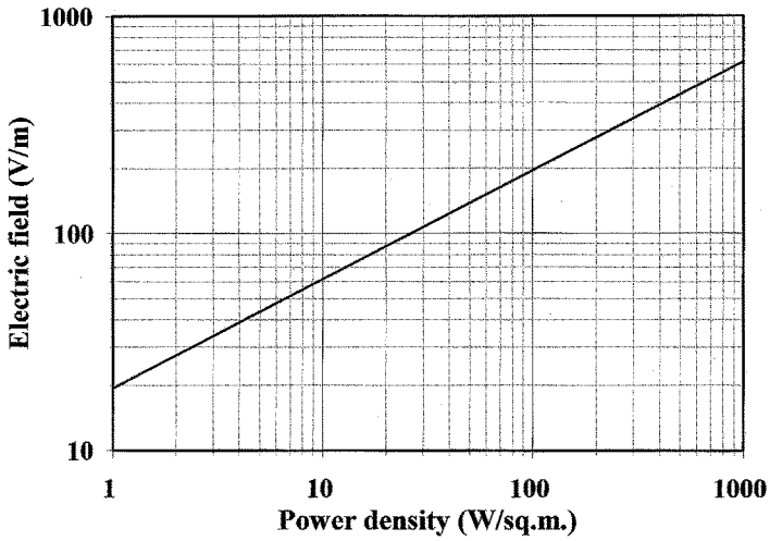
Figure A1.1 Power density values ( \text{Wm}^{-2} ) versus electric field plane wave values ( \text{Vm}^{-1} )
