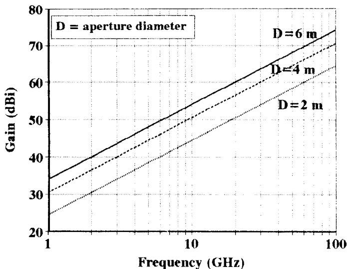
Figure 5.11 Gain of circular apertures versus frequency for three aperture diameters
