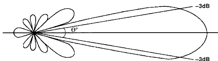
Figure 6.10 General beam characteristics
