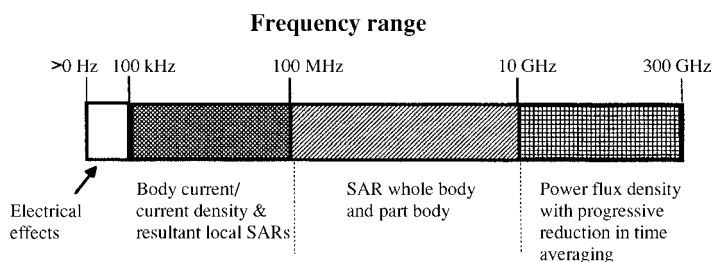
Figure 4.1 Outline of the criteria for deriving basic reference values
