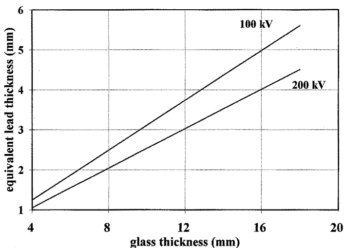
Figure 11.7 Curves for lead-glass shielding material (Courtesy of Pilkington Special Glass, Wales UK)
