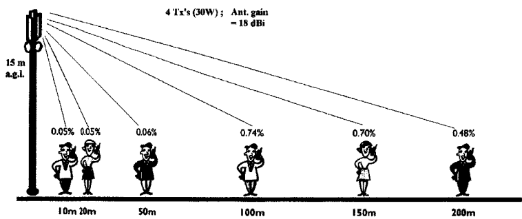
Figure 6.15 Measured levels from mast-mounted antennas as a percentage of a permitted level of 2 \text{ Wm}^{-2} (Courtesy of C&W Communications)
