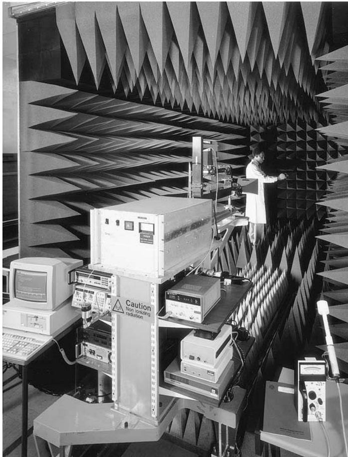
Figure 12.4 Anechoic chamber for calibration in the range 2.4 to 45.5 GHz (© Crown copyright 1998 reproduced by permission of the controller, HMSO)
