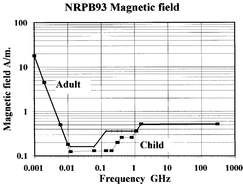
Figure 4.7 NRPB93 magnetic field
