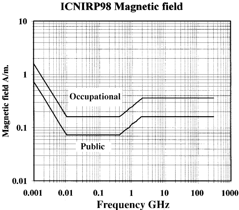
Figure 4.9 ICNIRP98 magnetic field
