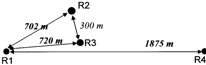
Figure 10.10 Typical airport radar layout in plan view
