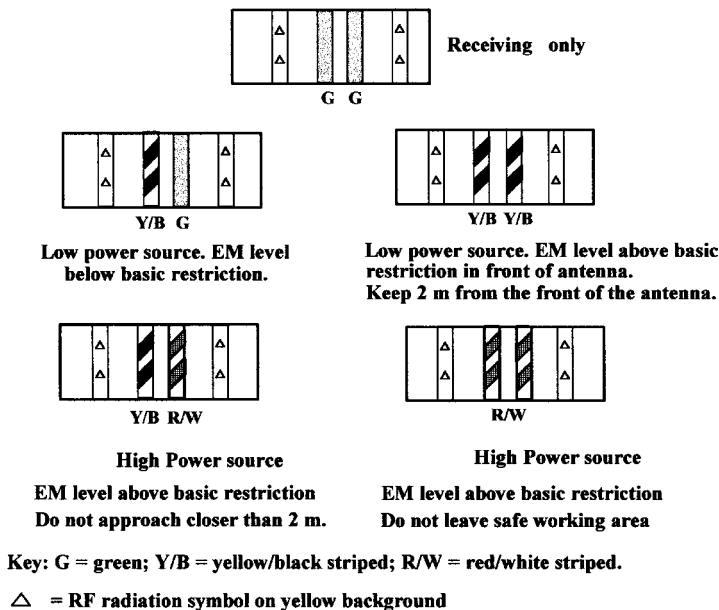
Figure 6.24 Experimental safety markings for rooftop and similar installations
