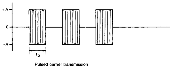
Figure 1.7 Pulse modulation
