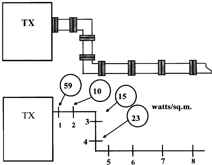
Figure 9.10 Leakage testing – waveguide runs
