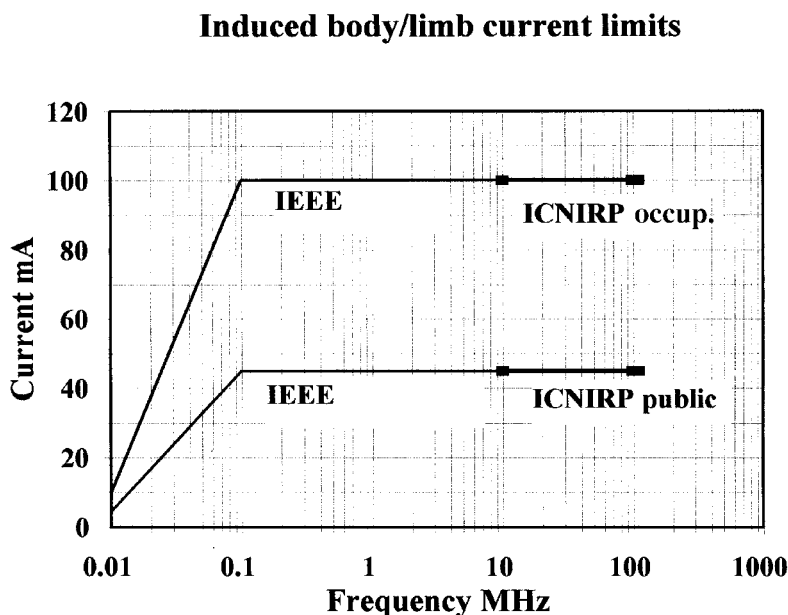
Figure 4.10 Induced body/limb currents
