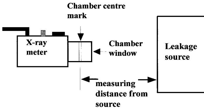
Figure 8.20 Measurement distance measurement for ionising chamber instruments
