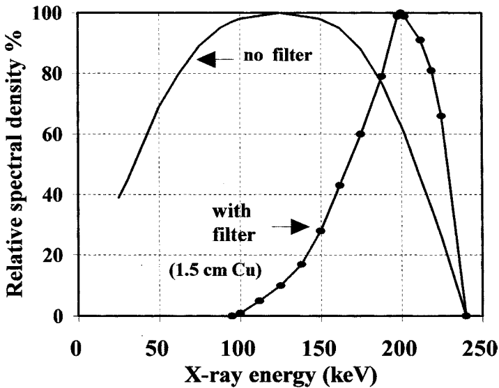
Figure 8.5 Klystron energy distribution (Courtesy Thomson Tubes Electronics)
