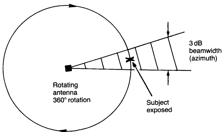
Figure 5.13 Rotating beam power density time-averaging for a subject in the intermediate/far field
