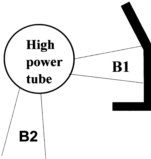
Figure 10.2 High power transmitter tube showing the possibility of X-ray beams appearing at angles outside a shield
