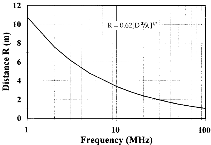
Figure 5.16 Plot of 0.62[D^3/\lambda]^{1/2} versus distance for 1 to 100 MHz
