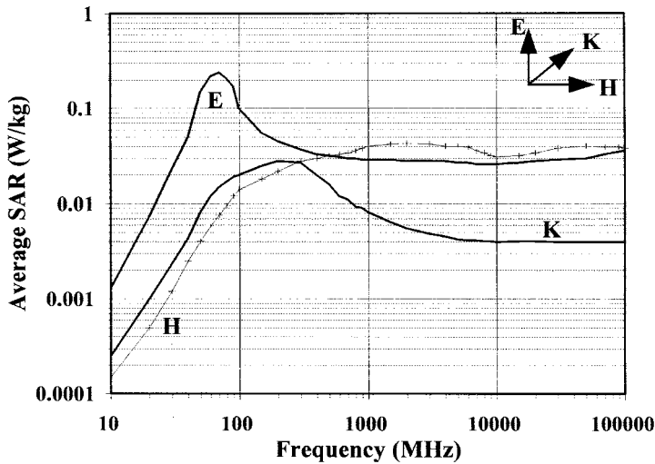
Figure 3.3 SAR versus frequency for orientations parallel to the E, H and K vectors (courtesy WHO – European Office)
