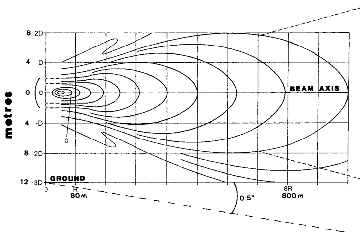
Figure 5.7 Portraying beam elevation-ground level relationships on antenna field charts
