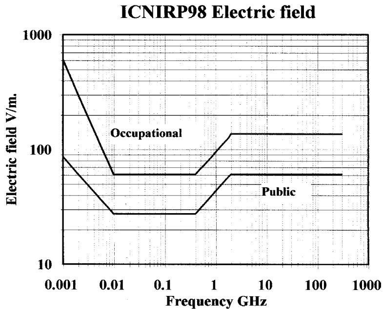
Figure 4.8 ICNIRP98 electric field
