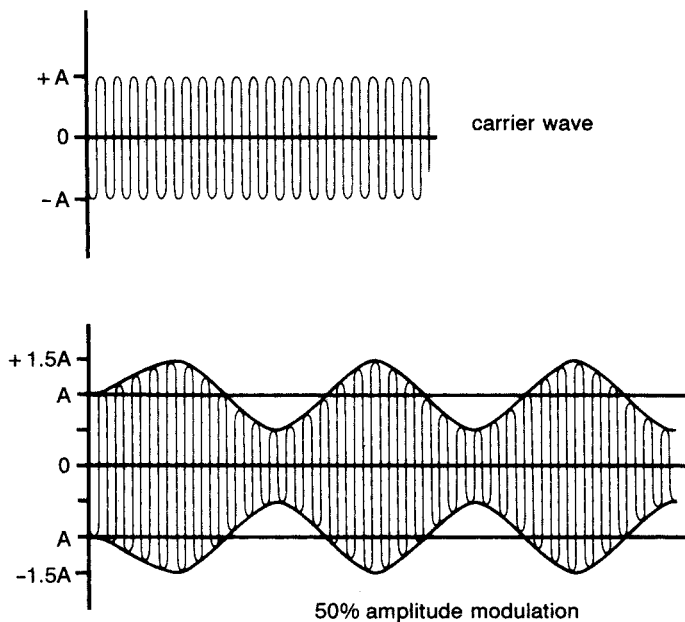
Figure 1.5 RF signal, amplitude modulated by a low frequency signal
