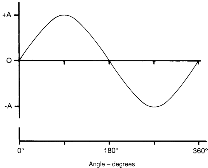
Figure 1.1 Sine wave illustration
