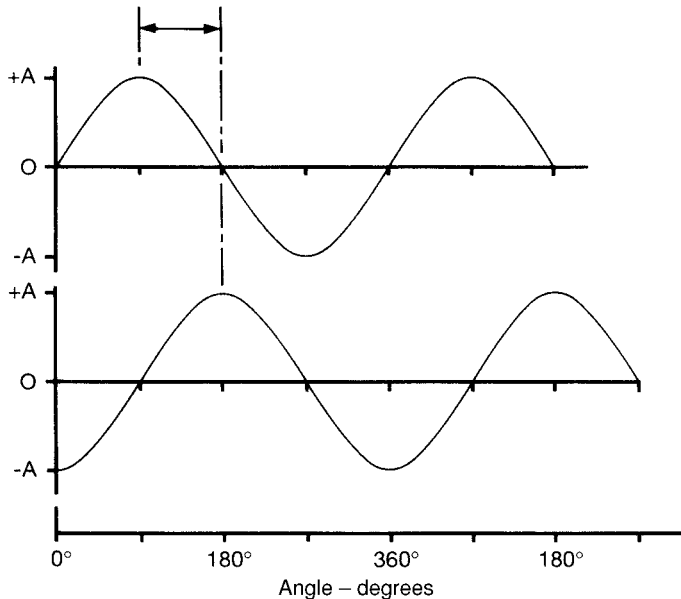
Figure 1.3 Phase difference between two waveforms
