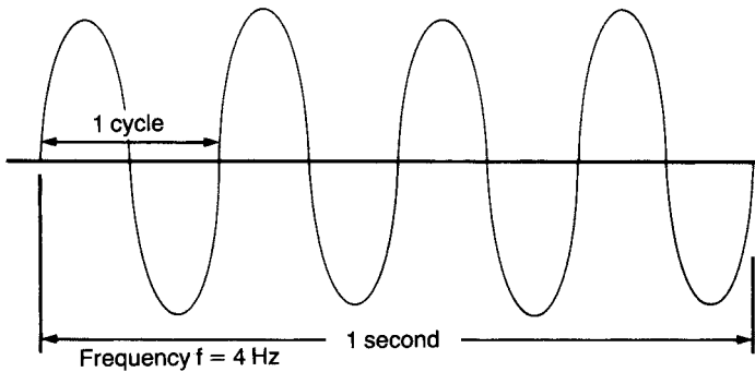
Figure 1.2 Sine wave frequency and time relationship
