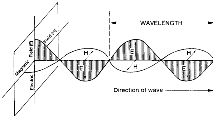
Figure 1.4 Representation of a plane wave
