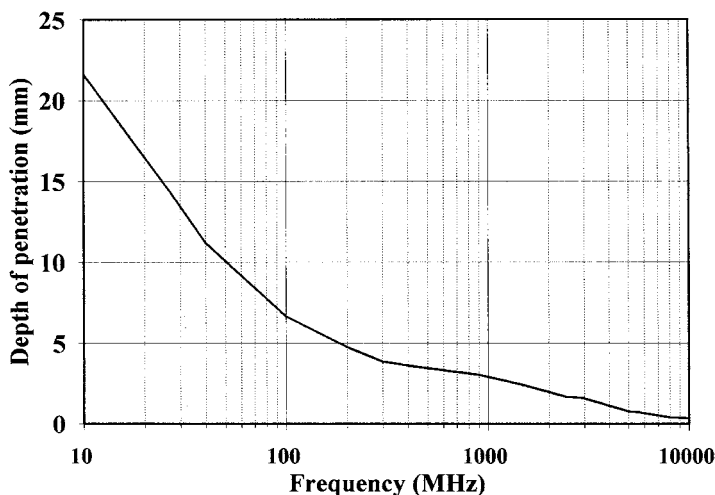
Figure 3.2 Depth of penetration of RF energy in tissues with high water content (data from reference 10)
