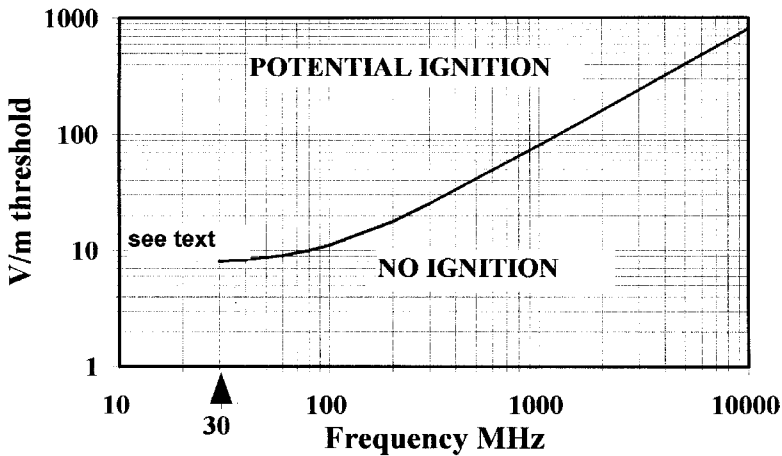
Figure 4.15 Safe thresholds gas group 2c – CW (single transmission)
