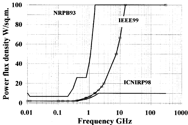
Figure 4.3 Comparison of power density limits for three standards (Public)
