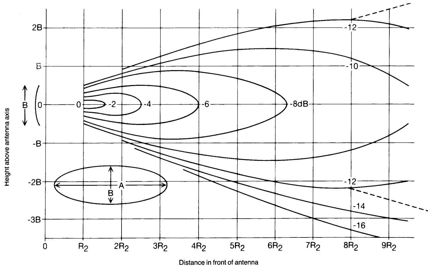
Figure 5.5 Elliptical and rectangular aperture antennas – intermediate field with larger aperture dimension horizontal
