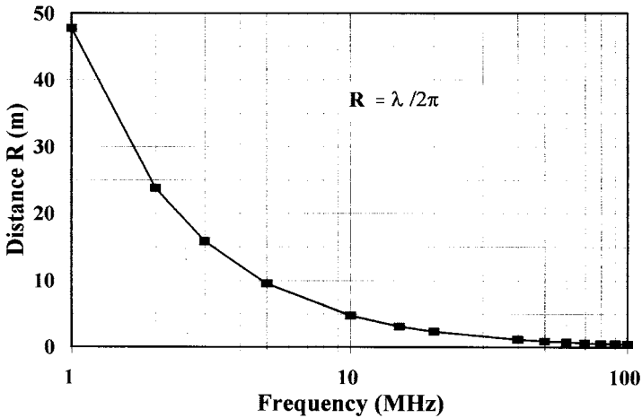
Figure 5.15 Plot of \lambda/2\pi versus distance for 1 to 100 MHz
