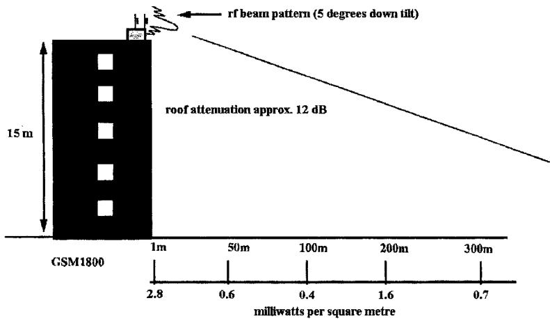
Figure 6.14 Theoretical levels for GSM(1800) exposure at ground level (Courtesy of C&W Communications)
