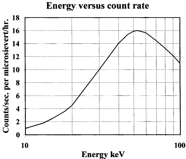
Figure 8.15 Mini-monitor type X energy–dose rate response (Courtesy Mini-instruments Ltd)
