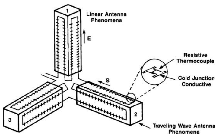
Figure 7.6 Diagrammatic illustration of a high frequency electric field sensor
