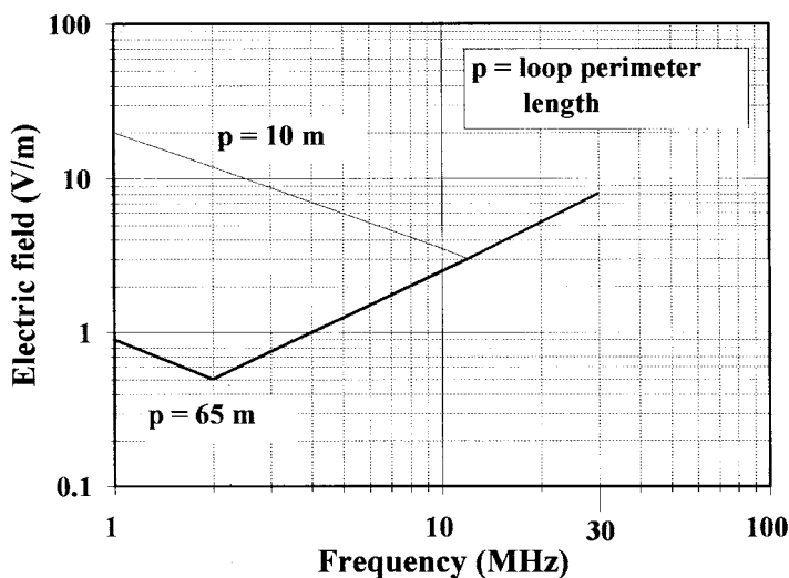
Figure 10.17 Field strength safety limits for the 1 to 30 MHz band calculated from BS6656:1991 for flammable vapours, gas group 2c
