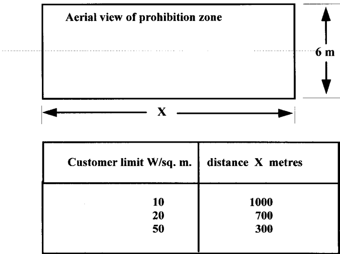
Figure 10.14 Mobile equipment prohibited areas
