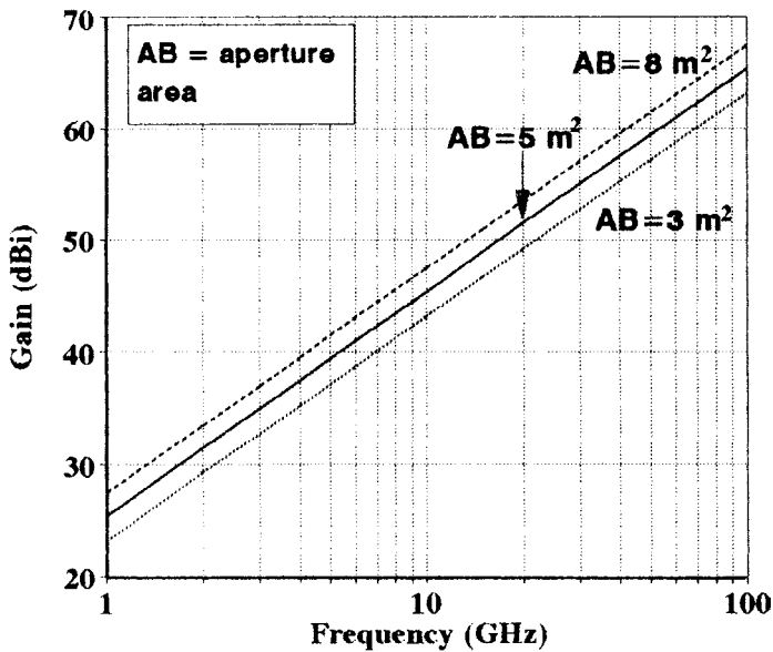
Figure 5.12 Gain of elliptical and rectangular apertures versus frequency for three values of the product A \times B
