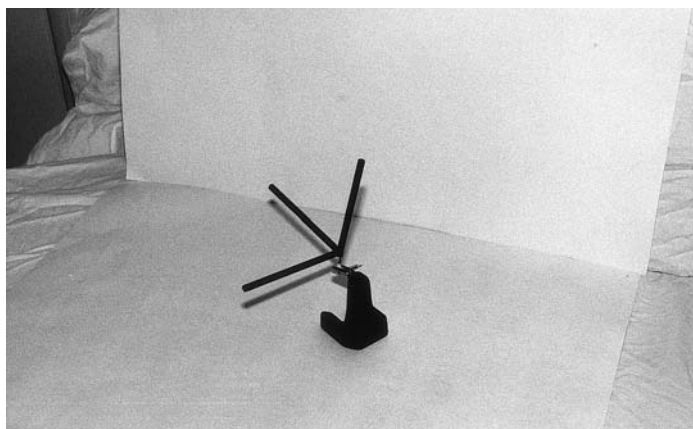
Figure 7.3 Sensor isotropic antennas – electric field
