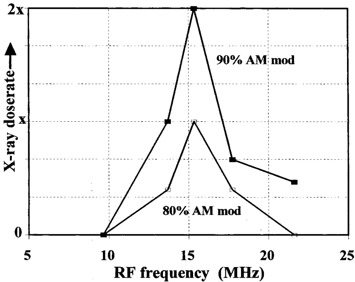
Figure 8.7 High power HF broadcast transmitter X-ray leakage investigation
