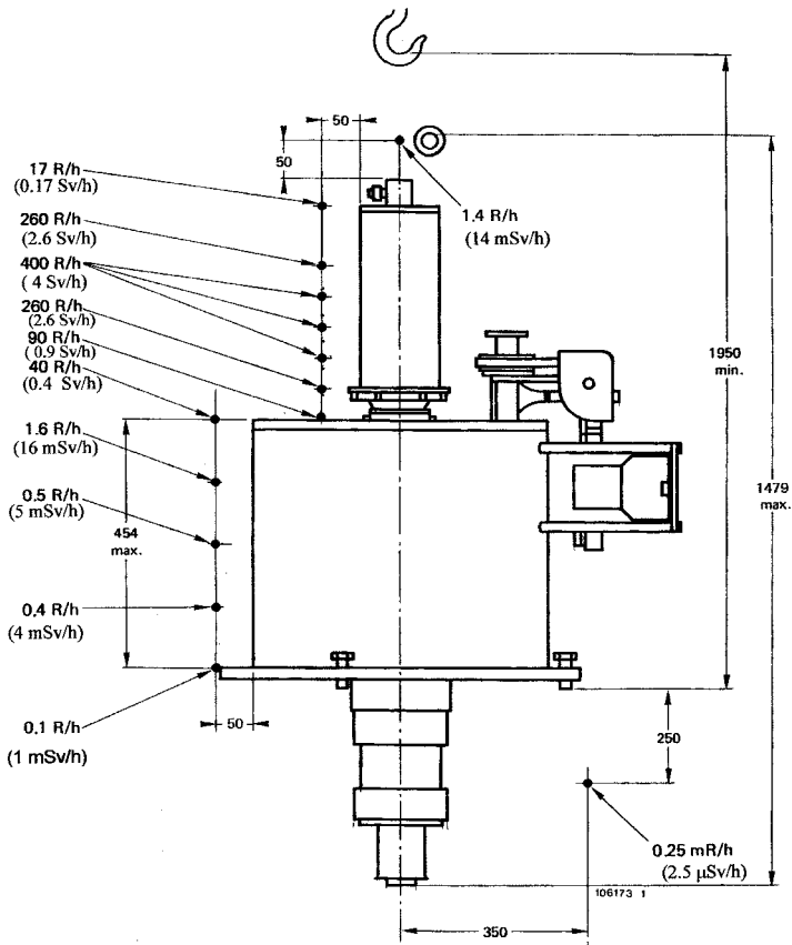
Figure 8.4 Klystron X-ray test results (Courtesy Thomson Tubes Electroniques)
