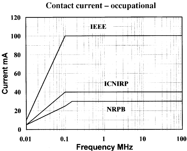
Figure 4.11 Contact current (occupational)
