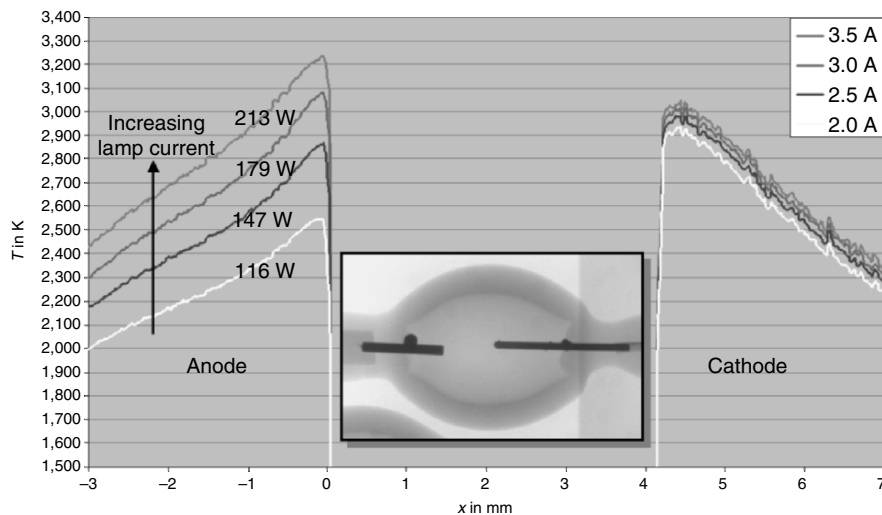
Fig. 3.25. One-dimensional temperature plot of a dc high-pressure mercury lamp at four different lamp currents (2–3.5 A) using (2+1)-\lambda pyrometry. An X-ray photograph visualizing the lamp under investigation is shown between the temperature profiles of anode and cathode ([9, 128], mercury pressure: 2 MPa, electrode distance: 4.23 mm)
