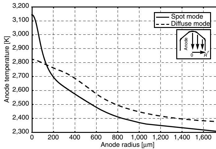
Fig. 4.102. Calculated anode temperature distribution vs. anode radius for spot and diffuse arc attachments on anode (ApolloHg-lamp, Hg, p = 4 MPa, I = 4 A (dc), d_{\text{electrode}} = 2 mm, \varphi_{\text{emission}} = \varphi_{\text{cool/heat}} = 4.55 eV)
