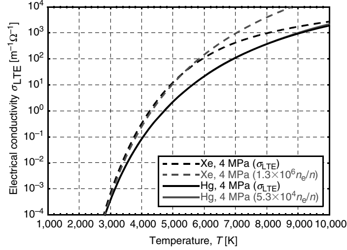
Fig. 4.18. LTE electrical conductivity \sigma_{\text{LTE}} compared to the ratio n_{e,\text{LTE}}/n for a 4 MPa xenon or mercury plasma vs. plasma temperature
