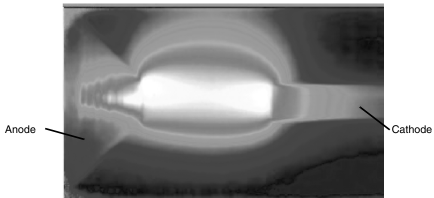
Fig. 4.89. Measured radiation intensity (ApolloHg-lamp, plasma and electrodes, [9, 128])
