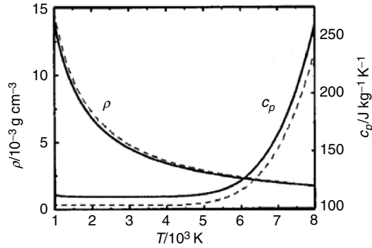
Fig. 4.42. Comparison of plasma properties: Mass density \rho and specific heat at constant pressure c_p vs. plasma temperature for mercury, 0.6 MPa taken from [102] ( solid lines ) and calculated according to Sect. 2.3 and [171] ( dashed lines )
