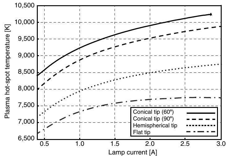
Fig. 4.50. Calculated plasma hot-spot temperature near cathode tip vs. dc lamp current I for different electrode geometries (LS9hg-lamp, Hg, p = 0.6 MPa, \phi = 4.55 eV, electrode diameter/length 0.7 mm/10 mm, [57])
