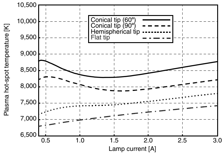
Fig. 4.51. Calculated plasma hot-spot temperature near anode tip vs. dc lamp current I for different electrode geometries (LS9hg-lamp, Hg, p = 0.6 MPa, \phi = 4.55 eV, electrode diameter/length 0.7 mm/10 mm, [57])
