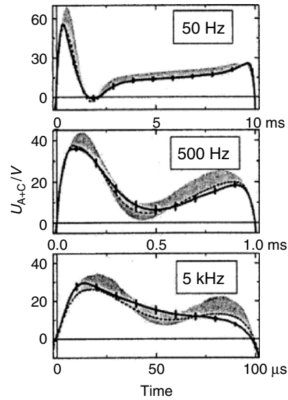
Fig. 3.44. Electrode fall voltages ( solid line ) vs. time obtained from the extrapolation of the lines shown in Fig. 3.42 to zero electrode gap. The dashed line corresponds to the total lamp voltage of the 28 mm lamp minus a calculated electric field in the plasma column according to a model described in [102] times the electrode gap, the shaded band corresponds to the same for all other lamps with larger electrode gaps
