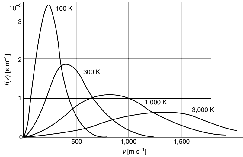
Fig. 2.3. Maxwell probability distribution for the velocity of \text{N}_2 molecules (air) for four different temperatures [72]
