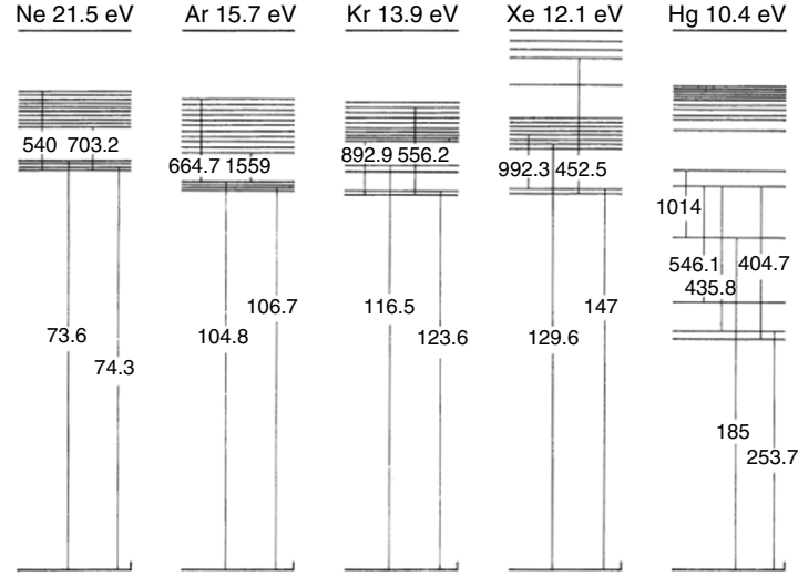
Fig. 2.11. Energy level diagram of rare gas atoms compared to mercury atom. The ionization energies are drawn at the same height, the numbers at the lines connecting different energy levels are the corresponding photon wavelengths in nm for a radiative transition (excitation or de-excitation) [48]
