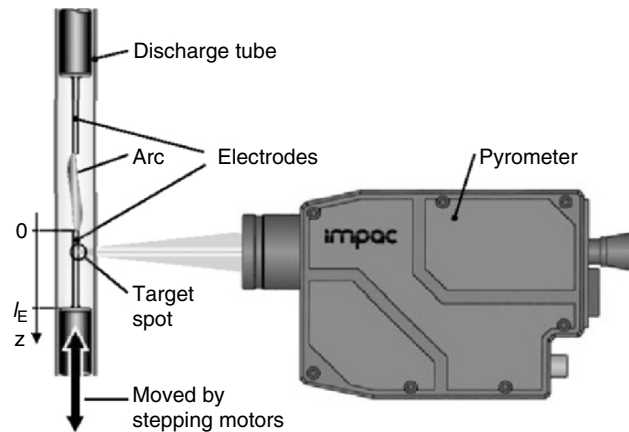
Fig. 3.5. Experimental setup for 1- \lambda pyrometry used in [43, 121, 123]. The electrodes are moved along the target spot of the pyrometer
