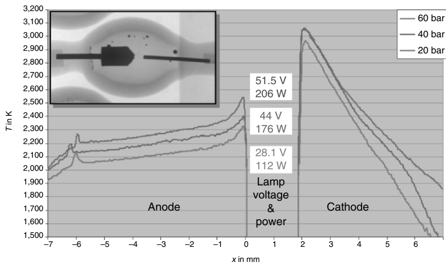
Fig. 3.24. One-dimensional temperature plot of three different dc high-pressure mercury lamps with different mercury pressures (2, 4, and 6 MPa) using (2+1)-\lambda pyrometry. An X-ray photograph of the lamp under investigation is shown in the top left-hand corner. The lamp voltage and lamp power corresponding to the three temperature curves are given between the temperature profiles of anode and cathode [9, 128], electrode distance: 2 mm, current: 4 A)
