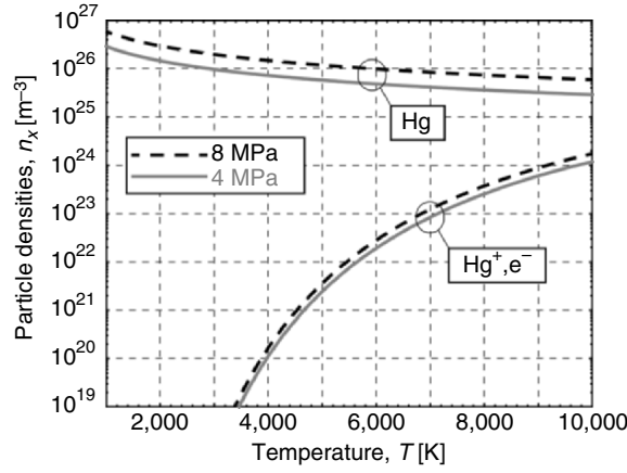
Fig. 2.6. Particle densities of Hg, \text{Hg}^+ , and e^- ( n_i = n_e ) calculated using the Saha equation for a 4 and 8 MPa mercury plasma vs. plasma temperature [171]
