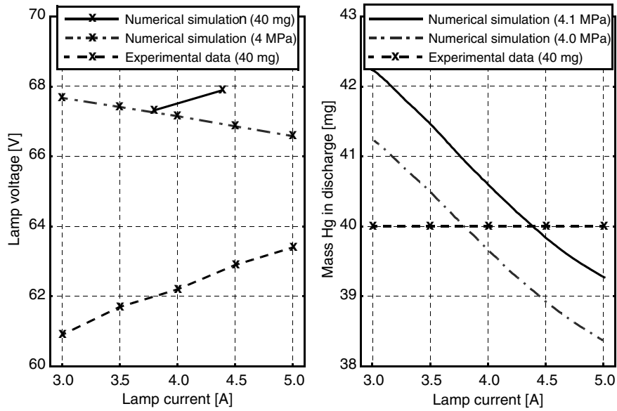
Fig. 4.91. Calculated and measured lamp voltage (left-hand side) and calculated mercury mass in the discharge (right-hand side) vs. lamp current (ApolloHg-lamp, Hg, p = 4.0 or 4.1 MPa, I = 3\text{--}5 A (dc), d_{\text{electrode}} = 3 mm, \varphi_{\text{emission}} = \varphi_{\text{cool/heat}} = 4.55 eV, [62])
