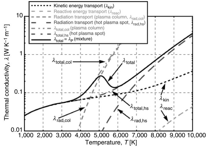
Fig. 2.26. Thermal conductivity \lambda (and components) of a D2 automotive headlight lamp plasma (Xe, Hg, NaI, and \text{ScI}_3 with partial pressures of 50, 20, 0.03, and 0.05 bar, respectively) vs. plasma temperature [59]
