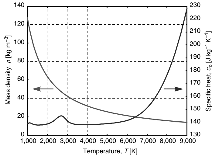
Fig. 4.76. Mass density \rho (left axis) and specific heat at constant pressure c_p (right axis) for a D2 lamp plasma (Xe, Hg, NaI, ScI 3 ) vs. plasma temperature [59]
