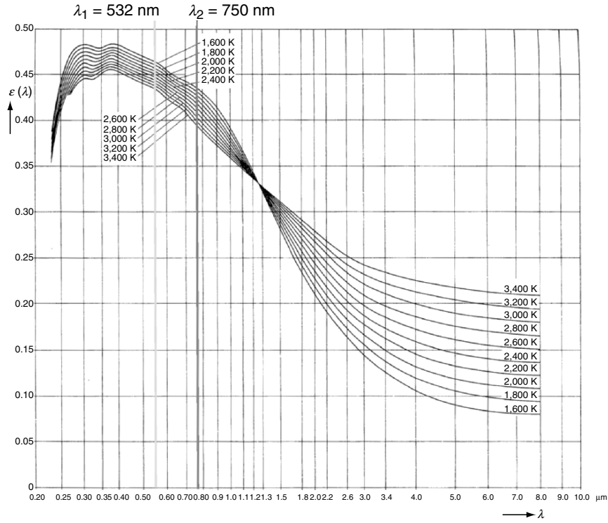
Fig. 3.8. Spectral emissivity \varepsilon(\lambda, T) of tungsten vs. wavelength \lambda for several temperatures superimposed by two wavelengths \lambda_1 and \lambda_2 selected with the help of optical interference filters for 2- \lambda pyrometry [48]
