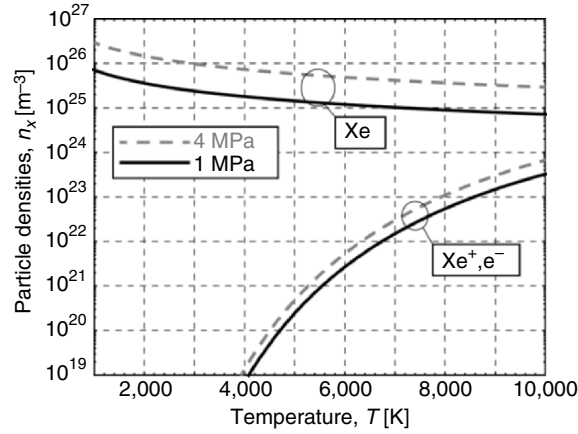
Fig. 2.7. Particle densities of Xe, \text{Xe}^+ , and e^- ( n_i = n_e ) calculated using the Saha equation for a 1 and 4 MPa xenon plasma vs. plasma temperature [171]
