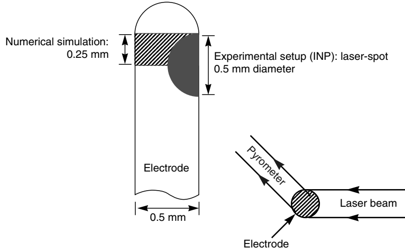
Fig. 4.57. Laser heating areas on the electrode surface in the experimental setup and for the numerical simulations with the self-consistent electrode-plasma model
