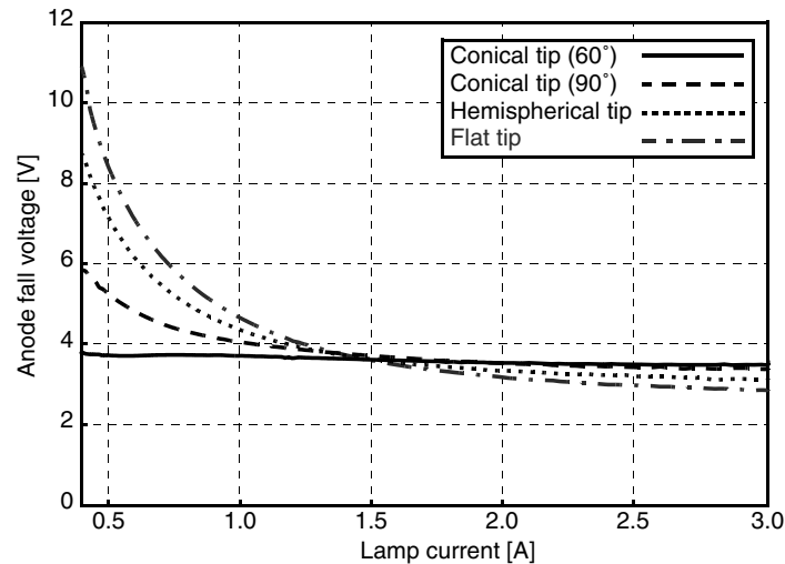
Fig. 4.54. Calculated anode fall voltage vs. dc lamp current I for different electrode geometries (LS9hg-lamp, Hg, p = 0.6 MPa, \phi = 4.55 eV, electrode diameter/length 0.7 mm/10 mm, [57])
