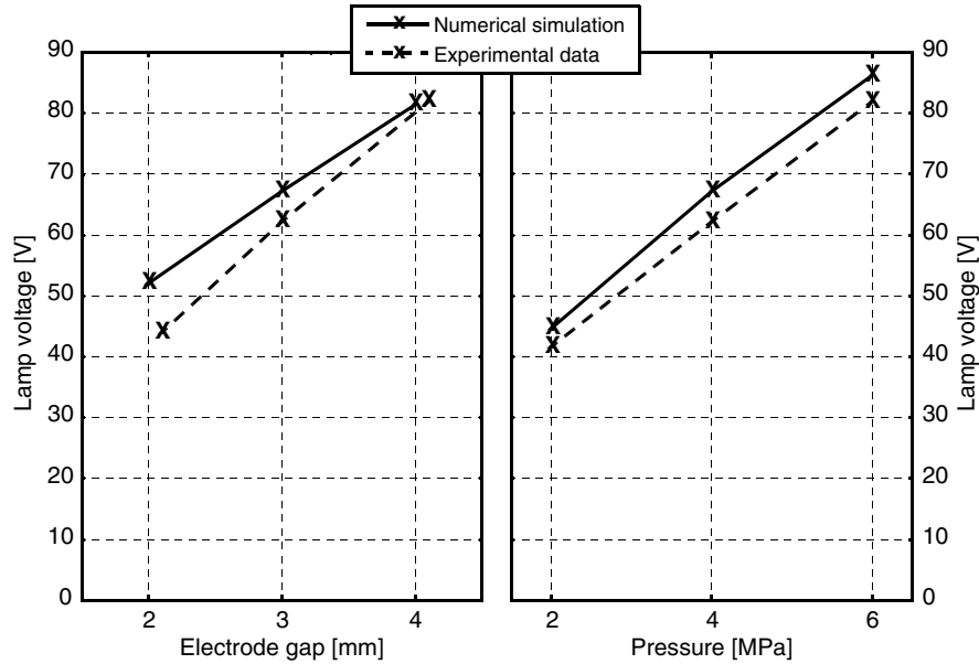
Fig. 4.92. Calculated and measured lamp voltage vs electrode gap (left-hand side) and vs. pressure (right-hand side) (ApolloHg-lamp, Hg, p = 2, 4 , or 6 MPa, I = 4 A (dc), d_{\text{electrode}} = 2, 3 , or 4 mm, \varphi_{\text{emission}} = \varphi_{\text{cool/heat}} = 4.55 eV, [62])
