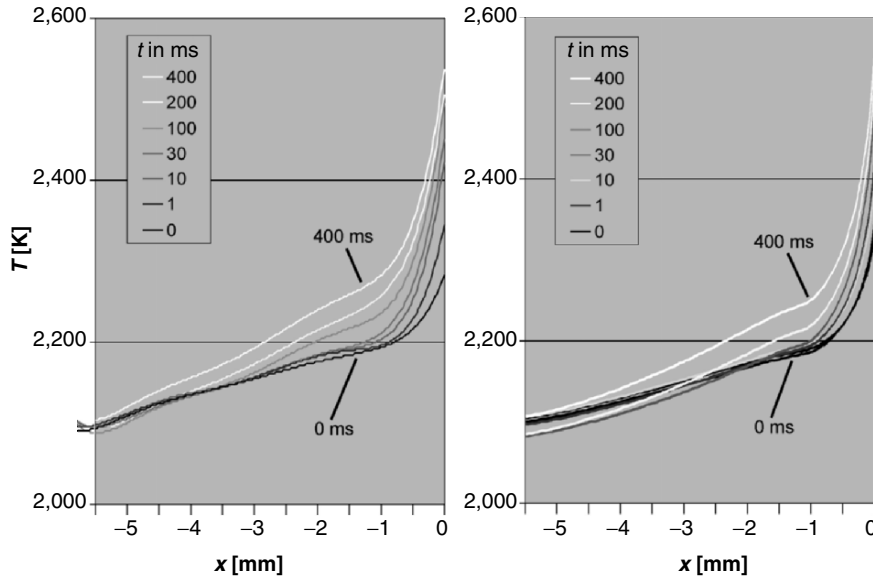
Fig. 4.105. Calculated (right-hand side) and measured (left-hand side) anode temperature distribution at certain points in time after a lamp current jump from 2.5 to 6 A at t = 0 (ApolloHg-lamp, Hg, p = 2 MPa, d_{\text{electrode}} = 3 mm, \phi_{\text{emission}} = 3.5 eV, \phi_{\text{cool/heat}} = 4.55 eV, [128])
