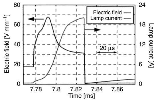
Fig. 4.10. Lamp current and electric field in the plasma column vs. time during and after the current pulse (Hg, 6 MPa, [160])
