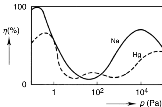
Fig. 1.12. Relative luminous efficacies of sodium and mercury discharge lamps depending on vapor pressure of sodium and mercury, respectively. In the case of the mercury discharge, the use of a fluorescent powder to convert UV radiation into visible light is assumed [118]
