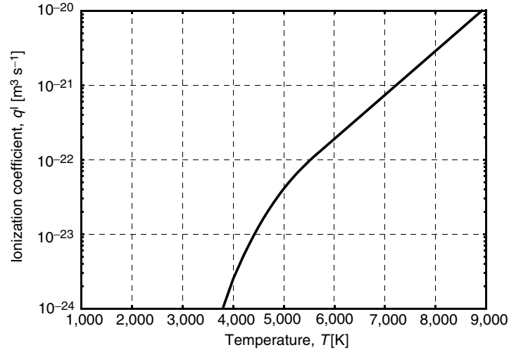
Fig. 4.23. Rate coefficient for ionization q^I for a D2 lamp plasma (Xe, Hg, NaI, \text{ScI}_3 ) vs. plasma temperature
