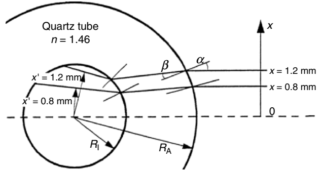
Fig. 3.38. Deflection of line-of-sight due to the refraction at the arc tube (here: the quartz vessel of a D2 automotive headlight lamp, R_I = 1.35 mm, R_A = 3 mm [132]). The electrodes are located above and below the drawing plane
