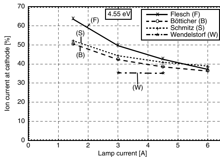
Fig. 4.35. Ratio of ion to total lamp current at the cathode vs. dc lamp current (LS8-lamp, Xe, p = 1 MPa, \varphi = 4.55 eV, [56])
