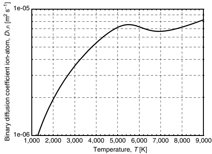
Fig. 4.77. Binary diffusion coefficient between ions and atoms D_{i,n} for a D2 lamp plasma (Xe, Hg, NaI, ScI 3 ) vs. plasma temperature [59]
