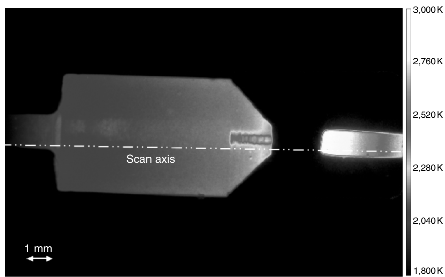
Fig. 3.23. Temperature distribution of anode (left-hand side) and cathode (right-hand side) of the mercury high-pressure discharge lamp shown in Fig. 3.21 using (2+1)-\lambda pyrometry. The scan axis for the determination of a one-dimensional temperature plot avoids the problems due to reflections of the radiation coming from the cathode [9, 128], mercury pressure: 2 MPa, electrode distance: 2 mm, current: 4 A)
