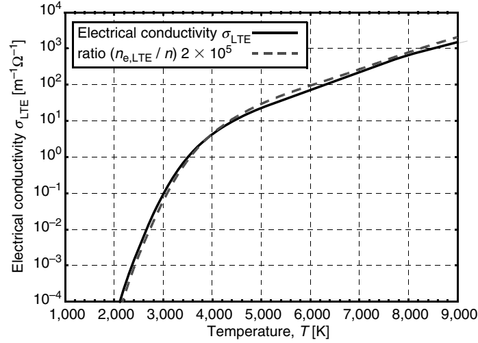
Fig. 4.20. LTE electrical conductivity \sigma_{\text{LTE}} compared to the ratio n_{\text{e,LTE}}/n \cdot 2 \times 10^5 \text{ m}^{-1} \Omega^{-1} for a D2 lamp plasma (Xe, Hg, NaI, ScI 3 ) vs. plasma temperature [59]
