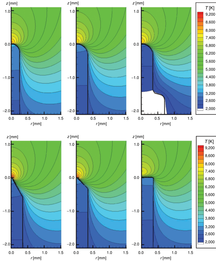
Fig. 4.47. Calculated plasma and cathode temperature for different electrode geometries (LS9hg-lamp, Hg, p = 0.6 MPa, I = 1.0 A (dc), \phi = 4.55 eV, electrode length: 10 mm, [57])
