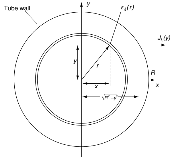
Fig. 3.39. Illustration of the inverse Abel transformation of the measured line-of-sight radiation intensity J_\lambda(y) to get the wanted emission density \epsilon_\lambda(r) per steradian at wavelength \lambda . The electrodes are located above and below the drawing plane at x = y = 0
