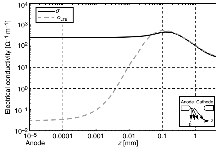
Fig. 4.66. Calculated electrical conductivity (LTE and non-LTE, double logarithmic scale) on lamp axis near anode (LS9hg-lamp, Hg, p = 0.6 MPa, I = 1.8 A (dc), \phi = 4.55 eV, hemispherical tip, electrode diameter/length 0.5 mm/13 mm)
