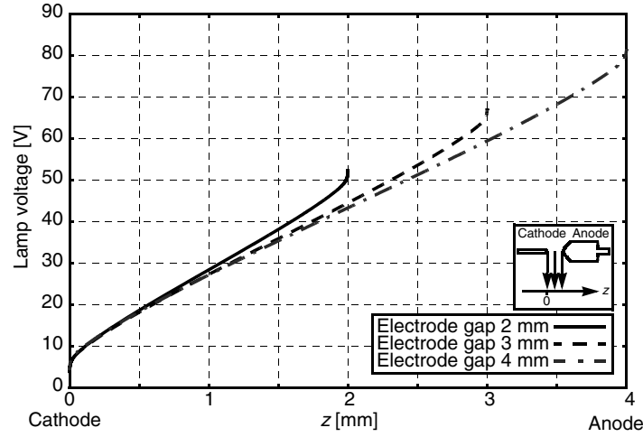
Fig. 4.90. Calculated electric potential on lamp axis (ApolloHg-lamp, Hg, p = 4 MPa, I = 4 A (dc), d_{\text{electrode}} = 2, 3 , or 4 mm, \phi_{\text{emission}} = \phi_{\text{cool/heat}} = 4.55 eV, [62])
