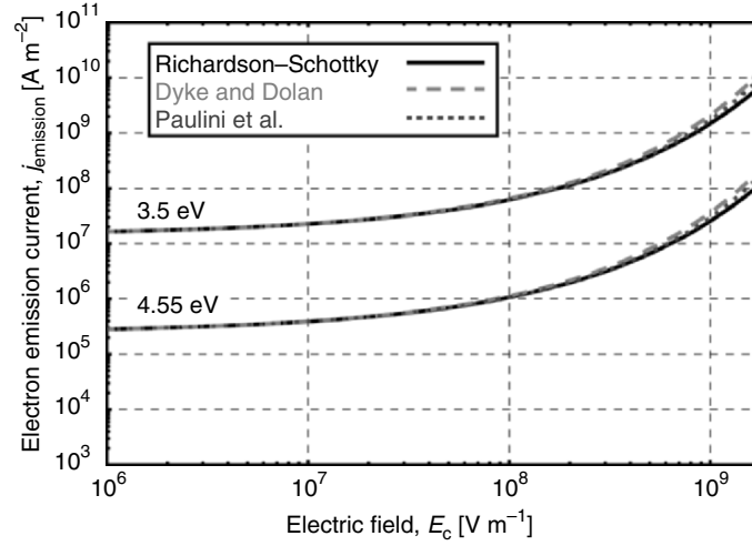
Fig. 2.33. Electron emission current j_{\text{emission}} for T = 3,000 K vs. electric field for two work functions \phi = 3.5 eV and 4.55 eV computed with three different models [59]
