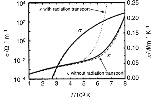
Fig. 4.41. Comparison of plasma properties: Electrical conductivity \sigma_{\text{LTE}} and thermal conductivity \kappa vs. plasma temperature for mercury, 0.6 MPa taken from [102] ( solid lines ) and calculated according to Sect. 2.3 and [171] ( dashed and dotted lines ). The thermal conductivity \lambda used for the numerical simulations is shown in Fig. 2.25
