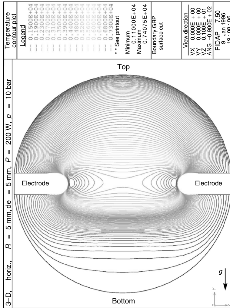
Fig. 4.12. Temperature profile (vertical longitudinal section) of a horizontally burning mercury HID lamp (Hg, 1 MPa, R_{\text{lamp}} = d_{\text{elec}} = 5 mm, r_{\text{elec}} = 0.5 mm, P_{\text{el}} = 200 W, [73])
