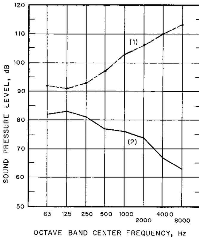
FIGURE 10-9 Sound pressure levels around the hoist: (1) before, L_A = 115 dBA, and (2) after installation of the muffer on the air exhaust of the hoist motor, L_A = 81 dBA.
